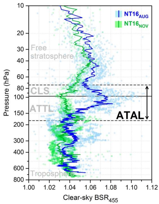
Figure 11. All clear-sky (i.e. aerosol-only) data points (dots) and mean profiles (solid lines) of BSR 455 as a function of pressure, for NT16 AUG (blue) and NT16 NOV (green). Black lines show the mean LRM (dashed), CPT (solid) and TOC (dashed) levels for NT16 AUG . The troposphere, ATTL, CLS and free stratosphere regions are identified by grey labels, and the ATAL region by a black arrow.
