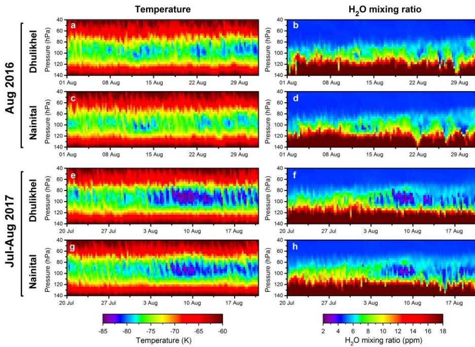
Figure 3. Time series of temperature (left column) and water vapor mixing ratio (right) as a function of pressure, from ECMWF operational analysis data (6-hourly, same horizontal and vertical resolution as given in caption of Figure 2 ) for the locations of NT (Panels c, d, g, h) and DK (a, b, e, f) during 1-31 August 2016 (a-d) and 20 July-21 August 2017 (e-h).
