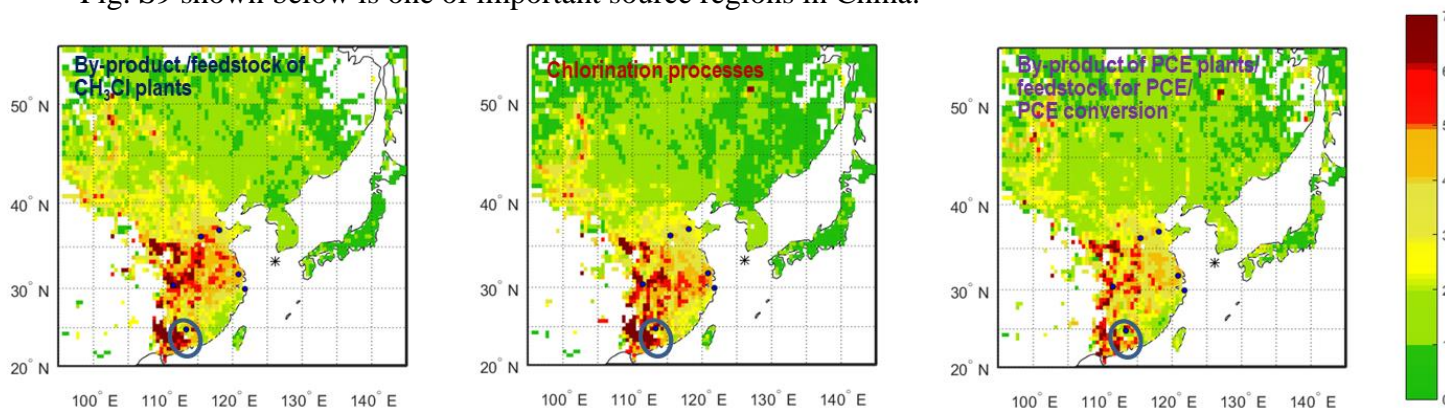
Fig. S9 shown below is one of important source regions in China.
