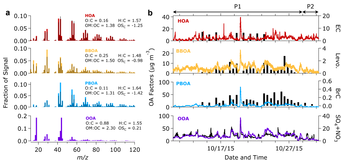
5 Figure 4: (a) Mass spectra of OA components resolved by the ME-2 analysis. Black bars represent the reference mass spectra of HOA and BBOA (Ng et al., 2011c) and peat burning aerosol (Budisulistiorini et al., 2017a) used as the constraints in the ME-2 analysis. The elemental ratios were estimated from signals at mass-to-charge ratio ( m/z ) 44 ( f_{44} ) and 43 ( f_{43} ) using the improved-ambient elemental analysis method (Canagaratna et al., 2015). (b) Time series of OA factors observed in Singapore during the 2015 haze episode. Time series of EC, levoglucosan, the sum of brown carbon (BrC) constituents, and the sum of SO 4 2- and NO 3 - in a unit of \mu\text{g m}^{-3} are shown against the time series of HOA, BBOA, PBOA, and OOA, respectively.
