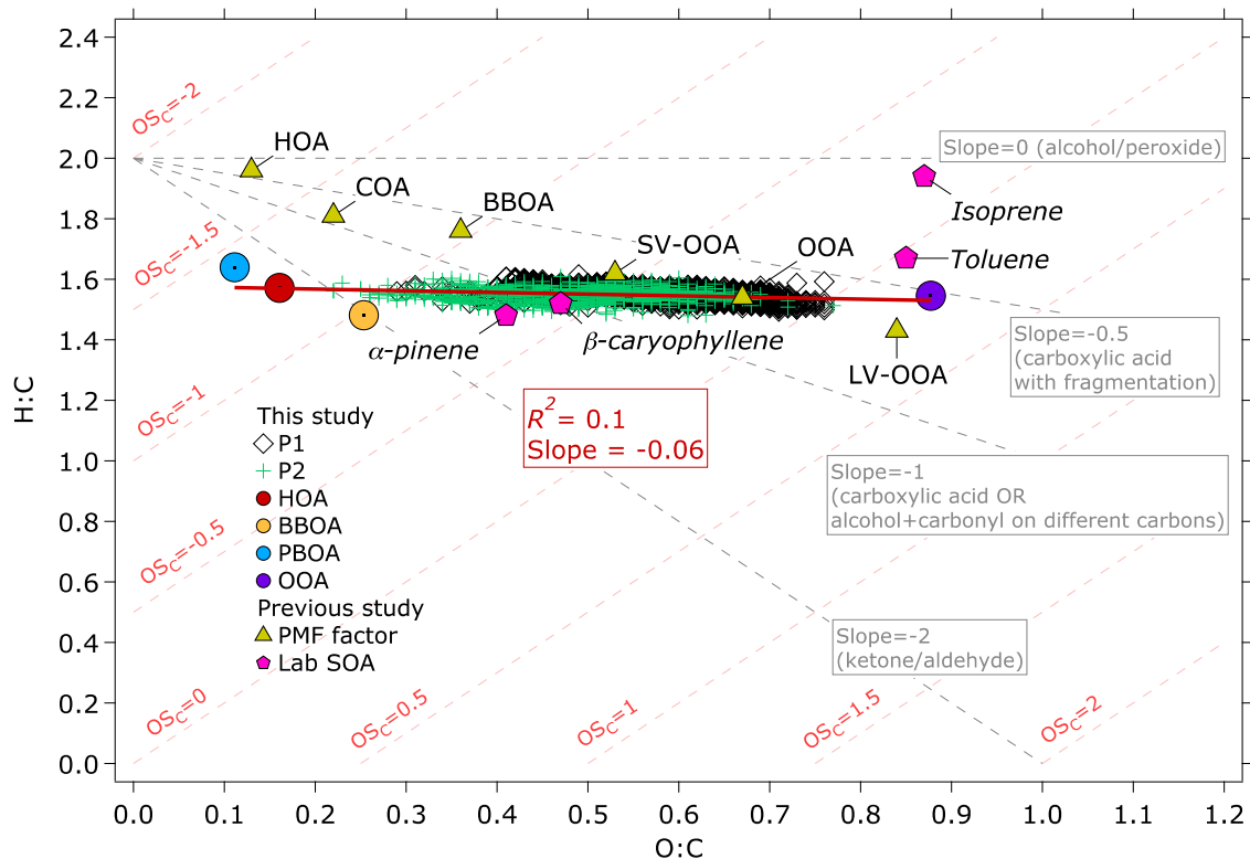
5 Figure 8: Van Krevelen diagram of the OA measured during the 2015 haze episode and the OA factors resolved by the ME-2 analysis. The H:C to O:C ratios are colored based on the P1 and P2 periods. The H:C to O:C ratios of the OA factors resolved by the ME-2 analysis of this study are plotted as colored circles. Linear regression analysis of H:C vs. O:C from the OA factors yielded R^2 = 0.1 and slope = -0.06 as plotted on the figure. Comparison with HOA, BBOA, cooking OA (COA), OOA, semi-volatile OOA (SV-OOA), and low-volatility OOA (LV-OOA) (triangle markers) and laboratory-generated SOA (hexagonal markers) of previous studies (Canagaratna et al., 2015 and references therein) show that the OOA factor of this study exhibits close characteristics to LV-OOA and toluene-derived SOA, indicating that its formation could be attributed to atmospheric processing.
