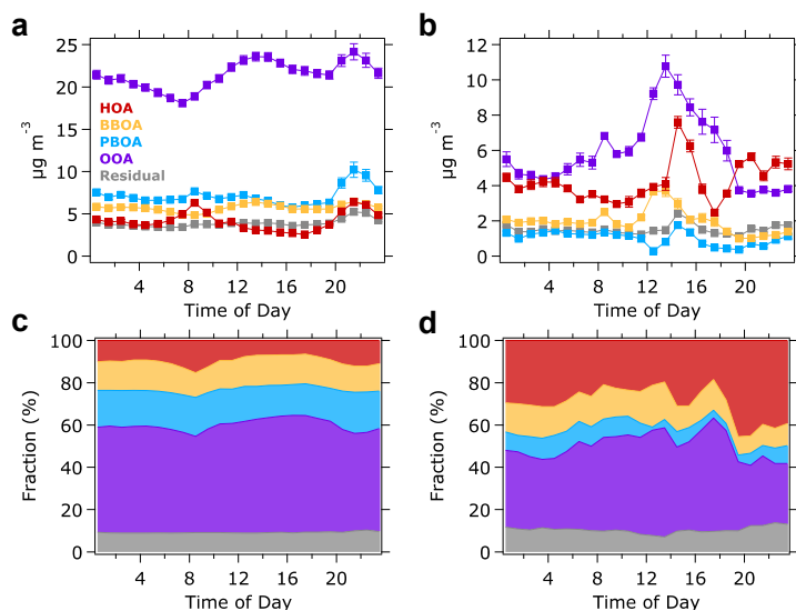
10 Figure 5: Average diurnal profiles of OA sources in a unit of \mu\text{g m}^{-3} (top panels) for (a) the P1 and (b) P2 periods. Bottom panels show similar diurnal profile but in fraction contribution to the total OA mass for (c) the P1 and (d) P2 periods.
