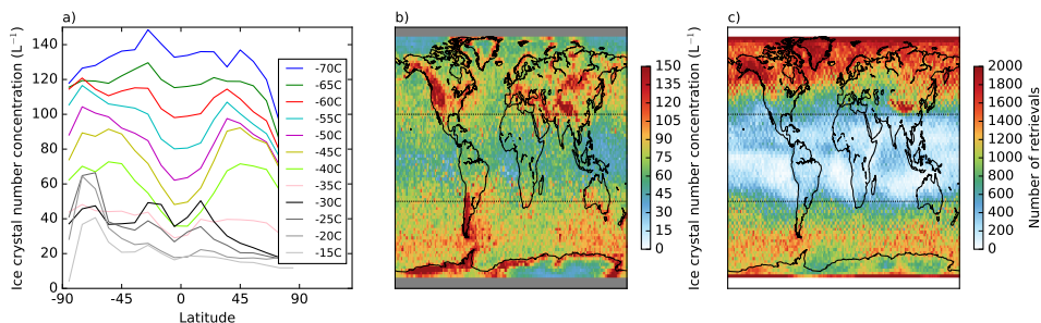
Figure 1. a) The zonal mean DARDAR-LIM cloud top N_i ( N_{i(top)}^{5\mu\text{m}} ) for crystals larger than 5\mu\text{m} as a function of temperature from DARDAR-LIM data for the period 2006-2013. Temperatures warmer than -35^{\circ}\text{C} are in greyscale. b) The mean N_{i(top)}^{5\mu\text{m}} at -50^{\circ}\text{C} . Grey indicates missing data. c) The number of cloud top retrievals at -50^{\circ}\text{C} . Zonal means and maps of N_i are available in part one.
