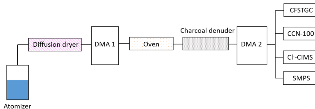
Figure 1. Experimental schematic.
