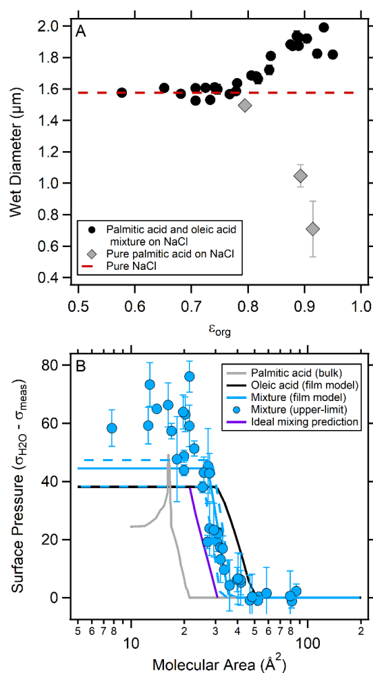
Figure 4. (A) Measured wet diameter at \text{RH} = 99.88\% as a function of organic volume fraction for 200 nm NaCl particles coated with pure palmitic acid (diamonds) and a mixture of palmitic acid and oleic acid (triangles). (B) Upper-limit and film model estimates for NaCl particles coated with a mixture of oleic acid and palmitic acid surface pressure as a function of molecular area. The black line is the oleic acid film model estimate and the grey line corresponds to bulk surface pressure measurements from Tang et al. 2010, since surface pressure measurements for NaCl particles coated pure palmitic acid were not possible (see text for details). The purple line is the ideal mixing estimate for surface pressure based on the measured molar fractions of oleic acid and palmitic acid.
