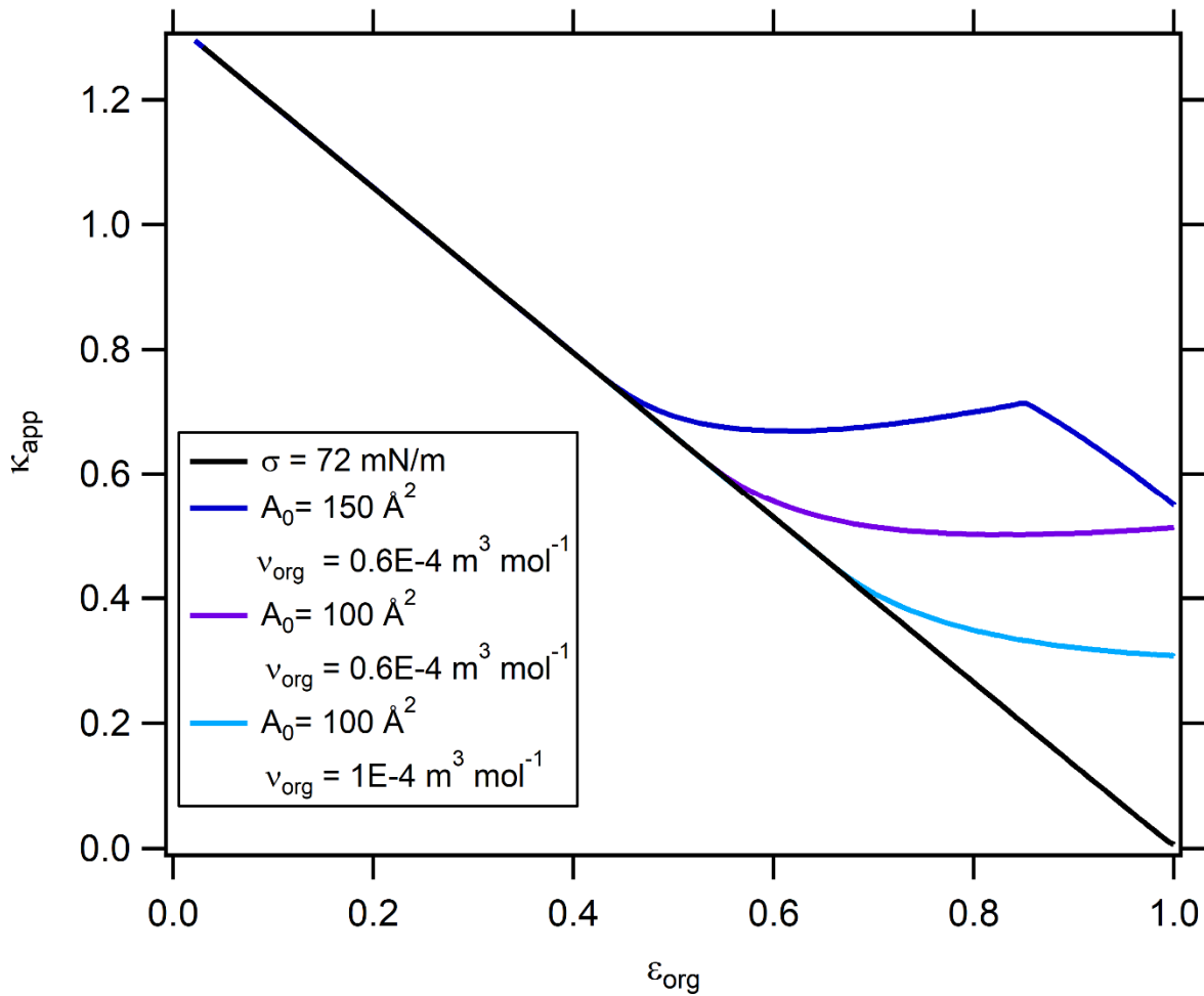
5 Figure 9. Apparent \kappa ( \kappa_{app} ) as a function of \epsilon_{org} for mixed NaCl-organic particles having a constant total diameter (136.8 nm), calculated using the film model. The black line is the constant \sigma case, the dark blue line was calculated using A_0 = 150 \text{ \AA}^2 and v_{org} = 0.6 \times 10^{-4} , the purple line is calculated using A_0 = 100 \text{ \AA}^2 and v_{org} = 0.6 \times 10^{-4} , and the light blue line is calculated using A_0 = 100 \text{ \AA}^2 and v_{org} = 1 \times 10^{-4} .
