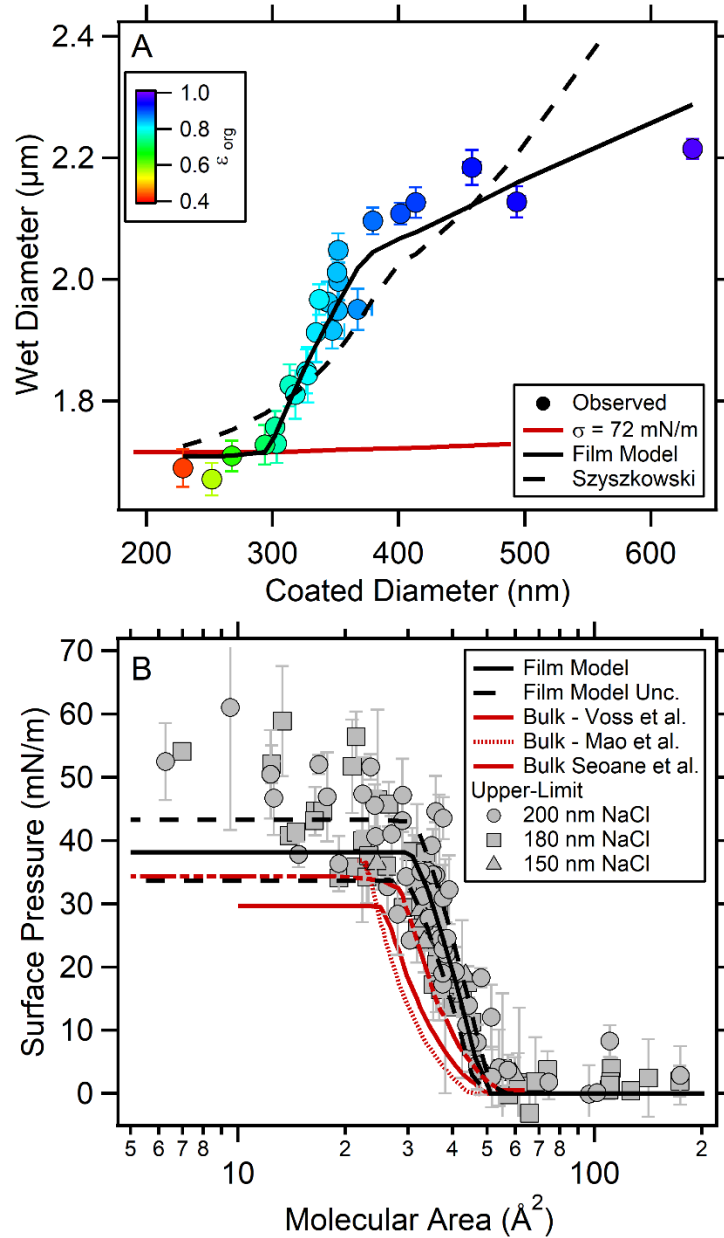
Figure 2. (A) Wet diameter (at RH = 99.93%) vs. dry diameter of 200 nm NaCl particles coated with varying amounts of oleic acid. The red line is the calculated droplet size, assuming \sigma = 72 mN/m independent of coating amount and the black and dashed black lines are film model and Szyszkowski model fits to the data, respectively. The error bars correspond to the 95% confidence interval for mode of the wet diameter distribution. The data points are colored by organic volume fraction ( \epsilon_{\text{org}} ). (B) Upper-limit estimates (grey points) and film model estimates (black lines) for surface pressure as a function of molecular area for various NaCl seed sizes (circles = 200 nm, squares = 180 nm, and triangles = 150 nm) and RH. Error bars on individual points and the film model fit (dashed black lines) are based on the precision in RH. Bulk measurements (red lines) adapted from Voss et al. 2007, Mao et al. 2013, and Seoane et al. 2000 are included for reference.
