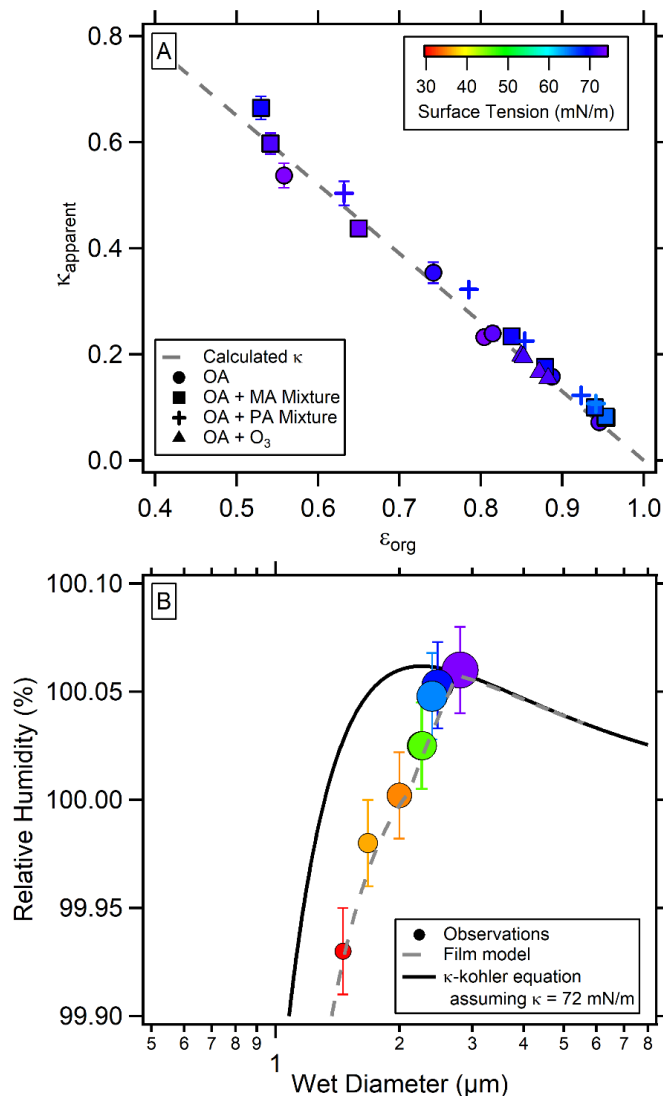
Figure 5. (A) Apparent \kappa values as a function of \epsilon_{\text{org}} as calculated from the critical supersaturation for NaCl particles coated with oleic acid (circles), a mixture of myristic acid and oleic acid (squares), a mixture of palmitic acid and oleic acid (crosses) and oxidized oleic acid (triangles). Also shown is the predicted \kappa based on volume mixing rules assuming that \kappa_{\text{NaCl}} = 1.3 and \kappa_{\text{org}} = 0.001 , with \sigma = 72 \text{ mN/m} . Each point is colored by the actual surface tension required to match observations in \kappa . (B) Relative humidity as a function of measured wet diameter for 150 nm (mobility diameter) NaCl particles coated with a fixed amount of oleic acid ( \epsilon_{\text{org}} = 0.95 ). Points are colored by upper-limit estimates for surface tension and the size of the points corresponds to the wet diameter. Also shown are values predicted from the compressed film model and \kappa -Köhler theory assuming \sigma = 72 \text{ mN/m} .
