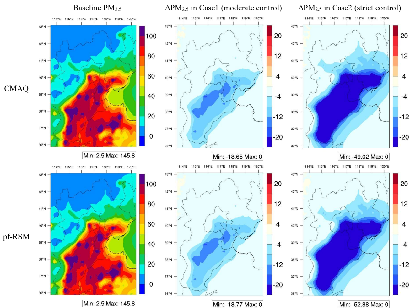
Figure 7. Spatial distribution of CMAQ-simulated and pf-RSM-predicted PM 2.5 in baseline and PM 2.5 responses in two control scenarios (monthly averages in January 2014, unit: μg m -3 , the E NO x , E SO 2 , E NH 3 , E VOCs and E POA in case1 and case2 are -49%, -45%, -20%, -64%, -20% and -76%, -79%, -81%, -83%, -73% respectively)
