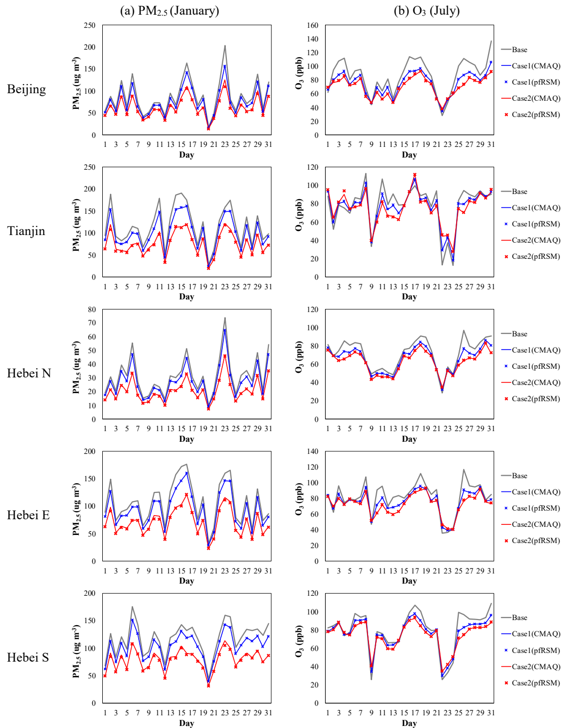
Figure 9. Daily series of CMAQ-simulated and pf-RSM-predicted daily averaged PM 2.5 in January and daily 1-hour maxima O 3 in July 2014 in baseline and two control scenarios (the E NOx , E SO2 , E NH3 , E VOCs and E POA in case1 and case2 are -49%, -45%, -20%, -64%, -20% and -76%, -79%, -81%, -83%, -73% respectively)
