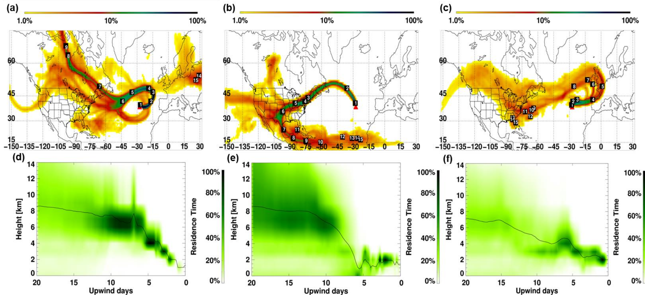
Figure 1. FLEXPART retroplumes for 27-28 June 2013 (PMO-1, (a, d)), 5-6 July 2014 (PMO-2, (b, e)), and 20-21 June 2015 (PMO-3, (c, f)): column integrated residence time over the 20-day transport time (a-c) and vertical distribution of the retroplume residence time at given upwind times (d-f). The white labels indicate the approximate locations of the center of the plume for each of the transport days. Residence time is color coded by logarithmic grades representing its ratio to the location of maximal integrated residence time (100%). The black line indicates the mean height of the plume during transport.
