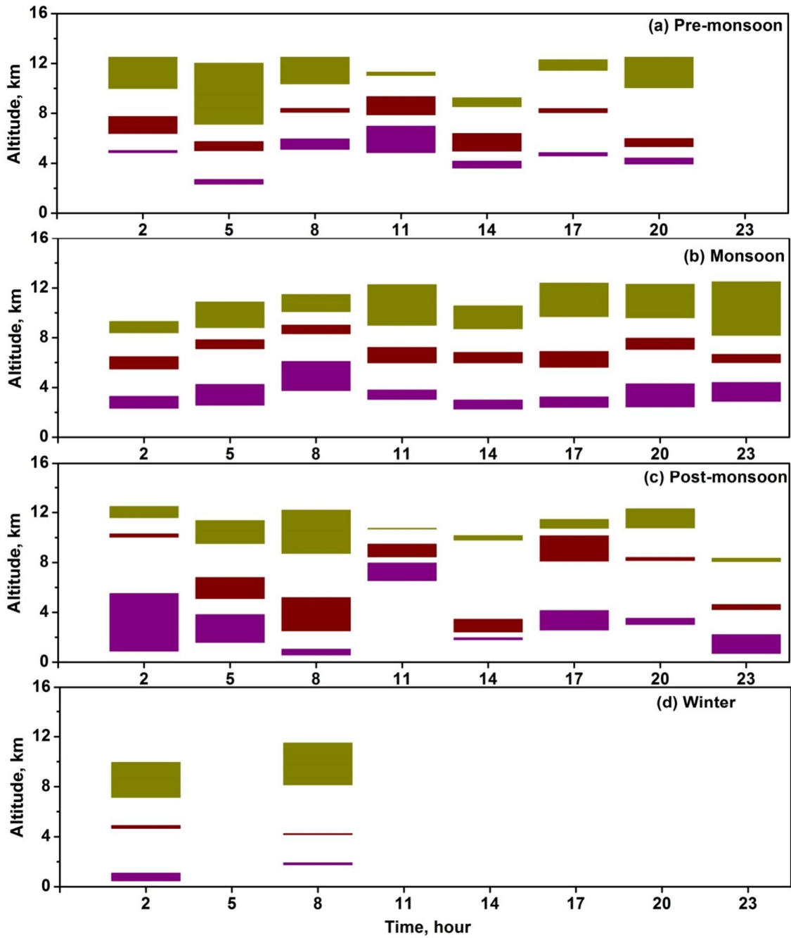
Figure S1. Diurnal variations of mean vertical locations (base and top), thicknesses of three-layer clouds observed during (a) pre-monsoon, (b) monsoon, (c) post-monsoon, and (d) winter seasons.
