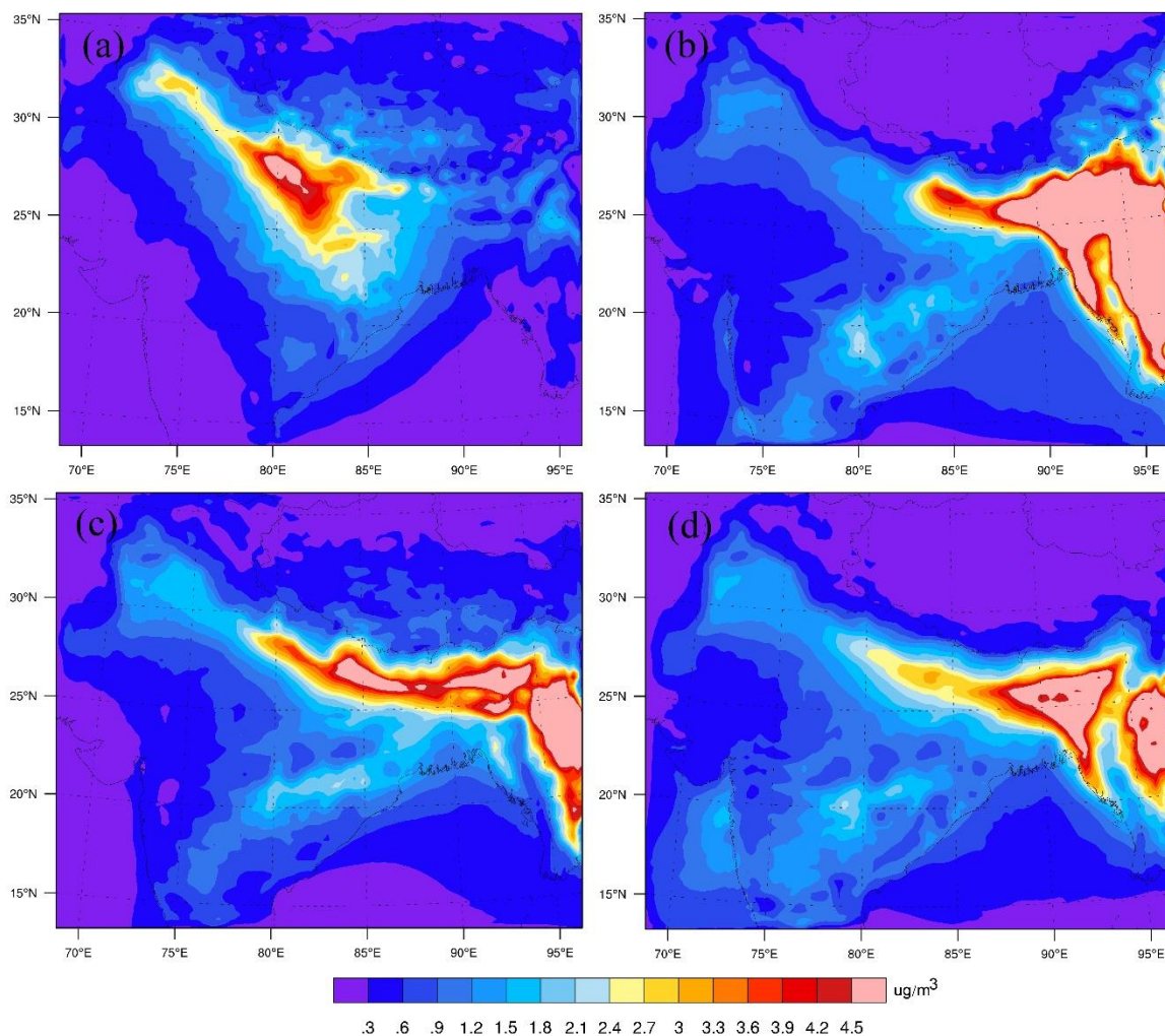
Figure 8. Mean BC concentration simulated by WRF-Chem model at QOMS and its vicinities: (a) event A; (b) event B; (c) event C; (d) event D.
