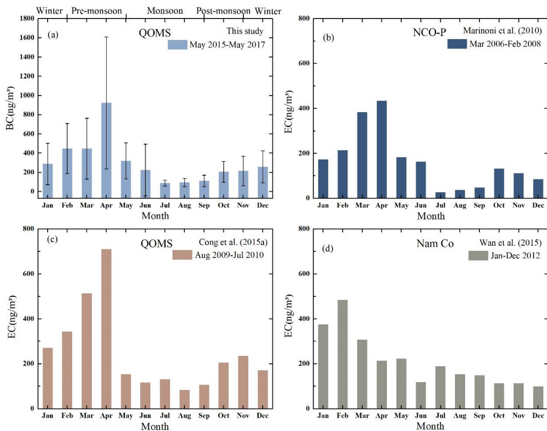
Figure 2. (a) Monthly mean BC concentrations at QOMS from May 2015 to May 2017 in this study; (b) Monthly mean EC at NCO-P from March 2006 to February 2008 from Marinoni et al. (2010); (c) Monthly mean EC at QOMS from August 2009 to July 2010 from Cong et al. (2015a); (d) Monthly mean EC at Nam Co station from January to December during 2012 from Wan et al. (2015).
