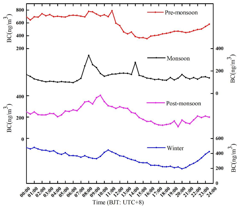
Figure 4. Diurnal variation in BC concentrations (every half an hour) at QOMS during study period.
