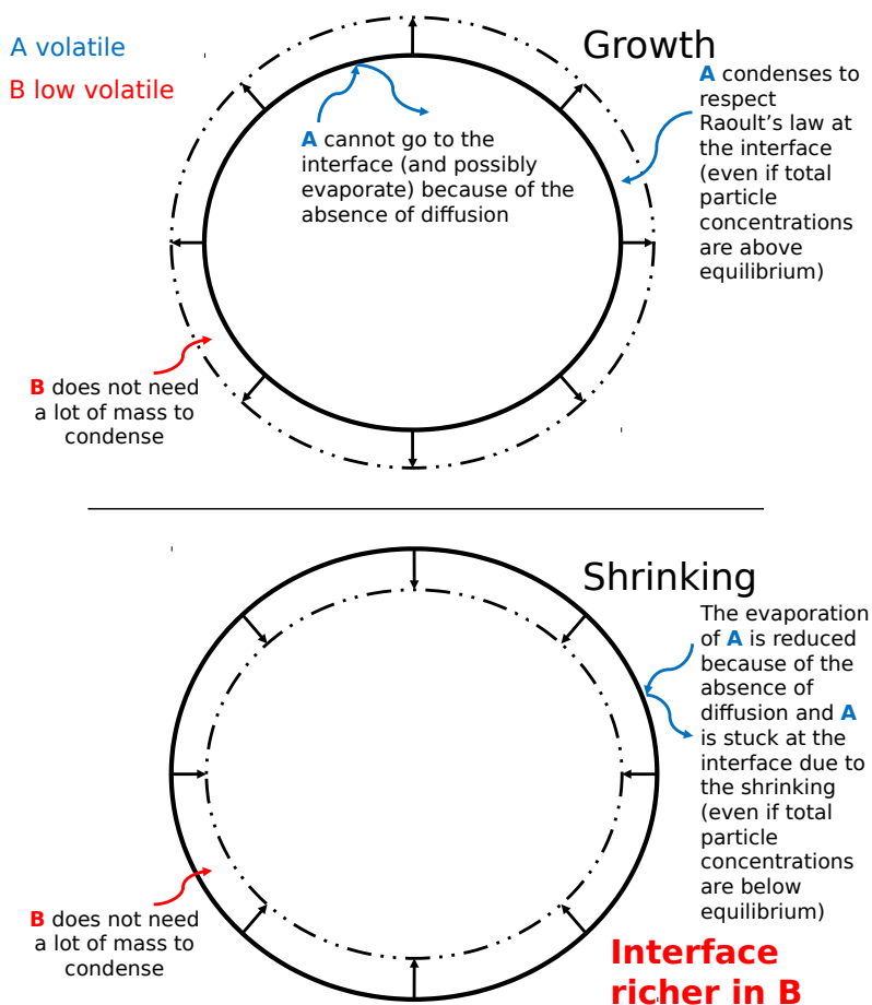
Figure 5. Schematic representation of SOA formation for a growing (top) and shrinking (down) highly viscous aerosol. The blue curved arrows describe the behavior of an organic compound A and the red curved arrows describe the behavior of a low-volatility organic compound B .
