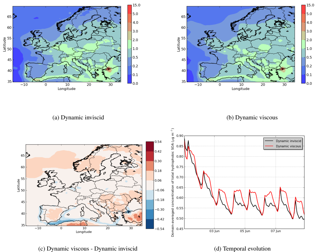
Figure 9. Modeled hydrophobic SOA concentrations in (a) the Dynamic inviscid simulation, (b) the Dynamic viscous simulation, (c) the differences between the simulations ( \mu\text{g m}^{-3} ) and (d) the temporal evolutions.
