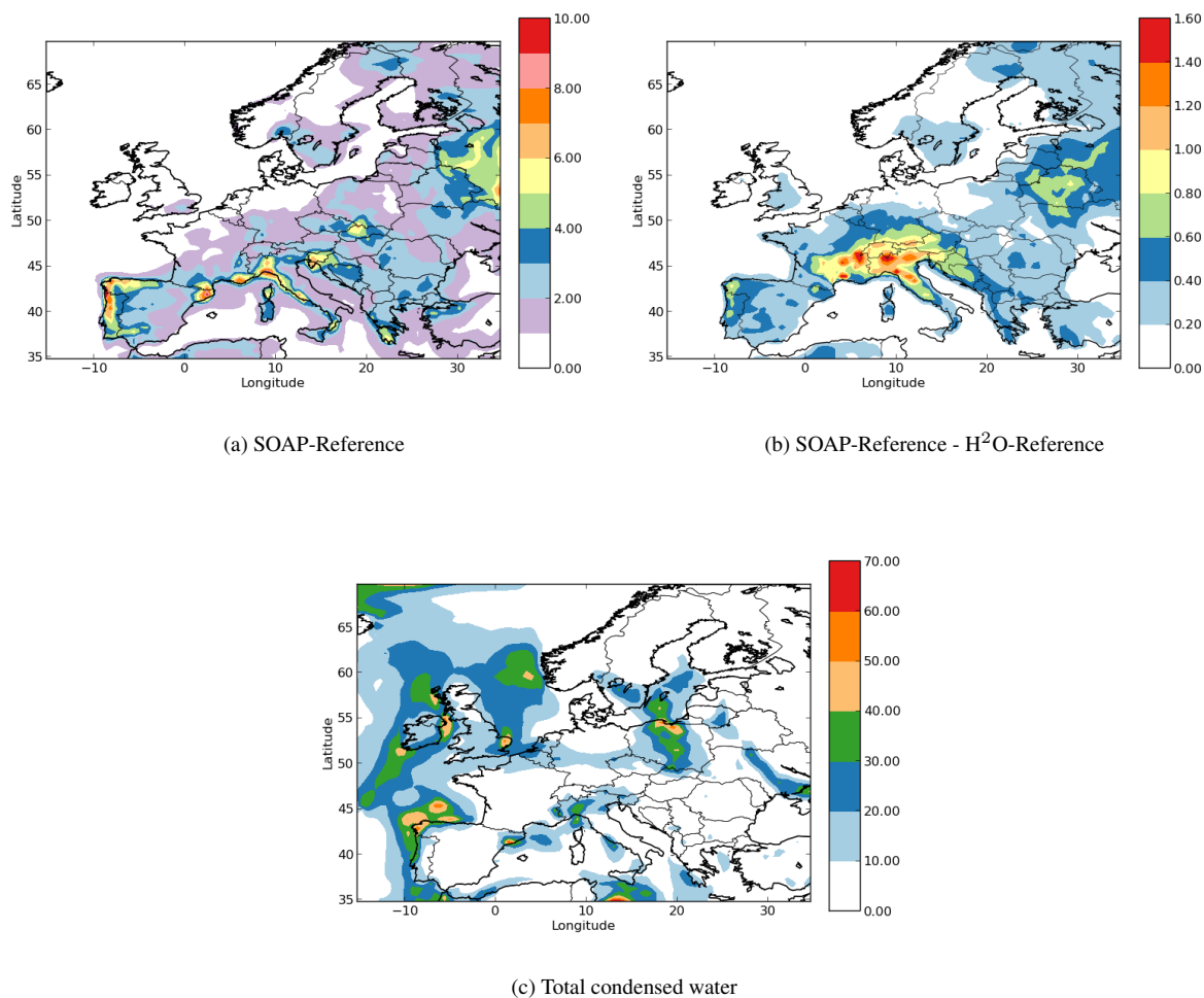
Figure 4. (a) SOA concentrations in the SOAP-Reference simulation ( \mu\text{g m}^{-3} ), (b) the differences of the SOA concentrations between the SOAP-Reference and H 2 O-Reference simulations ( \mu\text{g m}^{-3} ) and (c) concentration of total condensed water in the SOAP-Reference simulation ( \mu\text{g m}^{-3} ).
