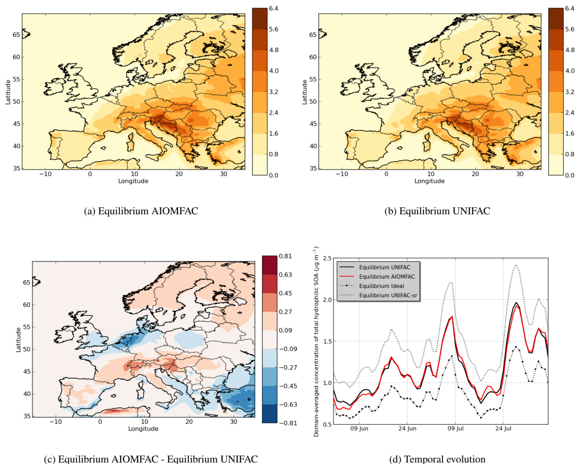
Figure 7. Modeled hydrophilic SOA concentrations in (a) the Equilibrium AIOMFAC simulation, (b) the Equilibrium UNIFAC simulation, (c) the differences between the simulations ( \mu\text{g m}^{-3} ) and (d) the temporal evolutions of domain averaged concentrations.
