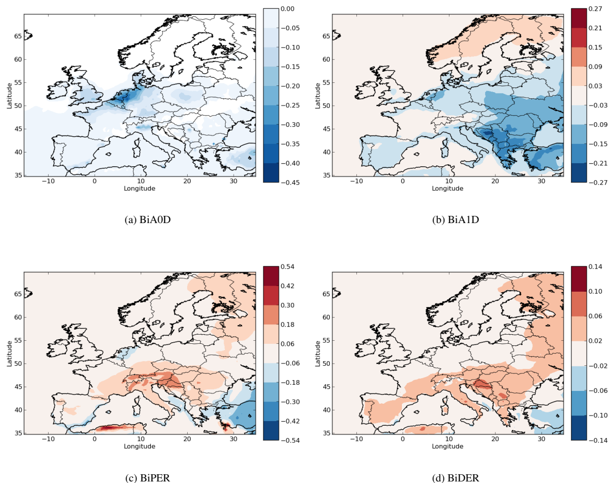
Figure 8. Differences in concentrations of several SOA compounds between AIOMFAC and UNIFAC over Europe (AIOMFAC - UNIFAC in \mu\text{g m}^{-3} ). The definition of the compounds is given in Table 1.
