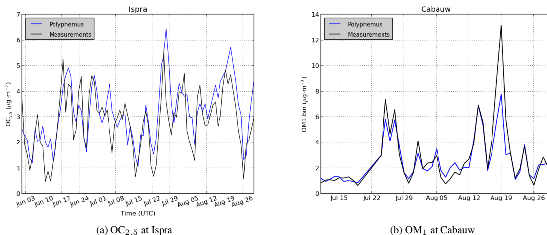
Figure 6. Comparison of modeled SOA concentrations (blue) with observations (black) for (a) OC_{2.5} concentrations at Ispra, (b) OM_1 concentrations at Cabauw.
