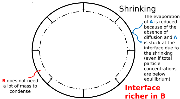
Fig. 2. Schematic representation of SOA formation for a growing (top) and shrinking (down) highly viscous aerosol (Blue arrows: an organic compound A and red arrow: a low-volatility organic compound B).
