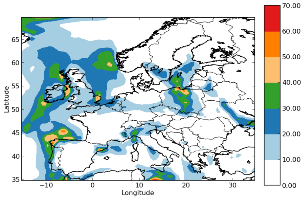
Fig. 1. Concentration of total condensed water in the SOAP-Reference simulation ( \mu\text{g m}^{-3} ).
