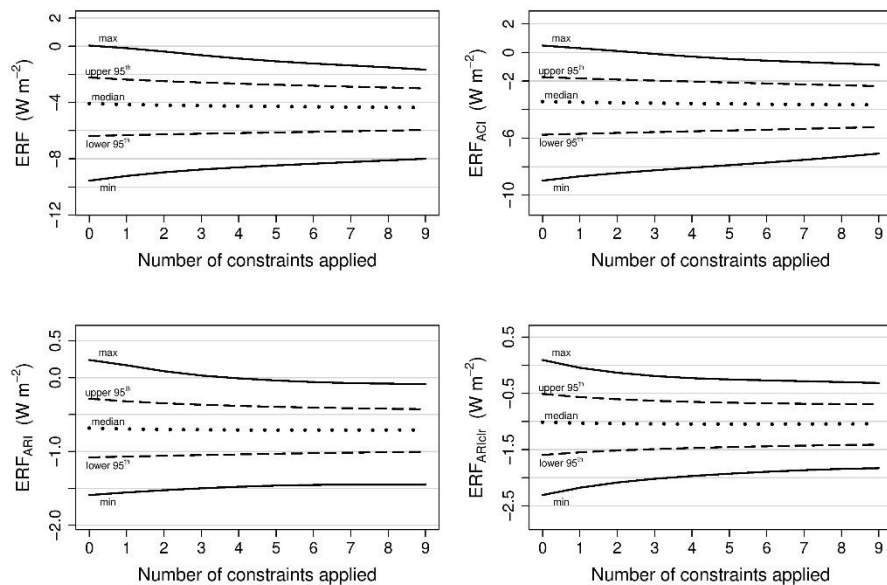
Figure 8. The dependence of aerosol ERF uncertainty on the number of observational constraints applied. The lines show the mean effect of different numbers of constraints.
