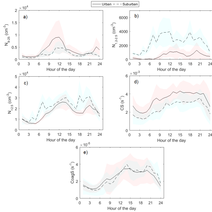
Figure A1: Averaged daily cycles of (a) total particle concentration in the size range 9-25 nm, (b) total particle concentration in the size range 1.2-2.5 nm measured with PSM at CSIC and ISCIII, (c) total concentration of particles >2.5 nm measured with PSM at CSIC and ISCIII, (d) condensation sink (CS), and (e) coagulation sink (CoagS) during regional new particle formation events at urban (CSIC and CIEMAT, solid line) and suburban (ISCIII, dashed line) stations. Red (urban) and blue (suburban) shaded shapes show 95% confidence intervals. The hour of the day is given in UTC. Local time is UTC+2 hours.
