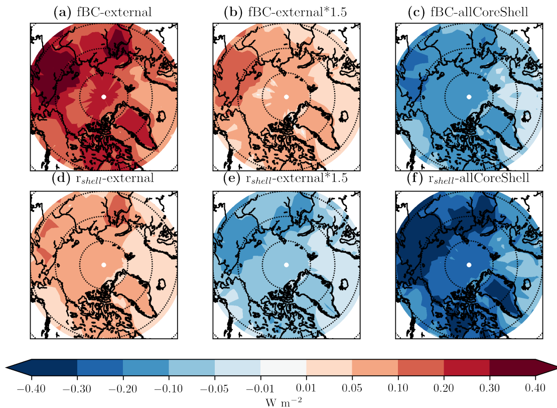
Figure 8. The difference in DRE between fBC-constrained (a,b,c) and r shell -constrained (d,e,f) compared to the bounding mixing-state assumptions.
