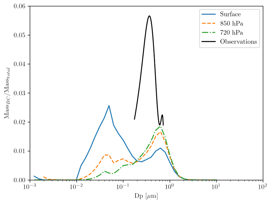
Figure 5. The fraction of BC aerosol mass relative total aerosol mass at each size bin in GEOS-Chem-TOMAS at three vertical levels along with the fraction determined from the SP2 and UHSAS observations.
