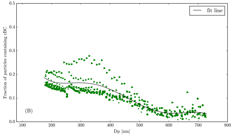
Figure 4. Number distributions for the bare rBC cores (black), the coated rBC-containing particles (green), and the total aerosol as detected by the UHSAS (grey) for the median coating thickness scenario. Shown in the bottom panel is the distribution of the fraction of the total aerosol containing rBC in the median coating scenario. The solid black line is a polynomial fit to the observations following the form (with x in nm): y = 1.25 - (1.52 \times 10^{-2})x + (8.05 \times 10^{-5})x^2 - (2.00 \times 10^{-7})x^3 + (2.31 \times 10^{-10})x^4 - (1.00 \times 10^{-13})x^5 .
