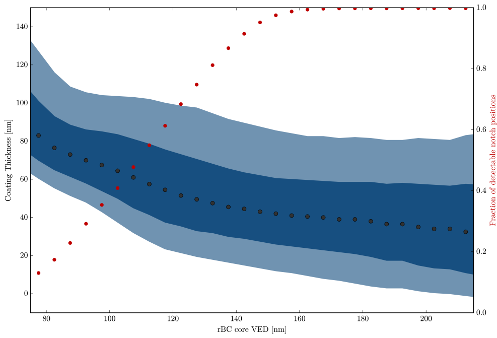
Figure 3. Coating thickness as a function of rBC core diameter. Grey markers are the median, dark shaded area is the 25th-75 percentile, lighter shaded area is the 10-90th percentile of coating thicknesses for each bin.
