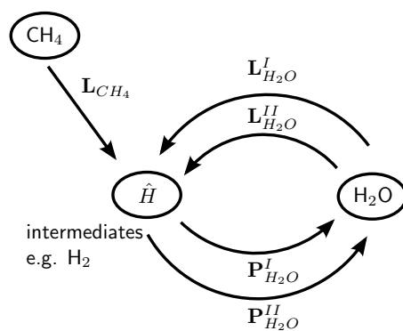
Figure 1. Sketch on the production and recycling of \text{H}_2\text{O} . The arrows of L_{\text{CH}_4} and P_{\text{H}_2\text{O}}^I are indicating the direct yield and all arrows together the effective yield.
