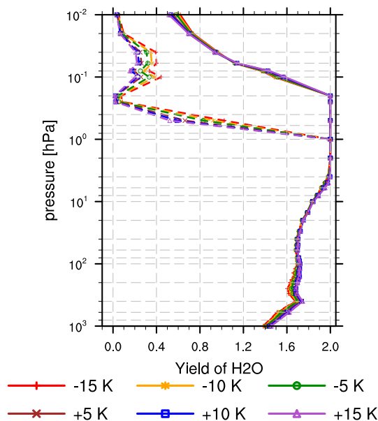
Figure 9. The pseudo vertical profile of the \text{H}_2\text{O} yield calculated by the box model approach. Solid lines represent the direct yield, the dashed lines the effective yield and circles indicate the pressure levels of the model boxes. OH is kept constant to the initial values of the respective vertical box. The plot shows sensitivities concerning temperature. Temperature is varied from the standard atmosphere value by -15K (red), -10K (orange), -5K (green), +5K (brown), +10K (blue) and +15 K (purple).
