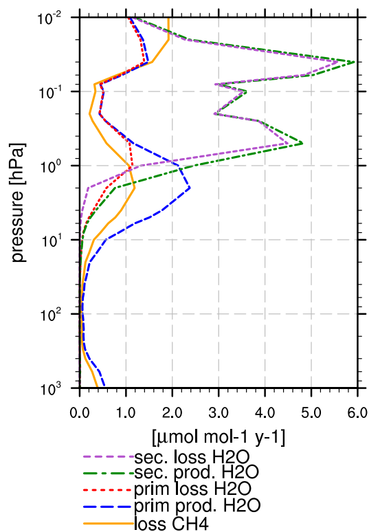
Figure 2. Separate loss of \text{CH}_4 and primary and secondary loss and production of \text{H}_2\text{O} from box model simulation Ref.
