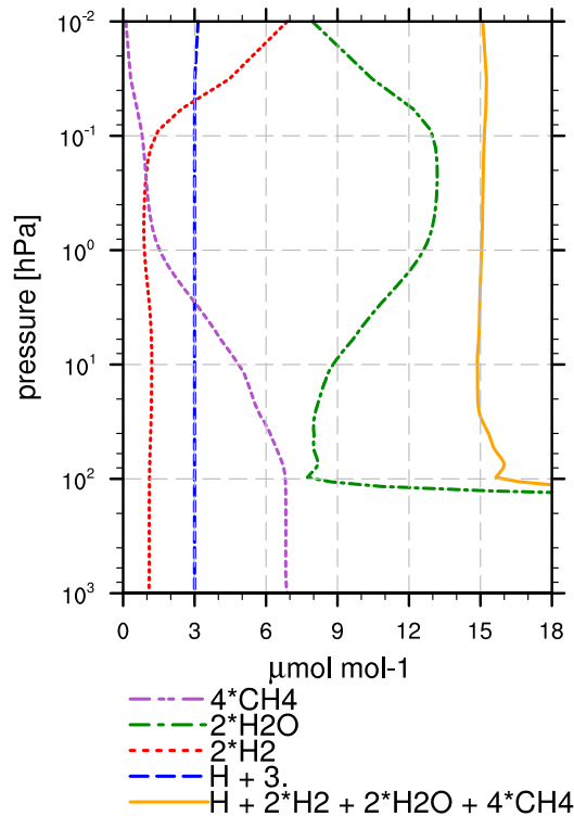
Figure 12. Annual zonal average of H content by species (in \mu\text{mol mol}^{-1} ) over the tropics ( 23^\circ \text{ S} - 23^\circ \text{ N} ). H is shifted by 3.0 \mu\text{mol mol}^{-1} for a better visibility.
