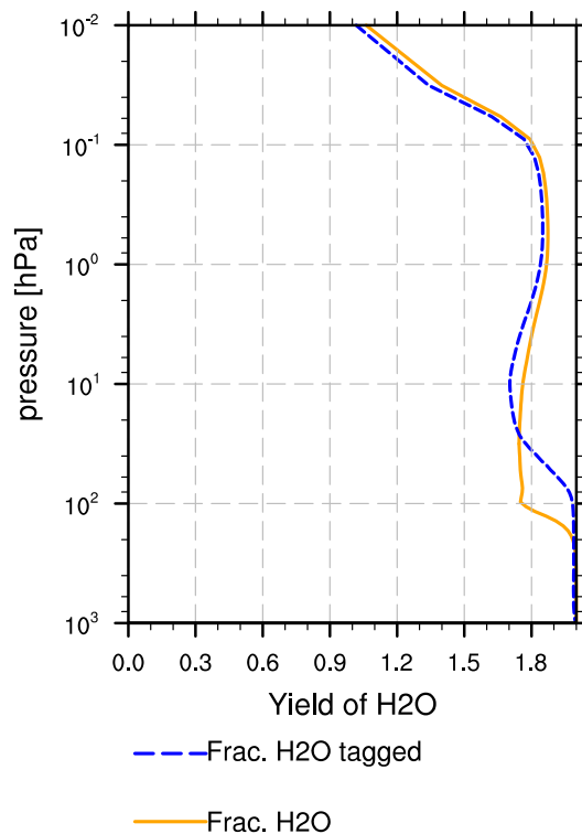
Figure 13. H portion of tagged and total H 2 O with respect to the tagged and total hydrogen content ( H+2\times H_2+2\times H_2O ), respectively.
