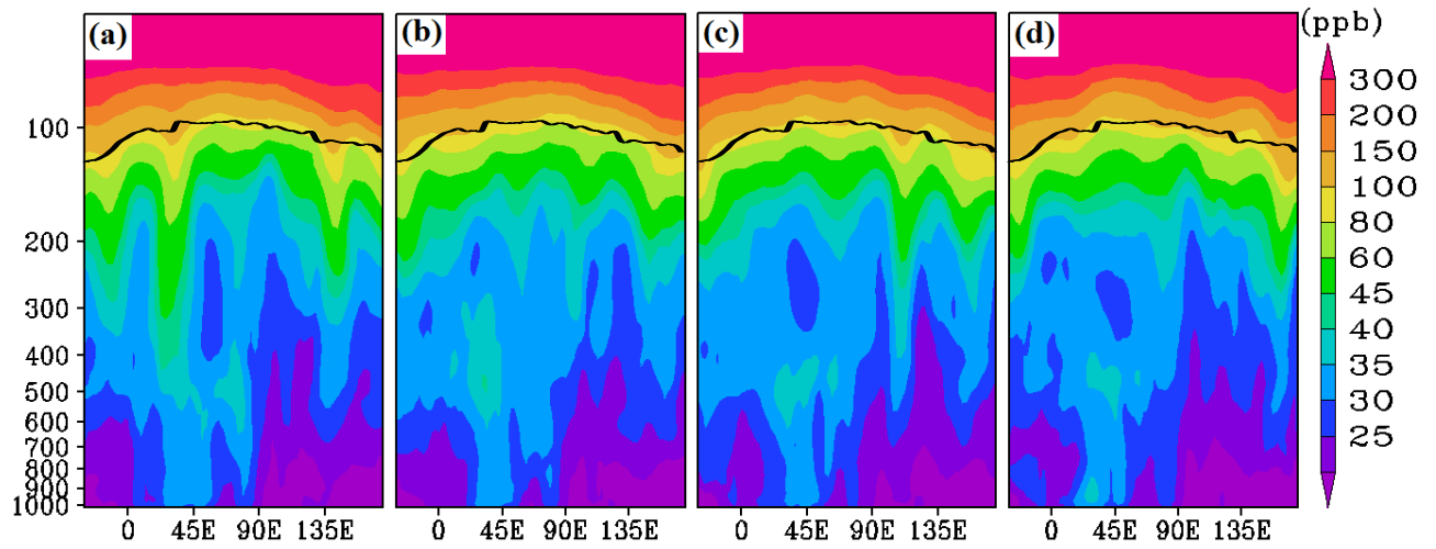
21 Figure S2: Longitude-pressure section (averaged for 20-40° N) of ozone (ppb) from 22 ECHAM5-HAMMOZ CTRL simulation for (a) 02 July, (b) 04 July, (c) 06 July, (d) 08 July, 23 2003. Black line indicates tropopause.
