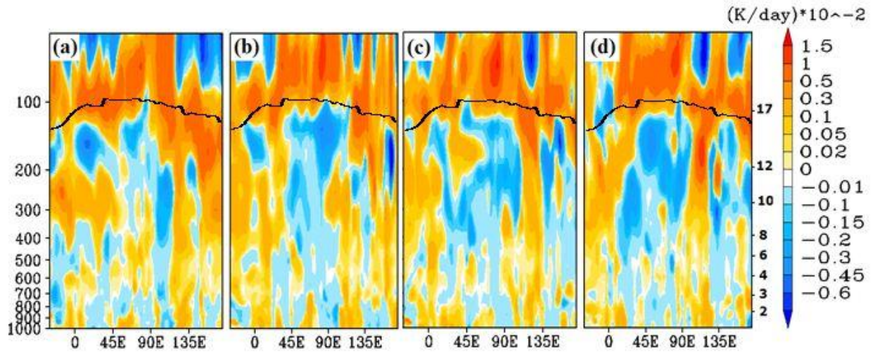
Figure 9: Longitude-pressure distribution (averaged for 18°-20° N) of anomalies of ozone heating rates ((K \cdot day^{-1}) \times 10^{-2}) for (a) 02 July, (b) 04 July, (c) 06 July, (d) 08 July, 2003. Pressure (hPa) is indicated on left y-axis and altitudes (km) on right y-axis. The black thick line indicates the tropopause.
