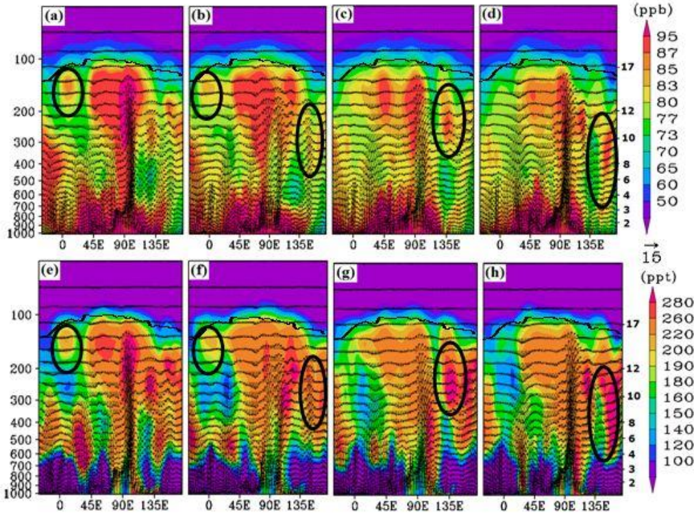
Figure 7: Longitude-pressure section (averaged for 20°-40° N) of CO (ppb) from ECHAM5-HAMMOZ CTRL simulation for (a) 02 July, (b) 04 July, (c) 06 July, (d) 08 July, 2003. (e)-(h) same as (a)-(d) but for PAN (ppt). Black thick line indicates the tropopause and black dotted circles indicate maximum in CO and PAN amounts near eddies. Pressure (hPa) is indicated on left y-axis and altitudes (km) on the right y-axis. Wind vectors ( \text{m}\cdot\text{s}^{-1} ) are shown by black arrows. Vertical velocity field is scaled by a factor of 300.
