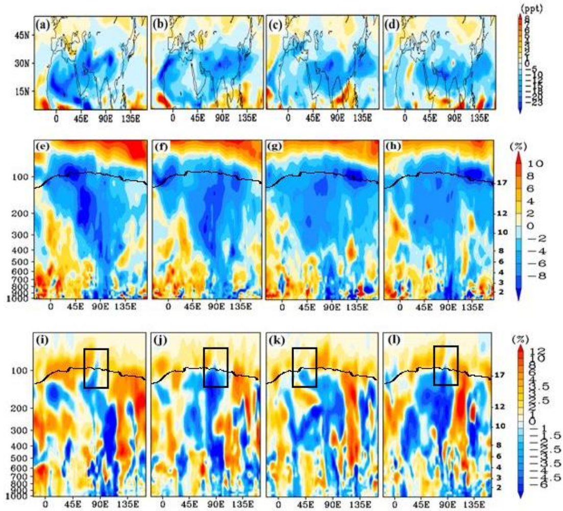
Figure 8: Spatial distribution of anomalies (Asia10-CTRL) of PAN mixing ratios (ppt) (color shades) at 16 km from ECHAM5-HAMMOZ model simulations for (a) 02 July, (b) 04 July, (c) 06 July, (d) 08 July, 2003. Longitude-pressure distribution (averaged for 20°-40° N) of anomalies of PAN (%) for (e) 02 July, (f) 04 July, (g) 06 July, (h) 08 July, 2003. (i)-(l) same as (e)-(h) but for ozone anomalies (%) (averaged for 18°-20° N). Black thick line indicates the tropopause. Pressure (hPa) is indicated on left y-axis and altitudes (km) on right y-axis. Black boxes in the bottom panels indicate regions of cross tropopause transport.
