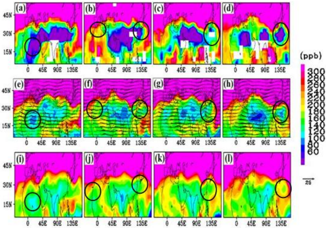
Figure 4: Spatial distribution of ozone mixing ratios (ppb) (color shades) corresponding to MIPAS satellite observations at 16 km for (a) 1-2 July, (b) 3-4 July, (c) 5-6 July, (d) 7-8 July, 2003; ERA-Interim reanalysis at 100 hPa for (e) 2 July, (f) 4 July, (g) 6 July, (h) 8 July, 2003, and ECHAM5-HAMMOZ CTRL simulations at 16 km for (i) 2 July, (j) 4 July, (k) 6 July, (l) 8 July, 2003. Black arrows in panels (e)-(h) show wind anomalies ( \text{m s}^{-1} ) at 200 hPa. Minimum ozone amounts near the location of eddies are shown with black circles.
