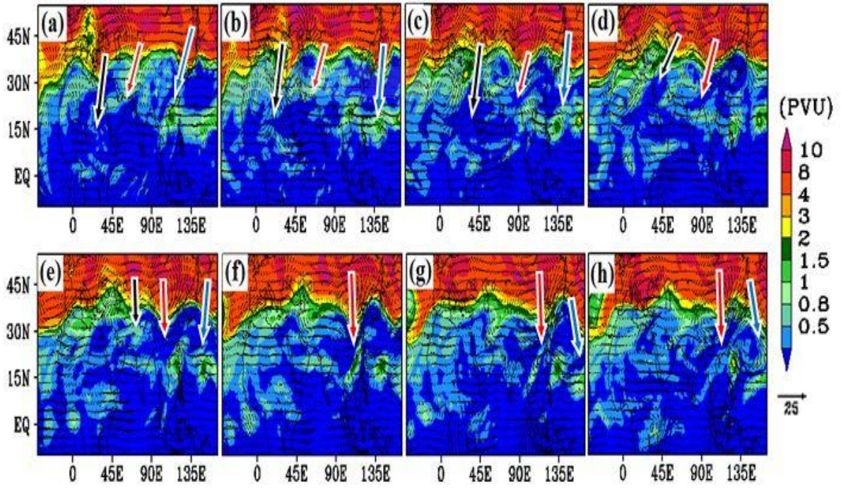
Figure 2: Spatial distribution of potential vorticity (PVU) (color shades) at 350 K potential temperature surface and wind anomalies in \text{m s}^{-1} (thin black vectors) at 200 hPa from ERA-Interim reanalysis for (a) 01 July, (b) 02 July, (c) 03 July, (d) 04 July, (e) 05 July, (f) 06 July, (g) 07 July, (h) 08 July, 2003. The events of RBW-1, RBW-2 and RBW-3 are indicated by solid black, red and blue arrows, respectively.
