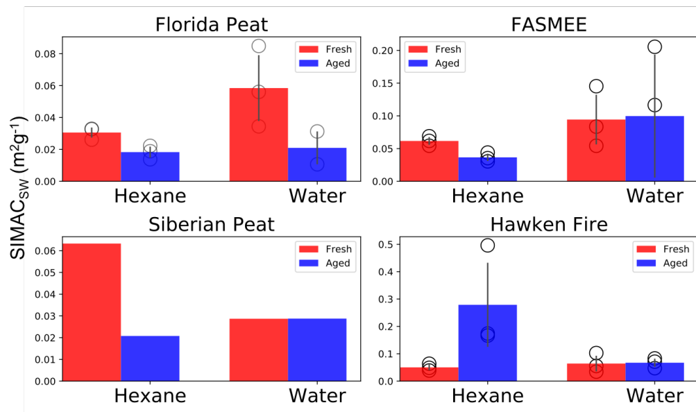
Figure 8. Comparison of the total solar-weighted spectrally integrated mass absorption coefficient (SIMAC sw ) for the fresh and aged aerosols in water and hexane extracts, normalized to 1-ml extraction volumes. Bars, circles, and error bars represent the mean values, individual observations, and standard deviations, respectively. No error bars are given for Siberian peat, because only one experiment was performed with this fuel.
