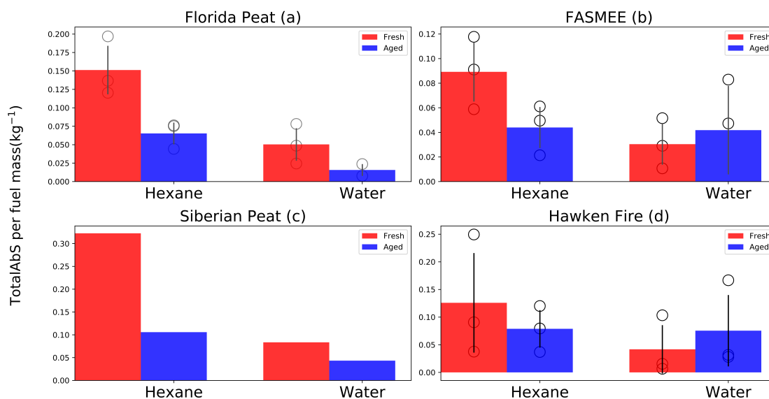
Figure 3. Comparison of total absorbance (eq. 3) per fuel mass consumed for fresh and aged aerosols in 15 water and hexane extracts, normalized to 1-mL extraction volumes. Bars, circles, and error bars
