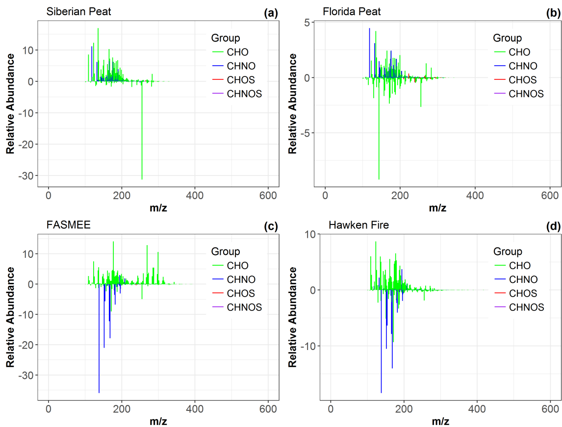
Figure 5. Ultrahigh resolution mass spectrometry difference mass spectra for the emissions from the combustion of the representative fuels (smoldering (peat) fuels (on top, (a) & (b)) and flaming fuels (on bottom, (c) & (d))
