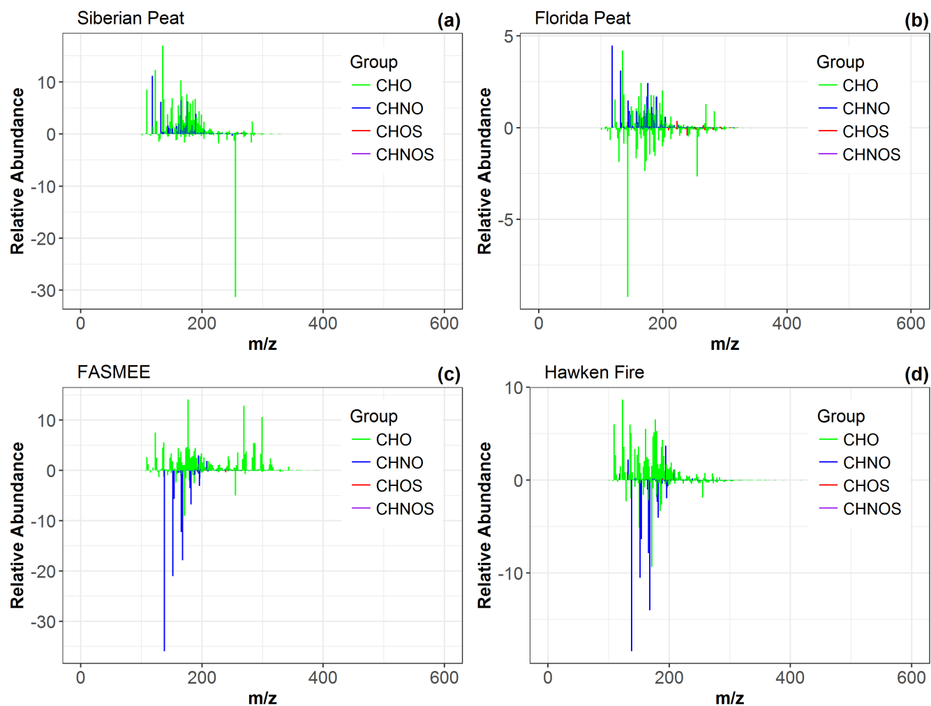
Figure 5. Ultrahigh resolution mass spectrometry difference mass spectra for WSOC from the combustion emissions from the combustion of the representative fuels (smoldering (peat) fuels (on top, 5 (a) & (b)) and flaming fuels (on bottom, (c) & (d))
