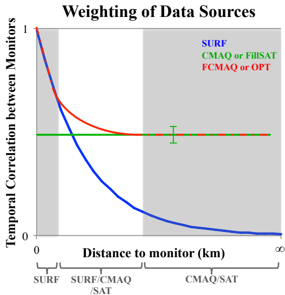
5 Figure 5: Theoretical plot of fused and optimized dataset weights as a function of distance from surface observations. Three regimes identify the contribution of each dataset towards improving concentration field estimates stratified by distance. As applied here, the exponential decay rate that reflects the temporal Pearson correlation between ground observations as a function of distance is species-specific. The temporal variations between ground observations and CMAQ or FillSAT are more consistent (shown as constant), independent of ground observations, and therefore, are not functions of distance to monitor. FCMAQ (surface measurements + model) and OPT (surface + satellite measurements + model) curves show how the strengths of the ground observations and other datasets are maximized using temporal correlations as each grid cell is a function of distance from a ground observation.
