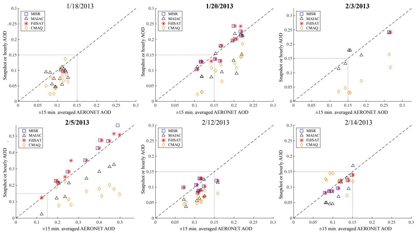
Figure 3: Scatterplot comparisons of AERONET coincidences with MISR-RA, MAIAC, gap-filled MISR-RA, and CMAQ results within \pm 15 minutes of Terra overpass time. The MAIAC and AERONET AOD comparisons are plotted at 550 nm, whereas the MISR-RA and AERONET AOD comparisons are at 558 nm; the dotted lines indicate the 0.15 AOD threshold; a 1:1 dashed lines are shown for reference.
