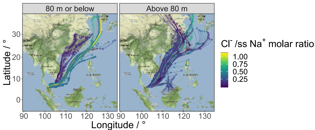
Figure 10: 7-day HYSPLIT back trajectories centred on the Bachok research station, between 18-01-2014 and 07-02-2014. The back trajectories are coloured by the Cl^-/ssNa^+ molar ratio. Trajectories with a mean height of 80 m or below are shown in the left panel and trajectories with a mean height greater than 80 m are shown in the right panel.
