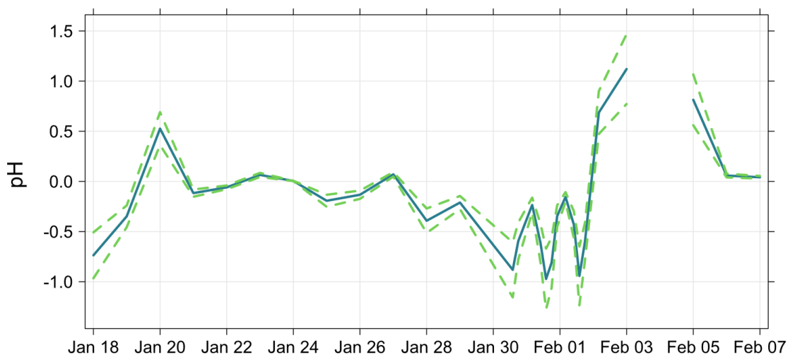
Figure 9: Predicted PM_{2.5} pH at the Bachok measurement site using ISOROPPIA-II (Fountoukis and Nenes, 2007). Dashed lines represent predictions of minimum and maximum limits of pH.
