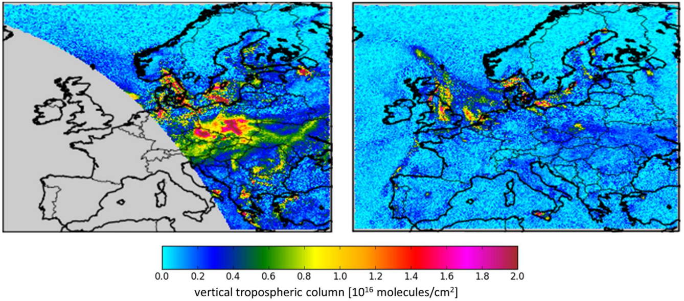
Figure 4 Example of two S4 NO 2 scenes, early morning, 4:00 UTC, and mid-day, 12:00 UTC, on 1 June 2003. Data is plotted for solar zenith angles < 85 degrees.
