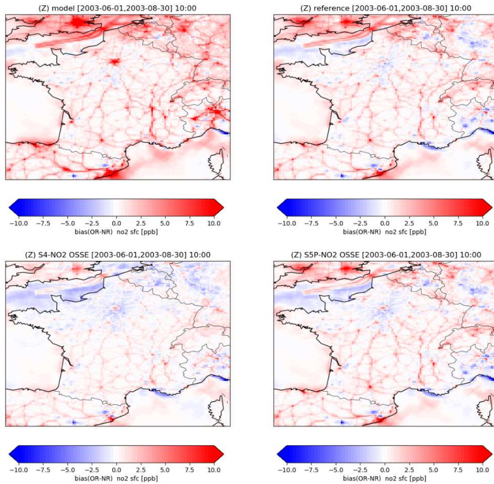
Figure 14 Zoom domain – summer, 10 UTC average. Bias with NR surface NO 2 before assimilation (top left), and after assimilation of ground-based O 3 (top right), ground-based O 3 +S4 NO 2 (bottom left) or ground-based O 3 +S5P NO 2 .
