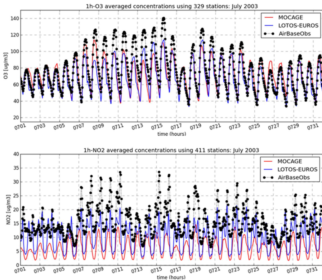
Figure 7 Time series of ozone (top) and NO 2 (bottom) concentration from NR (red, MOCAGE), CR (blue, LOTOS-EUROS) and AirBase background observations (black dots) for the period of July 2003.
