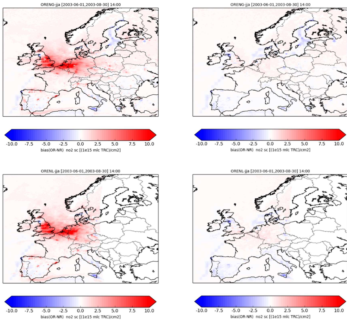
Figure 10 Summer period (JJA 2003) average NO 2 column bias at 14:00 UTC with synthetic observations for control run without assimilation (left column) and with assimilation of ground-based O 3 +S4 NO 2 (top row) and ground-based O 3 +S5P NO 2 (bottom row).
