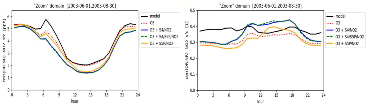
Figure 13 RMSE (left) and correlation (right) with NR surface NO 2 concentrations for the summer period and zoom domain. Prior (black line) and after assimilation of observations (coloured lines, ground-based O 3 only (dotted red), ground-based O 3 + S4 NO 2 (blue), ground-based O 3 + S5P NO 2 (yellow) or ground-based O 3 + S4 and S5P NO 2 (dashed green)).
