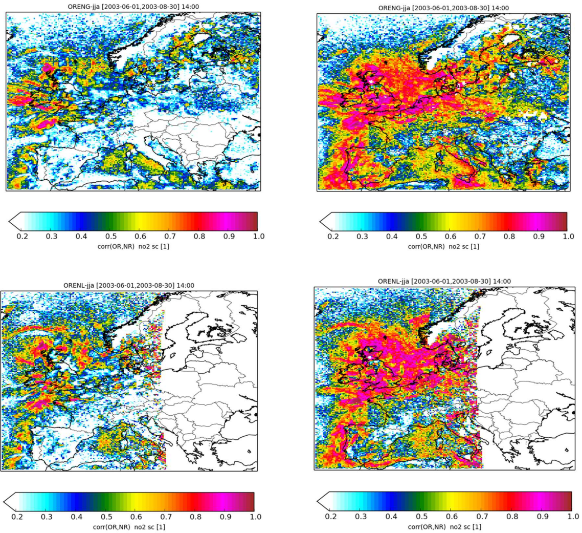
Figure 11 Summer period (JJA 2003) temporal correlation of modelled NO 2 columns at 14:00 UTC with synthetic observations for control run without assimilation (left column) and with assimilation of ground-based O 3 +S4 NO 2 (top row) and ground-based O 3 +S5P NO 2 (bottom row).
