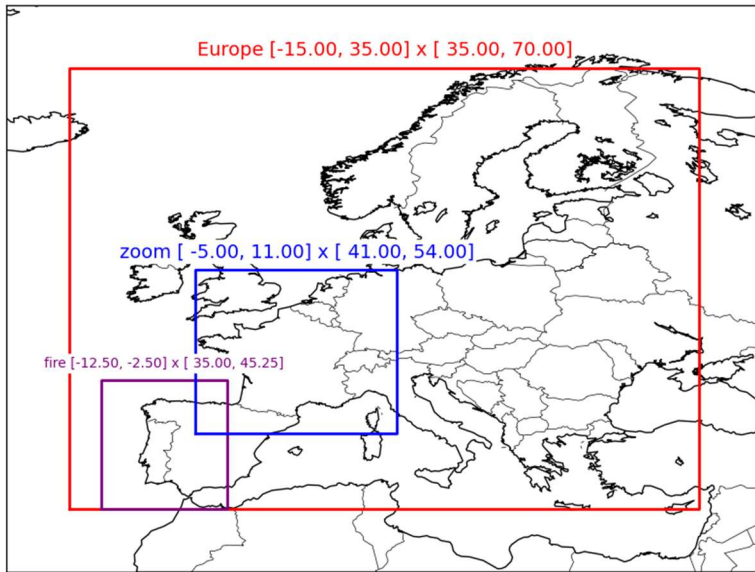
Figure 6 Illustration of different domains used for the assimilation runs. European domain (red rectangle), zoom domain (blue rectangle) and fire domain (purple rectangle).
