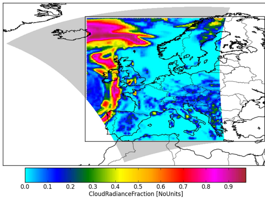
Figure 2 Example of the distribution of cloud radiance fractions for the simulated S5P 12:34 UTC overpass on 1 June 2003. The rectangle presents the European modelling domain.
