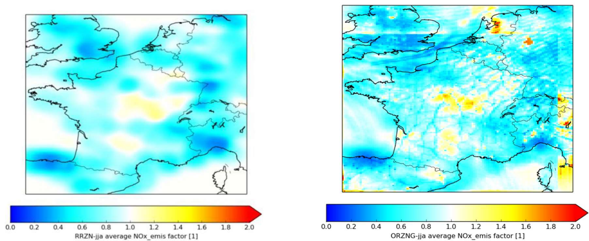
Figure 16 Average NO x emission increment for the run with assimilation of ground-based ozone observations only (RR) (left) and the S4 assimilation run (right) for the summer study period over the zoom domain.
