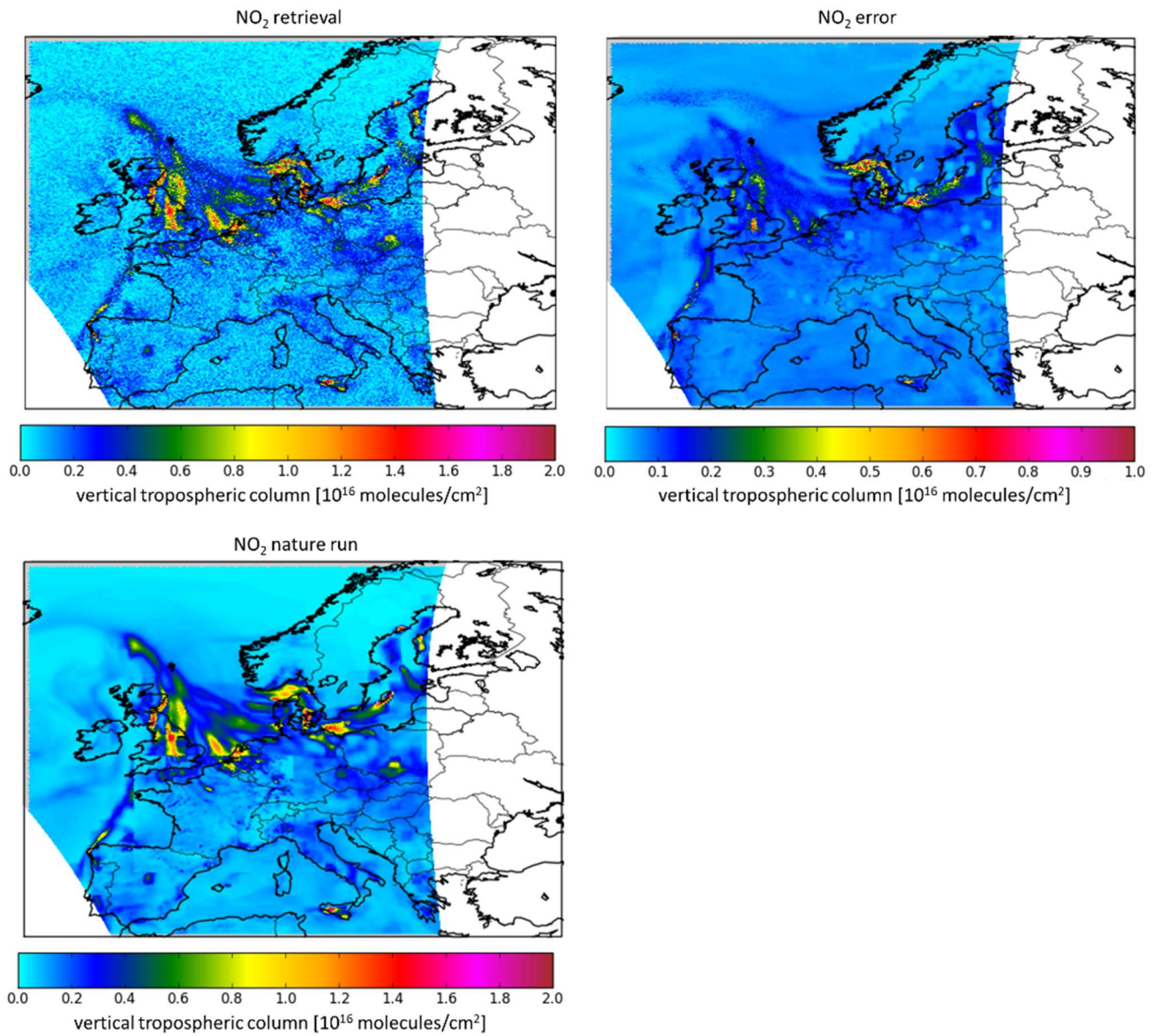
Figure 3 Example of the S5P synthetic retrieval of the NO 2 tropospheric column on 1 June 2003. The plots show the retrieved, noisy, NO 2 column (top left panel), the associated retrieval error (top right panel) and the NR result (bottom panel).
