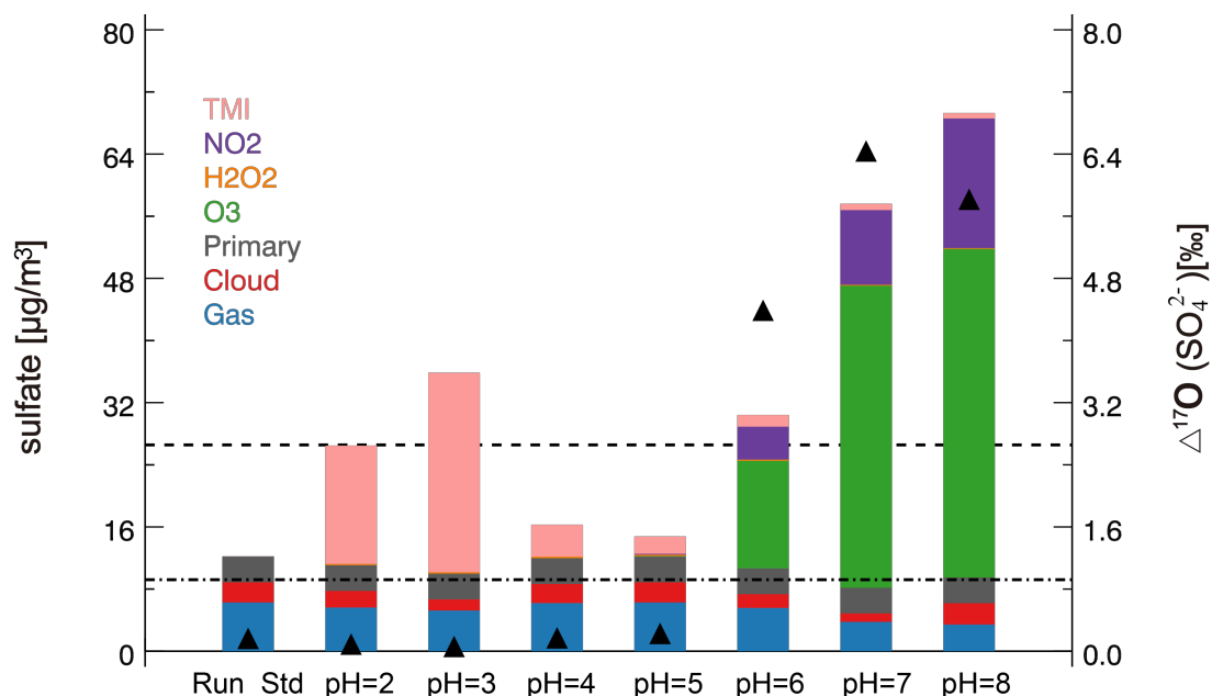
Figure 5. Model simulated mean sulfate concentration in Beijing averaged over heavy pollution periods (HPP as defined in the text). Model results are from the standard simulation (Run_Std) and sensitivity simulations with prescribed aerosol pH ranging 2 to 8. Different colors represent contributions from different sulfate formation pathways, including four heterogeneous reactions (oxidation by O 2 (TMI), NO 2 , H 2 O 2 , O 3 ), primary anthropogenic, aqueous-phase oxidation in clouds, and gas-phase oxidation. Also shown are the corresponding modeled \Delta^{17}\text{O}(\text{SO}_4^{2-}) values in Beijing (black triangles). The dashed line denotes observed mean sulfate concentration (25.9 \mu\text{g m}^{-3} ), and the dot-dashed line denotes observed mean \Delta^{17}\text{O}(\text{SO}_4^{2-}) (0.9‰) during HPP in Beijing.
