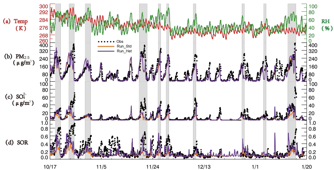
Figure 1. Time series of (a) GEOS-FP temperature (red line) and relative humidity (RH; green line), (b) \text{PM}_{2.5} and (c) sulfate concentration, and (d) SOR at the surface in Beijing during the study period of 17 October 2014 – 20 January 2015. Hourly \text{PM}_{2.5} , sulfate, and SOR observations (black dots) are compared with model results from Run_Std (orange line) and Run_Het (purple line). The gray shaded bars represent 10 heavy pollution periods (HPP) ( \text{PM}_{2.5} > 150 \mu\text{g m}^{-3} ) as defined in the text.
