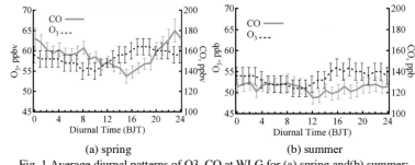
(a) spring (b) summer Fig.1 Average diurnal patterns of O 3 , CO at WLG for (a) spring and(b) summer; error bars indicate standard errors
