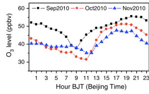
Fig 2. Diurnal cycle of O 3 concentration in Qinghai Lake area
