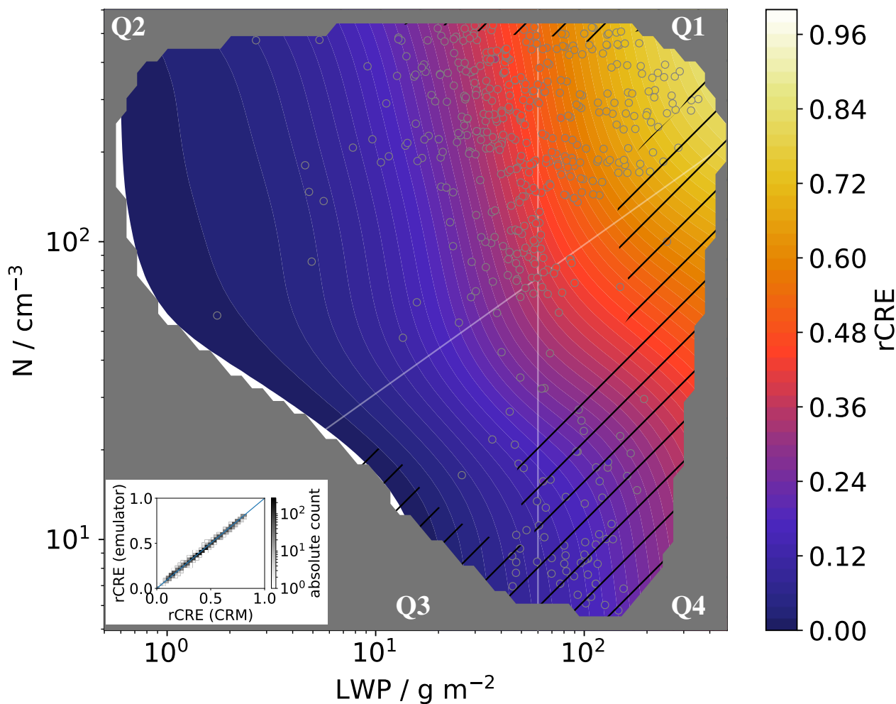
Figure 4. Emulated rCRE surface (ensemble mean Equation 3) as a function of LWP and droplet number N as color contours. The standard deviation \sigma of the emulated rCRE over the ensemble (Equation 4) is indicated by hatching, with \sigma < 0.01 and 0.01 < \sigma < 0.05 for non-hatched and hatched regions, respectively. Emulated values outside [0, 1] are masked. Color-filled circles show the validation subset of the total dataset shown in Figure 1 (see Section 3.1). For visibility only every 10th validation data point is shown. The scatter plots in the insets compare the complete validation dataset to the emulated values. White lines indicate quadrants as in Figure 1.
