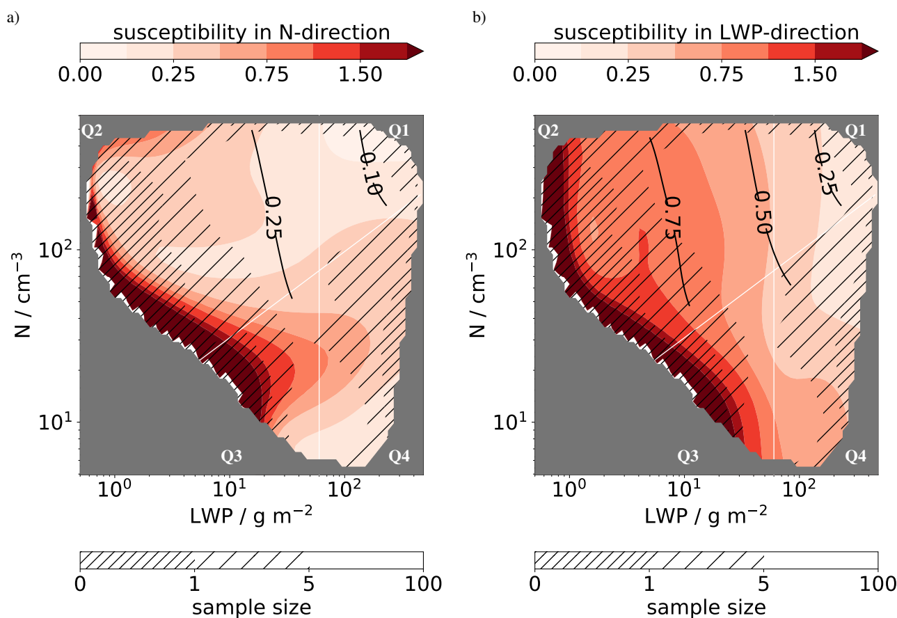
Figure 9. Partial susceptibilities of rCRE to (a) N and (b) LWP as a function of N and LWP as derived from the emulated rCRE surface (color contours). Solid lines show theoretical susceptibility values following Boers and Mitchell (1994), restricted to the non-drizzling region for which they apply. Hatchings indicate the sample size as in Figure 7. Note that sample sizes smaller than one trajectory can occur due to interpolation. White lines indicate quadrants as in Figure 1.
