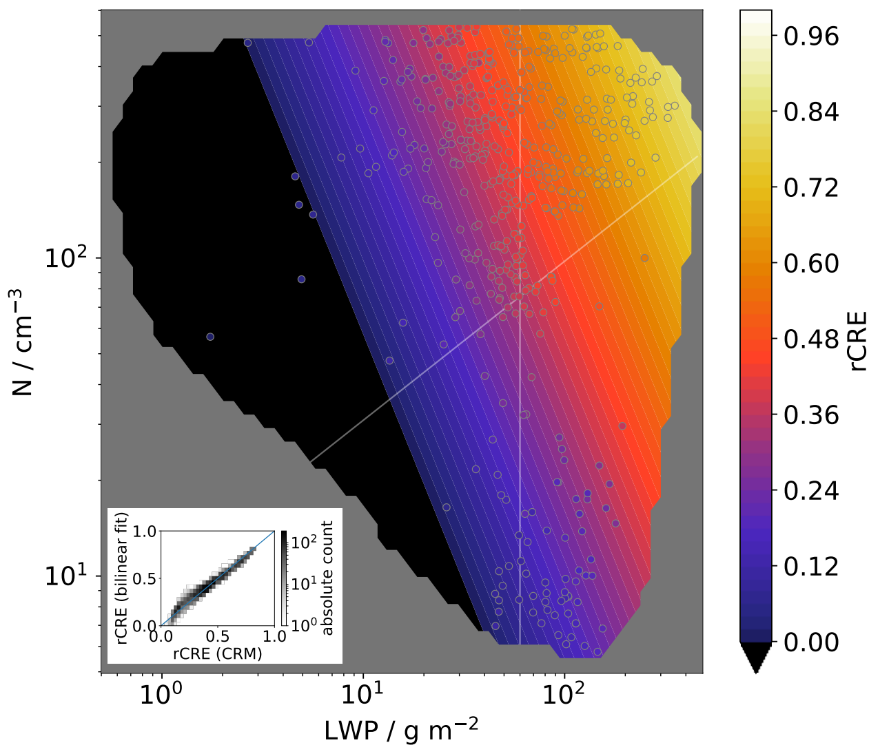
Figure 8. As Figure 4 but using bilinear regression rCRE = -0.86 + 0.40 \cdot \log_{10}(LWP) + 0.26 \cdot \log_{10}(N) instead of emulation to obtain the surface. The coefficient of determination of the regression amounts to r^2 = 0.95 and the rmse = 0.05 .
