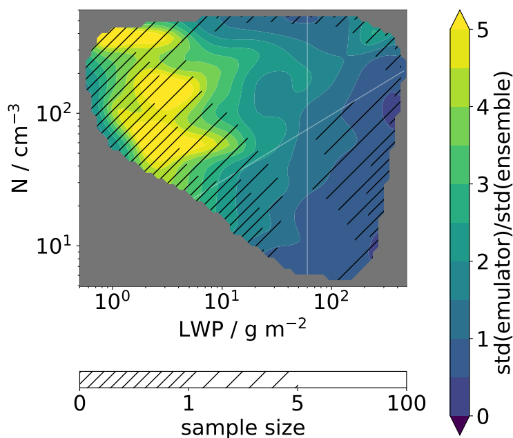
Figure 6. Comparison of errors from emulation, ensemble, and sampling. Contours show the ratio of emulator and ensemble standard deviation, hatchings show the sample size as in Figure 7. Note that sample sizes smaller than one trajectory can occur due to interpolation.
