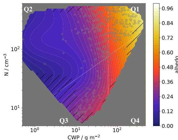
Figure 5. As Figure 4 but showing (a, b) cloud fraction and (c, d) cloud albedo as a function of (a, c) total liquid water path LWP and cloud droplet number concentration N and (b, d) cloud water path CWP and N . The standard deviation \sigma of the emulated rCRE over the ensemble (Equation 4) is indicated by hatching, with \sigma < 0.01 , 0.01 < \sigma < 0.05 and 0.05 < \sigma < 0.5 for non-hatched, single-hatched, and double-hatched regions, respectively.
