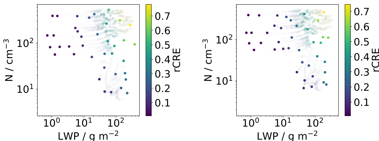
Figure 2. Sub-sampling (solid circles) from the total training data (opaque points) for the rCRE emulator ensemble members with the (left) lowest and (right) highest root mean square error (rmse) in predicting the validation data. The rmse values are 0.010 and 0.024, respectively.
