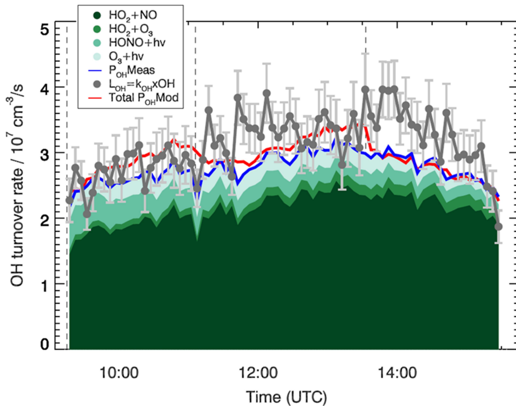
5 Figure 3: OH budget for the MBO experiment. The experimentally determined total OH loss rate, L_{\text{OH}} , and individual production terms are shown. For comparison, the red line indicates the total modelled OH production, P_{\text{OH, Mod}} , which equals the modelled loss rate. Vertical dashed lines indicate the times when MBO was injected. Error bars ( 1\sigma ) for L_{\text{OH}} include the accuracy of measurements.
