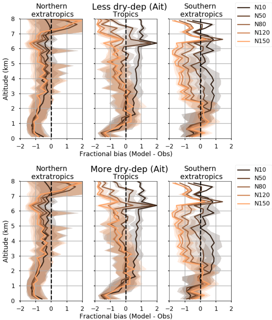
5 Figure 17: The vertical profile of fractional bias in modelled aerosol number at different size cut-offs for measurements in the Northern extratropics (a), the Tropics (b), and the Southern extratropics (c) with reduced (x0.5) and increased (x2.0) dry-deposition in the Aitken mod.
