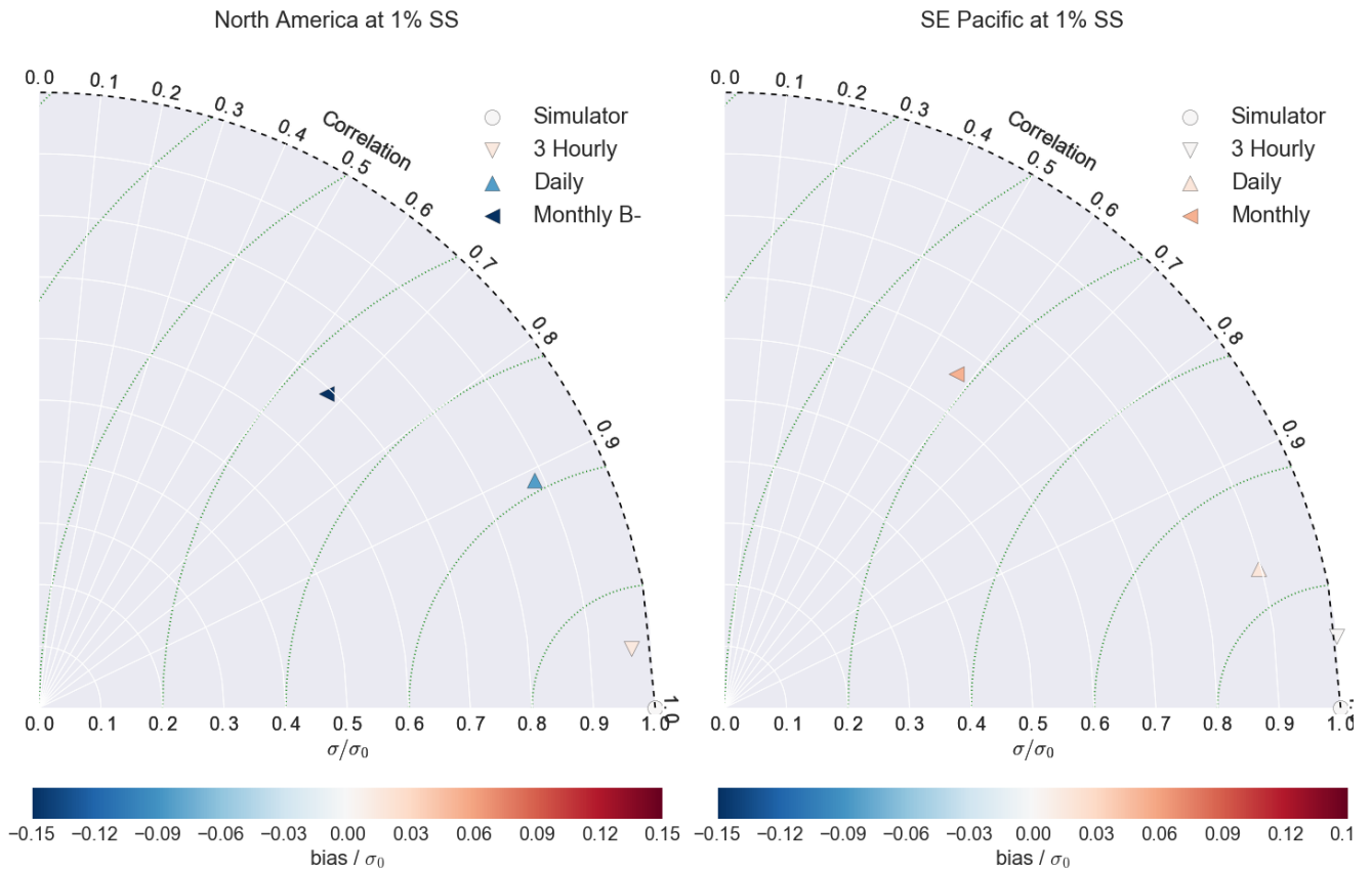
Figure 2: Taylor diagram showing the RMS error and reduction in correlation and variability introduced by comparing instantaneous model output (using a flight track simulator) with interpolations from different temporal aggregations of the same model data. All datasets are linearly interpolated from the same underlying 4-D model field (CCN at 1% supersaturation) and compared with an online interpolation. (a) shows points taken over North America, (b) shows points over the South East Pacific.
