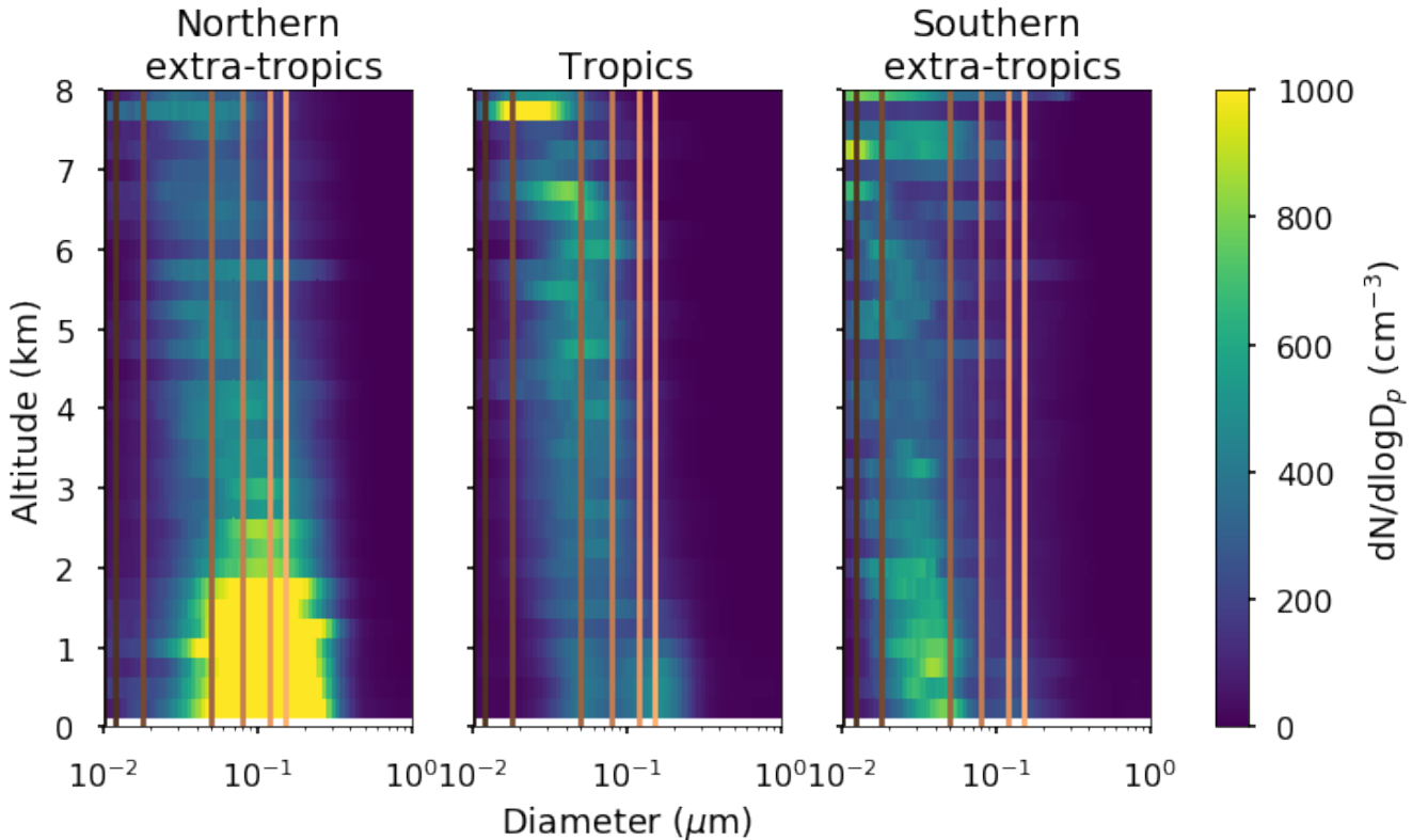
10 Figure 3: The median aerosol number size distribution observed at each altitude across all flights in the Northern extra-tropics (a), Tropics (b) and Southern extra-tropics (c). The copper lines represent the sizes from which the integrated numbers in e.g. Figure 4 are calculated.
