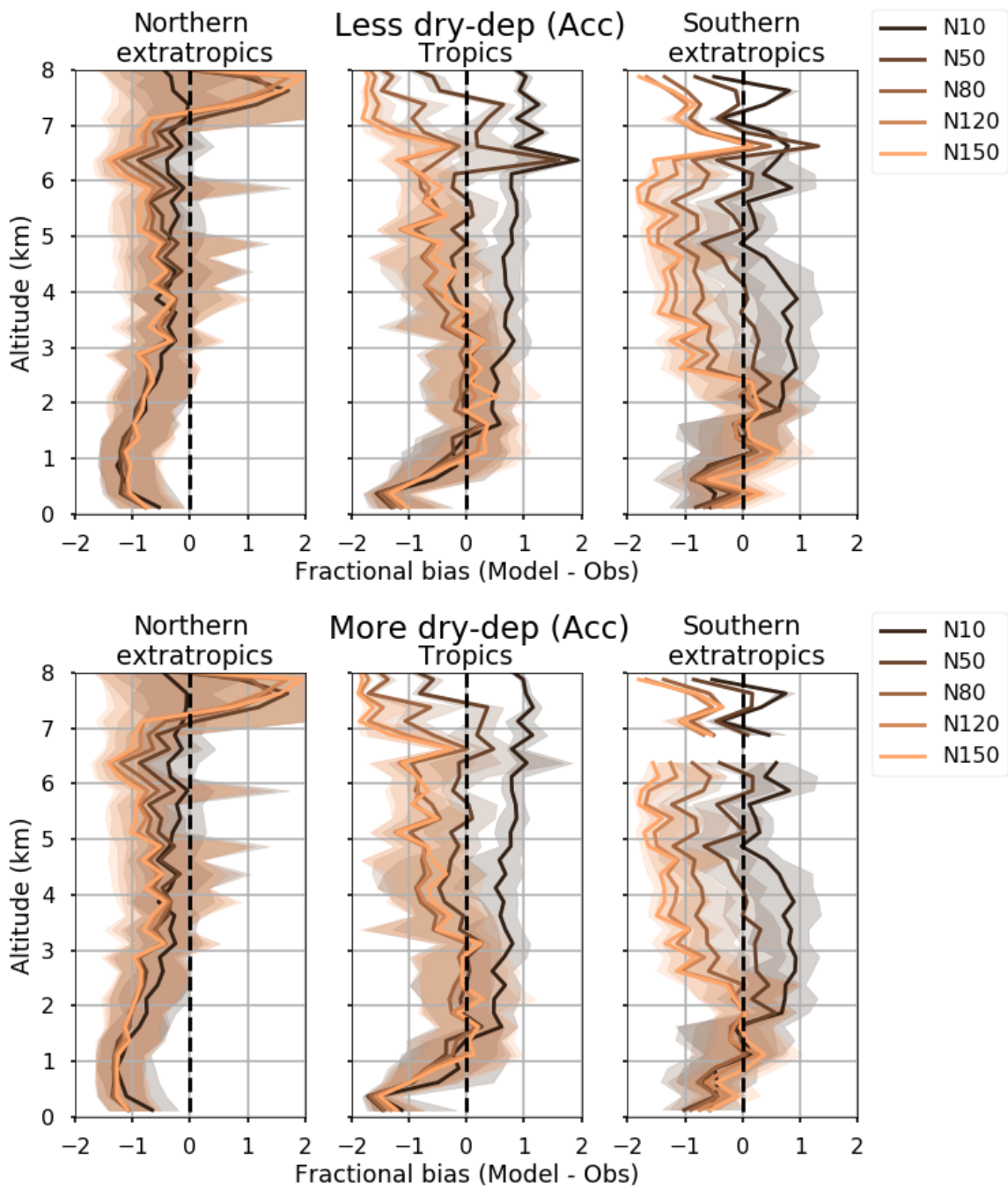
5 Figure 16: The vertical profile of fractional bias in modelled aerosol number at different size cut-offs for measurements in the Northern extratropics (a), the Tropics (b), and the Southern extratropics (c) with reduced (x0.1) and increased (x10) dry-deposition in the accumulation mode.
