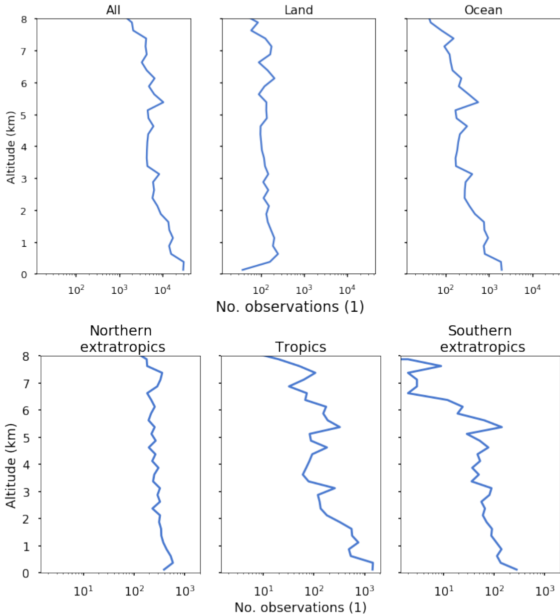
5 Figure 13: The number of observations (and model points) used in each altitude bin for different subsets of the data used throughout the analysis.
