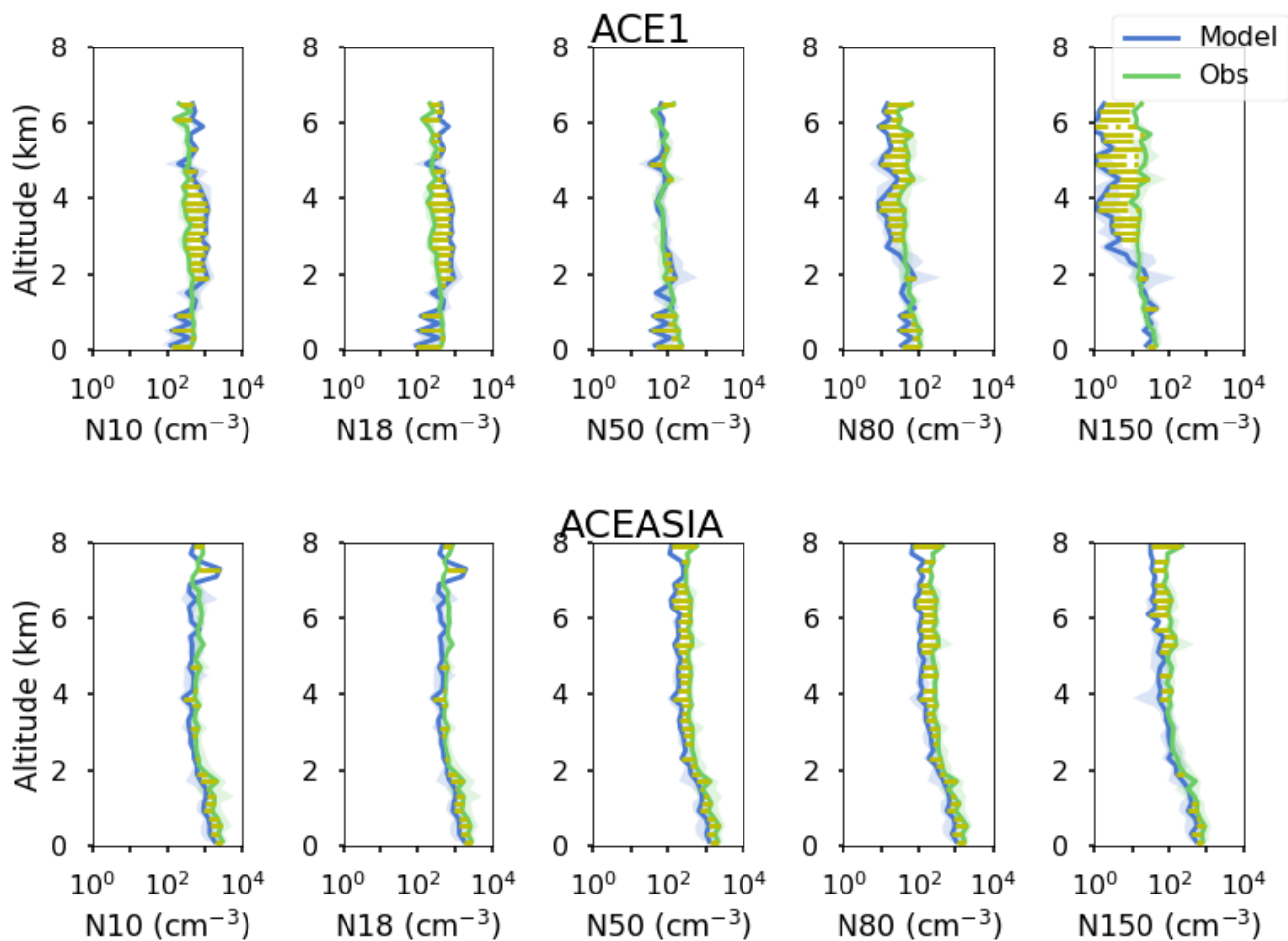
Figure 18: Per-campaign median profiles of aerosol number at different sizes. Yellow lines indicate a significant difference at that altitude.
