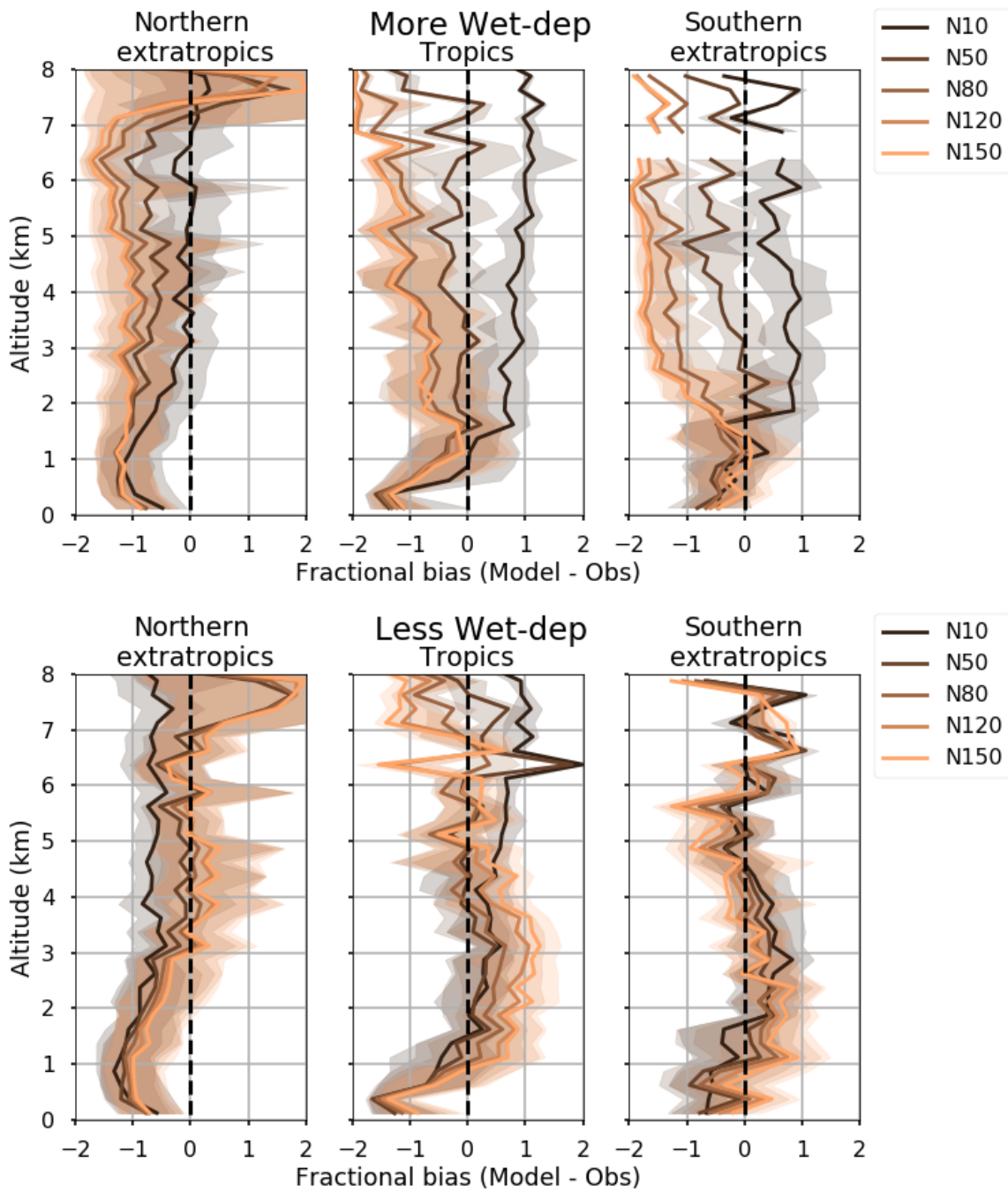
Figure 8: The vertical profile of fractional bias in modelled aerosol number at different size cut-offs for measurements in the Northern extratropics (a), the Tropics (b), and the Southern extratropics (c) with increased (x2) and decreased (x0.5) wet-deposition rate.
