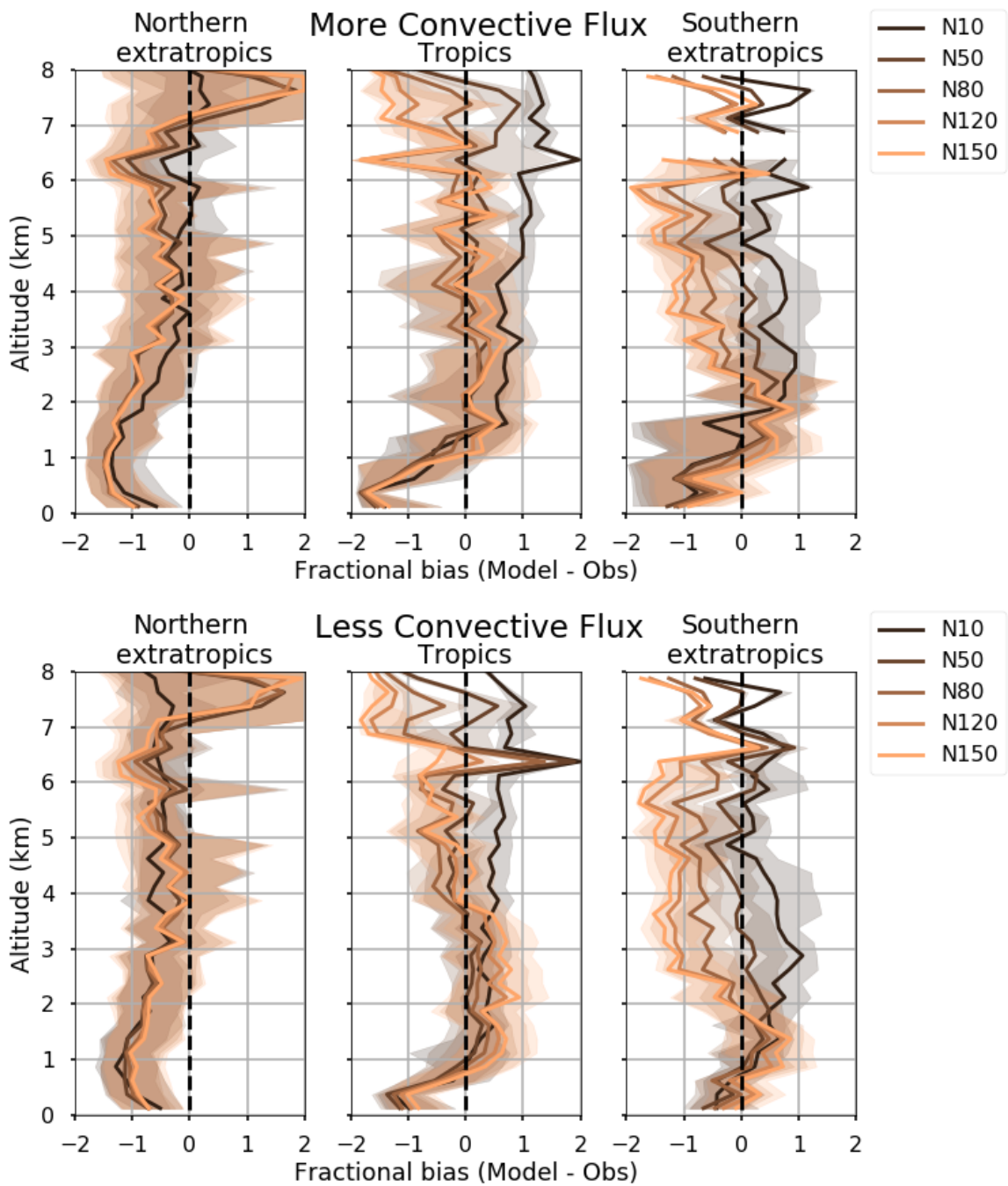
5 Figure 9: The vertical profile of fractional bias in modelled aerosol number at different size cut-offs for measurements in the Northern extratropics (a), the Tropics (b), and the Southern extratropics (c) with increased (x10) and decreased (x0.1) convective tracer entrainment rate.
