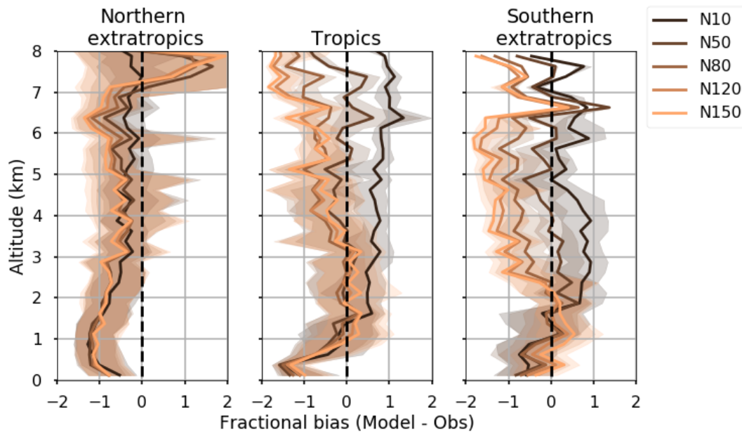
Figure 6: The vertical profile of fractional bias in modelled aerosol number at different size cut-offs for measurements in the Northern extratropics (a), the Tropics (b), and the Southern extratropics (c).
