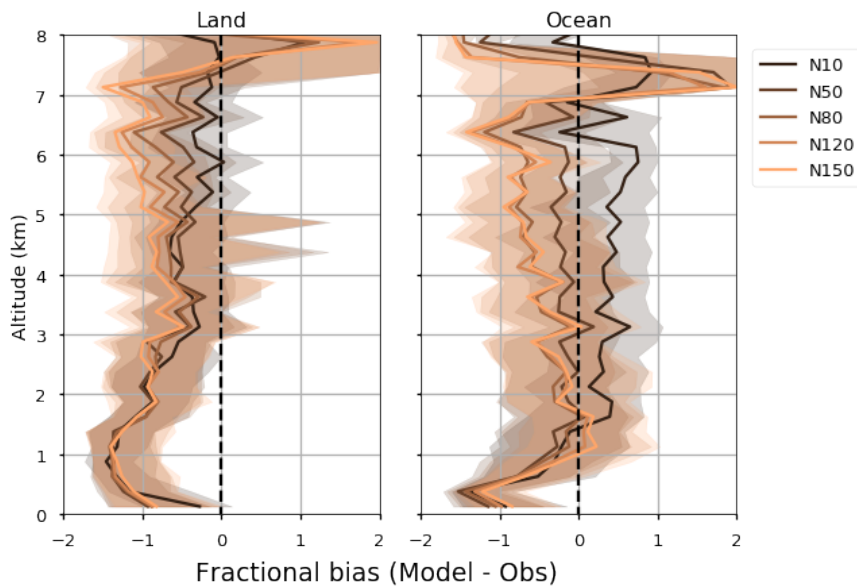
Figure 5: The vertical profile of fractional bias in modelled aerosol number at different size cut-offs for Land (a) and Ocean (b) measurements.
