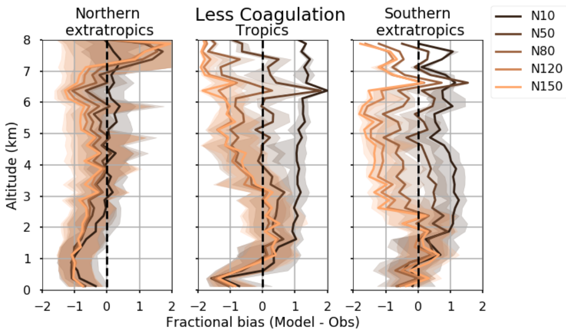
5 Figure 10: The vertical profile of fractional bias in modelled aerosol number at different size cut-offs for measurements in the Northern extratropics (a), the Tropics (b), and the Southern extratropics (c) with increased (x2.0) and decreased (x0.5) coagulation rate.
