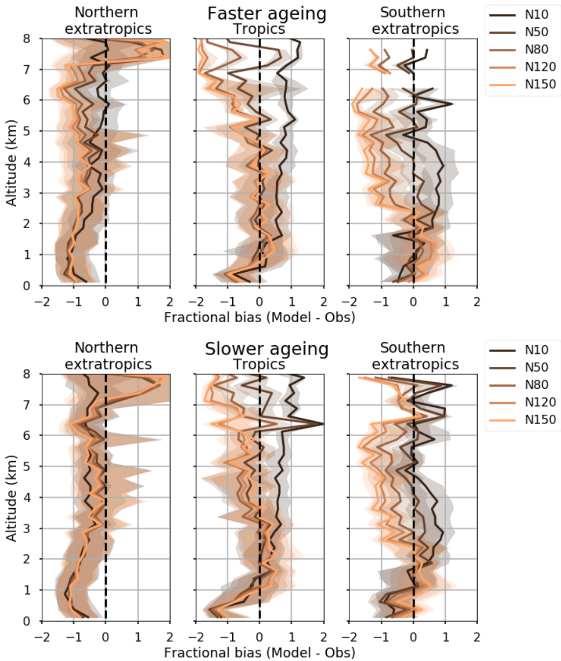
5 Figure 7: The vertical profile of fractional bias in modelled aerosol number at different size cut-offs for measurements in the Northern extratropics (a), the Tropics (b), and the Southern extratropics (c) with a faster (0.3 mono-layers required) and slower (5 mono-layers) condensational ageing rate.
