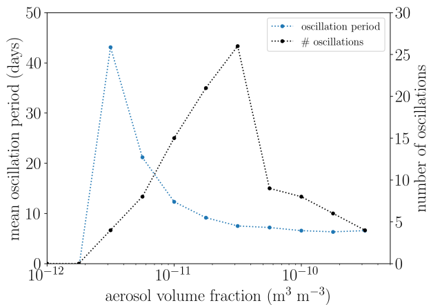
Figure 12. Oscillation characteristics depending on the aerosol volume fraction after 200 days
