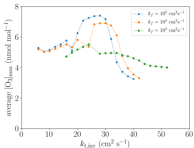
Figure 10. Dependence of the oscillation characteristics on the variations of k_{t,inv} and k_f , Figs. 10a–10c, and the variation of the mixing ratios of \text{O}_3 and Br at two different heights of 100 m and 225 m for the base settings, Fig. 10d
