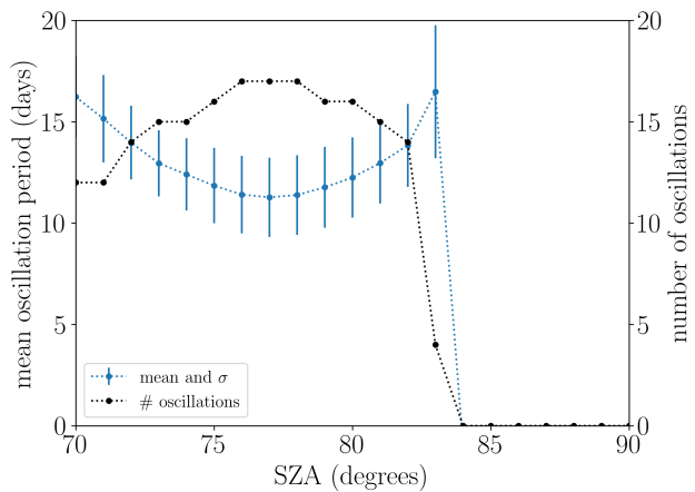
Figure 13. (a) Mean oscillation period and number of oscillations versus the solar zenith angle during 200 days. (b) Evolution of the mixing ratios of \text{O}_3 and the bromine species for SZA = 70°
