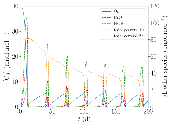
Figure 6. Oscillation and termination of ODEs for different values of k_{t,inv}
