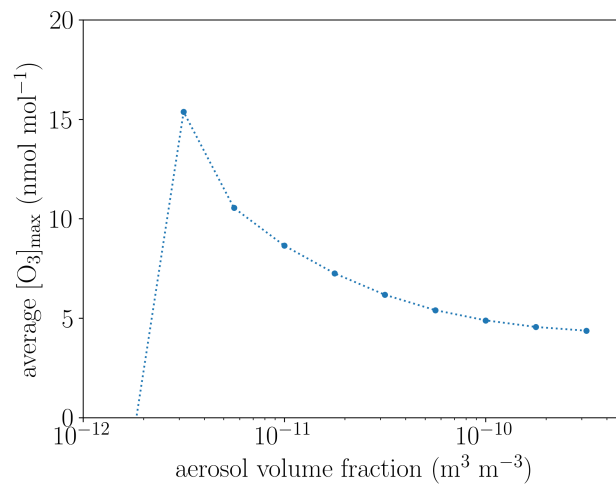
Figure 12. Oscillation characteristics depending on the aerosol volume fraction after 200 days
