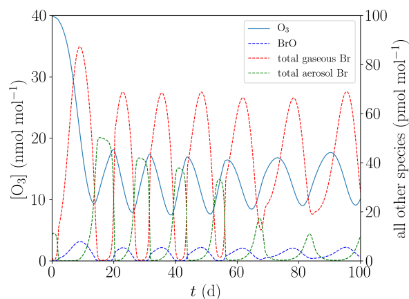
Figure 13. (a) Mean oscillation period and number of oscillations versus the solar zenith angle during 200 days. (b) Evolution of the mixing ratios of \text{O}_3 and the bromine species for SZA = 70°
