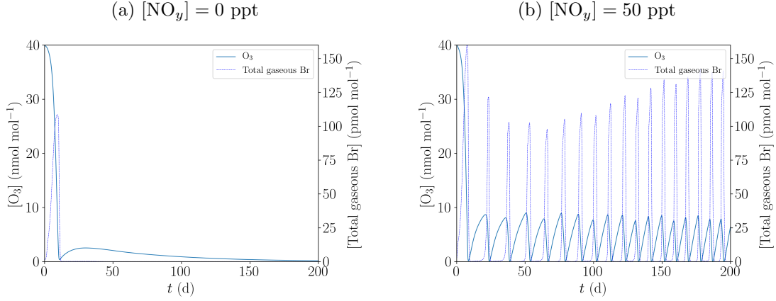
Figure R1: Base case simulations with k_{\text{inv}} = k_f = 10 \text{ cm s}^{-1} for [\text{NO}_y] = 0 and 50 ppt.
