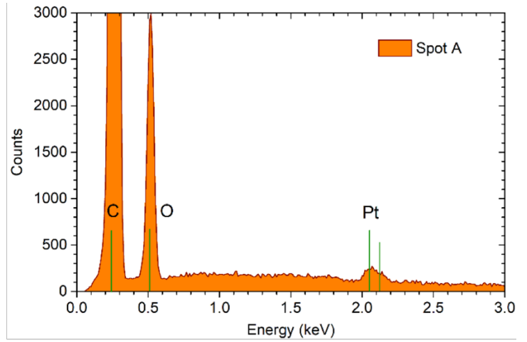
Figure 4: Morphology and composition of a fullerene soot particle extracted from the Marin-5 nebulizer output on a Nuclepore™ filter. Left panel: the SEM secondary electron image. Right panel: EDX-spectrum obtained from spot A on the particle (marked by the orange circle in the SEM image). The spectrum shows a pure carbonaceous signature with only the C and O peaks. Sample coating is responsible for the Pt peak at 2.08 keV.
