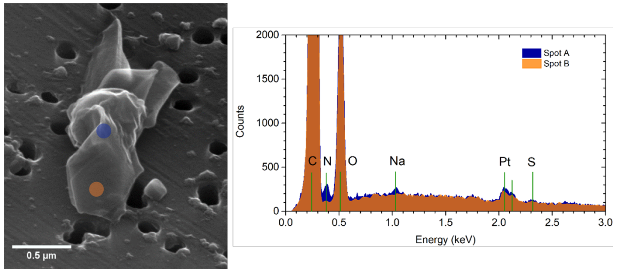
600 Figure 10: Same as Fig. 4 but for a biological. EDX-spectra obtained from different areas on the particle (marked as color spots in the image). A clear biogenic signature (N, S, Na) is visible for the central bulky part suggesting intracellular composition (spot A, blue color), whereas the exterior part of the particle shows pure carbonaceous compounds (C, O) (spot B, orange color). Sample coating is responsible for the platinum peak. ❌
