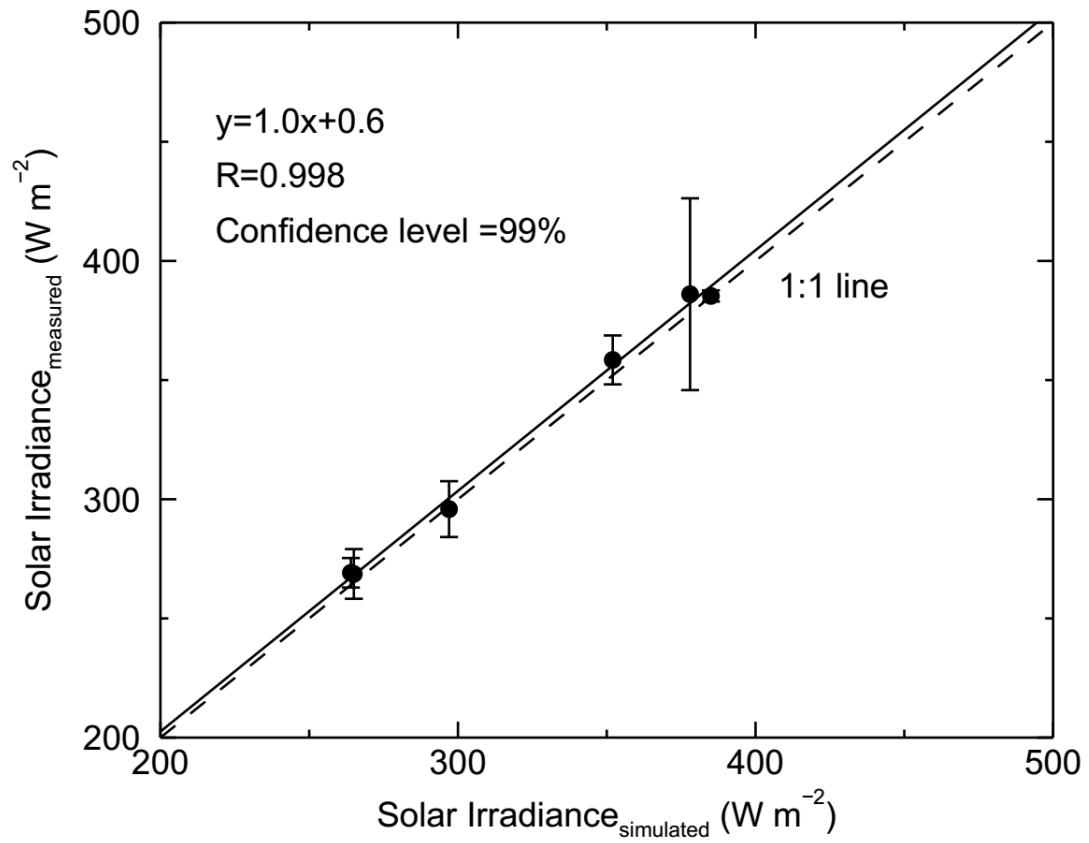
1 2 Figure S1. A comparison of the SBDART-simulated and ASD-measured solar 3 irradiance values in January 2014.
