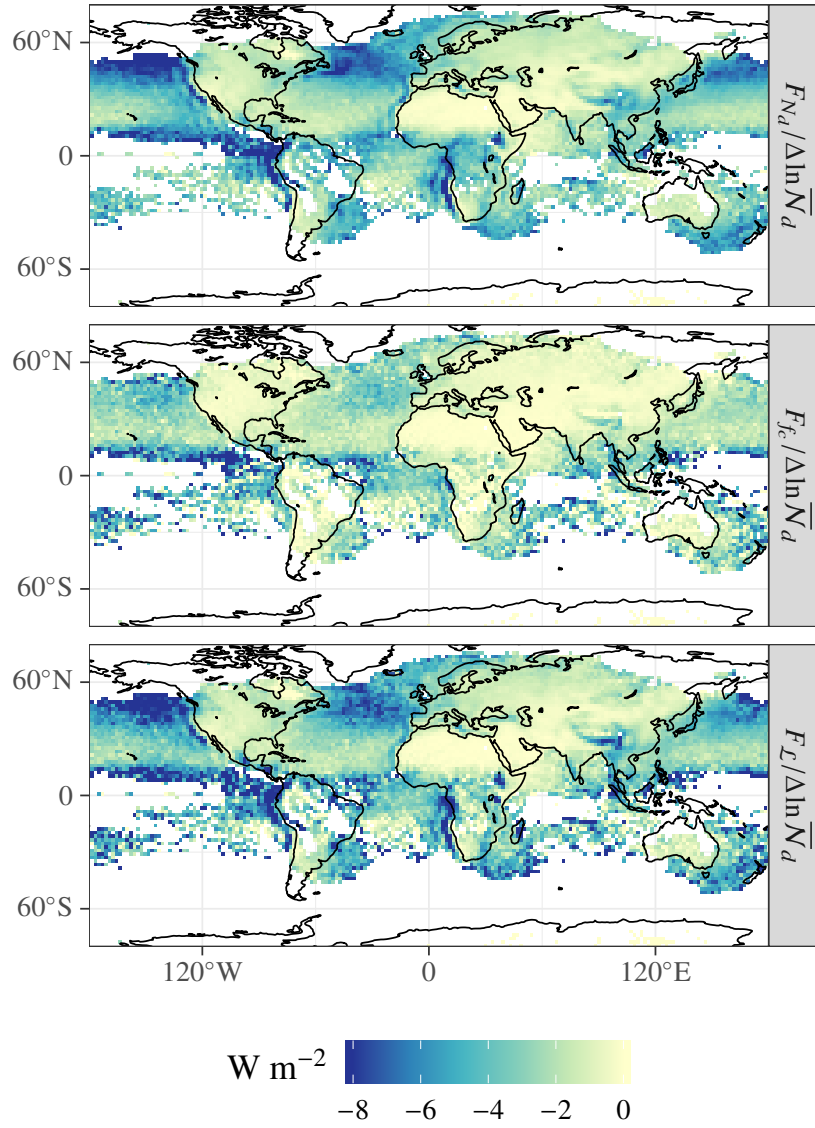
Figure 2. Sensitivity of ERF aci components to anthropogenic N_d change (shown only where \Delta \ln \overline{N_d} > 0.05 )
