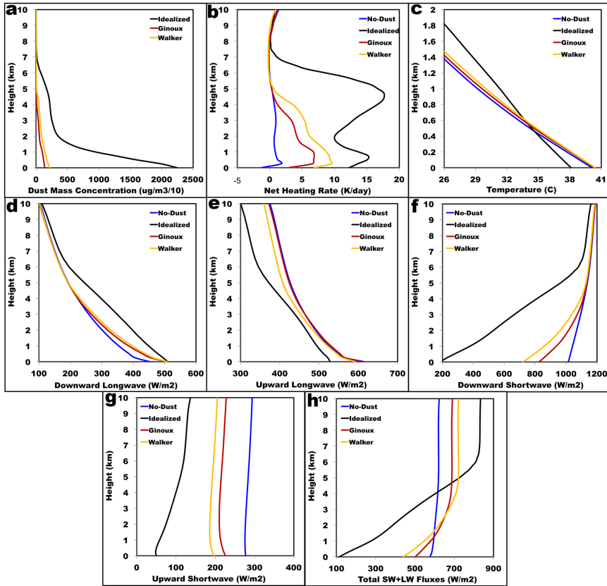
5 Figure 9. Daytime 1000 UTC (~1400 LST) 4 August vertical profiles of analysis-area averaged: (a) dust mass concentration ( \mu\text{g m}^{-3} 10^{-1} ), (b) net radiative heating rate ( \text{K day}^{-1} ), (c) temperature ( ^{\circ}\text{C} ), (d) downward longwave ( \text{W m}^{-2} ), (e) upward longwave ( \text{W m}^{-2} ), (f) downward shortwave ( \text{W m}^{-2} ), (g) upward shortwave ( \text{W m}^{-2} ), and (h) total radiative fluxes ( \text{W m}^{-2} ) computed as the sum of shortwave and longwave, downward minus upward fluxes. Note that panel (c) is on a different vertical scale so as to zoom in on lower-level temperature.
