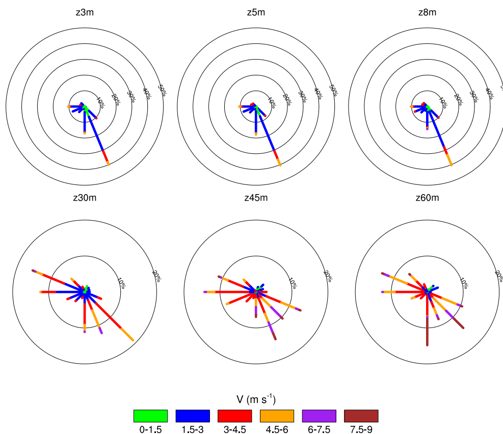
Figure 3. Night-time IOPs (nIOPs) wind roses for each level of the Skinflow mast and the Valimev tower during the BLLAST field campaign. Circles represent a 10% frequency increment.
