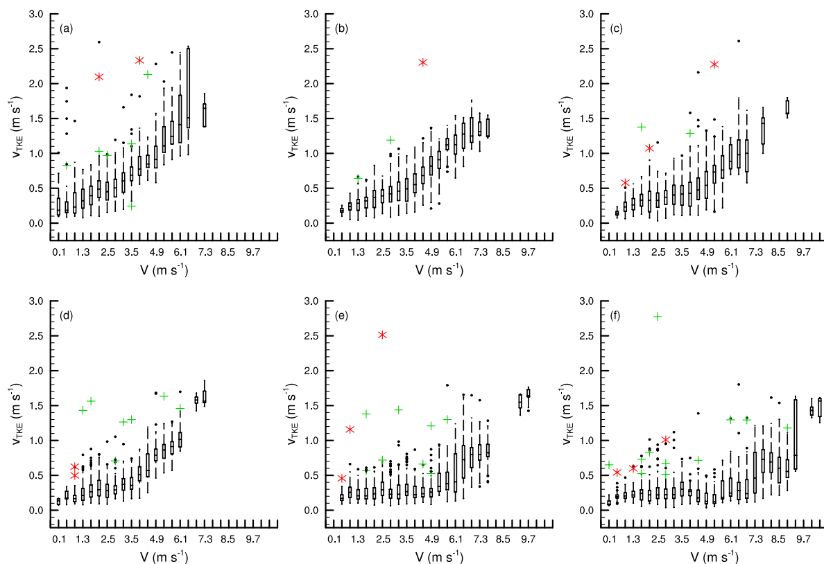
Figure 10. Box plots of the relationship between the bin-averaged turbulence strength V_{TKE} and the wind speed V for the Valimev dataset for the whole BLLAST field campaign. Top row figures correspond to the NW's direction range for (a) NW's at z_{30m} , (b) NW's at z_{45m} , and (c) NW's at z_{60m} and the bottom row corresponds to the SE's directions, (d) SE's at z_{30m} , (e) SE's at z_{45m} and (f) SE's at z_{60m} . The outliers represent a turbulence enhancement due to a quick variation of the wind speed ( \Delta V > 1 \text{ m s}^{-1} ) (green crosses), due to a sharp change in the wind direction ( \Delta dir > 75^\circ ) (red asterisks) or due to any other factor (black dots).
