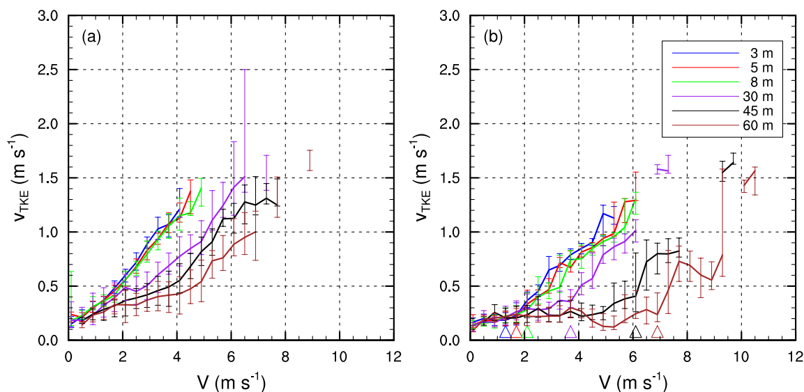
Figure 8. Relationships between the bin-averaged turbulence strength V_{TKE} and the wind speed V for the whole BLLAST field campaign for the main considered directions: (a) wind coming from 225^\circ to 45^\circ (included), named NW's, and (b) winds coming from 45^\circ to 225^\circ (included), named SE's. Each line represents the median within each 0.4 \text{ m s}^{-1} V bin. The vertical lines represent the deviation for each V bin with the low limit corresponding to Q1 and the upper limit to Q3. The threshold wind speed V_T is marked with a triangle with the heights colours in (b).
