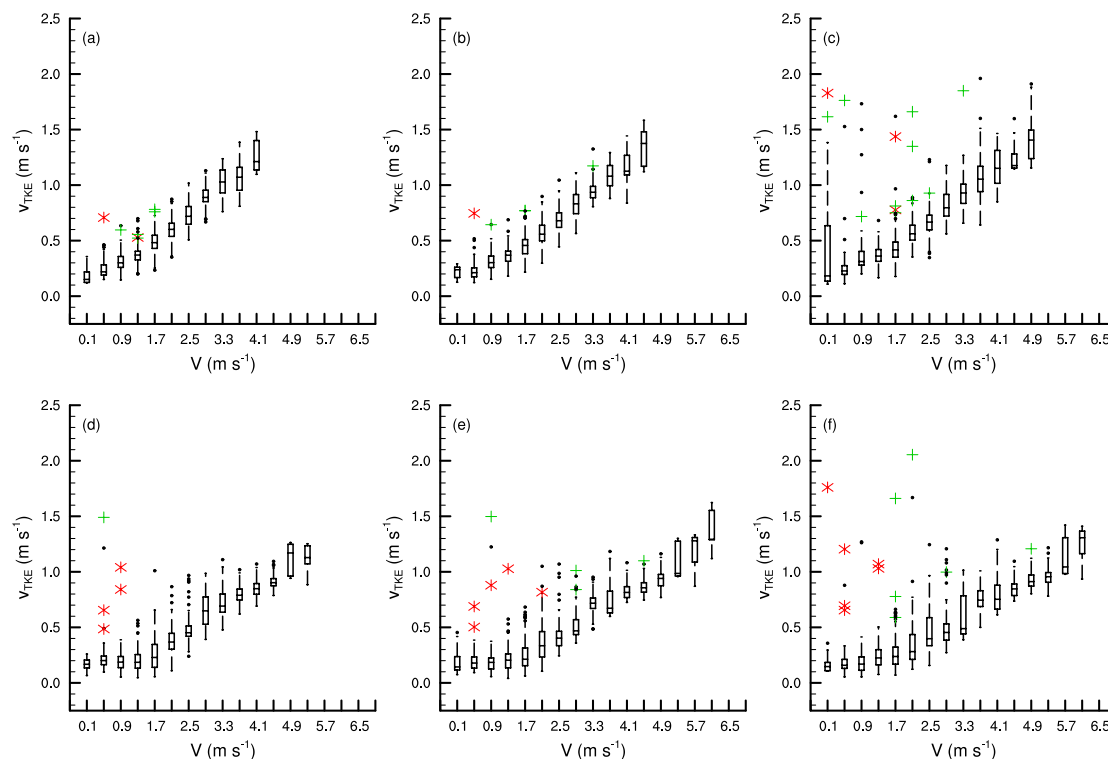
Figure 9. Box-plot of the relationship between the bin-averaged turbulence strength V_{TKE} and the wind speed V for the Skinflow night-time dataset for the whole BLLAST field campaign. The top row figures correspond to the NW's direction range for (a) NW's at z_{3m} , (b) NW's at z_{5m} , and (c) NW's at z_{8m} and the bottom row corresponds to the SE's directions, (d) SE's at z_{3m} , (e) SE's at z_{5m} and (f) SE's at z_{8m} . The outliers represent a turbulence enhancement due to a quick variation of the wind speed (greater than 1 \text{ m s}^{-1} ) (green crosses), due to a sharp change in the wind direction (greater than 75^\circ ) (red asterisks) or due to any other factor (black dots).
