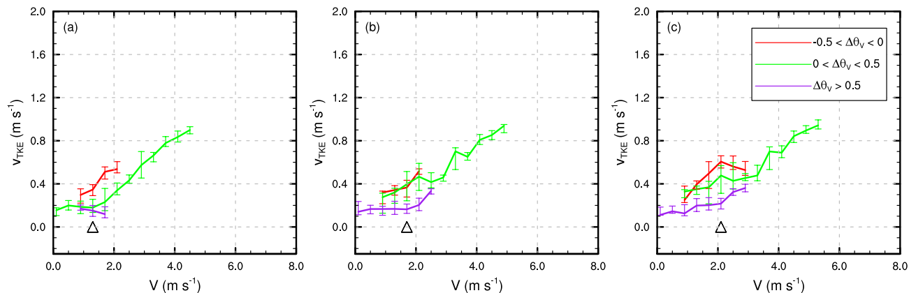
Figure 7. Relationship between the bin-averaged turbulence strength V_{TKE} and the wind speed V during the BLLAST campaign nIOPs as a function of potential temperature difference intervals, defined as, \Delta\bar{\theta}_v = \bar{\theta}_v(z) - \bar{\theta}_{v_{z_0}} , where \bar{\theta}_{v_{z_0}} is the virtual potential temperature of reference at 2 m, and \bar{\theta}_v(z) the virtual potential temperature at each height z : (a) z_{3m} , (b) z_{5m} , and (c) z_{8m} . The wind speed threshold V_T is marked with a black triangle for each height (a) z_{3m} , (b) z_{5m} , and (c) z_{8m} .
