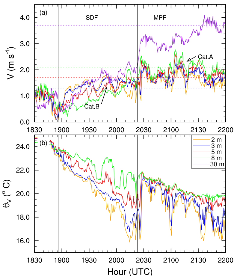
Figure 12. Time series of (a) horizontal wind speed and (b) virtual potential temperature for the 2 of July (nIOP09) during the BLLAST field experiment for z_{2m} , z_{3m} , z_{5m} , z_{8m} and z_{30m} . The shallow drainage flow (SDF) stage is indicated between 1855 and 2020 UTC, and a consecutive mountain-plain wave (MPF) stage thereafter. Both stages originated transitions between regime 1 to regime 2 (category A), and enhancement of turbulence within regime 1 (category B). The potential temperature is not represented for z_{30m} because there is only thermocouple measurements for the Skinfoam mast ( z_{2m} - z_{8m} ). The wind speed threshold for several levels are marked with the dashed line to better illustrate the transitions, whilst some transitions between regime 1 and regime 2 are marked with an arrow. The data shown herein is the 30 s temporal average from sonic anemometers with a frequency of 10 Hz.
