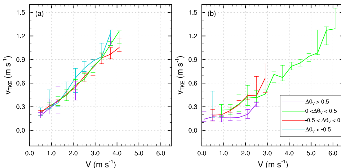
Figure 11. Relationship between the bin-averaged turbulence strength V_{TKE} and the wind speed V during the BLLAST campaign nIOPs as a function of potential temperature difference intervals, defined as, \Delta\bar{\theta}_v = \bar{\theta}_v(z) - \bar{\theta}_{v_{z_0}} , where \bar{\theta}_{v_{z_0}} is the virtual potential temperature of reference at 2 m, and \bar{\theta}_v(z) the virtual potential temperature at the height of z_{5m} for: (a) NW's direction range and (b) SE's direction range. The wind speed threshold V_T for z_{5m} is marked with a black triangle in (b).
