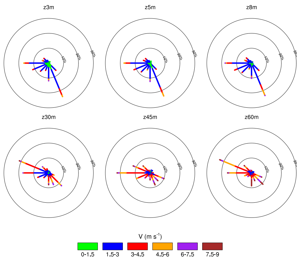
Figure 4. Night-time whole dataset wind roses for each level of the Skinflow mast and the Valimev tower during the BLLAST field campaign. Circles represent a 10% frequency increment.
