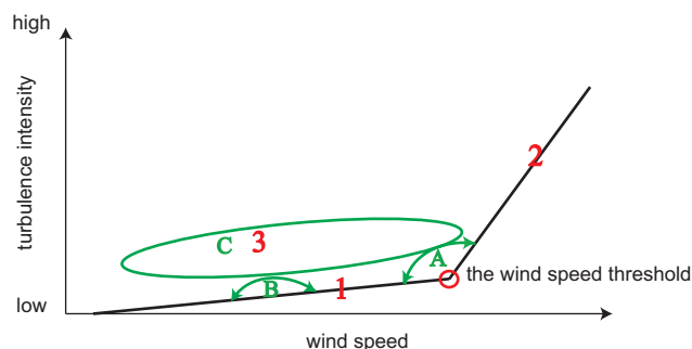
Figure 1. Schematic representation of the HOckey-STick (HOST) theory with the three turbulence regimes (regime 1, 2 and 3) and the three turbulence intermittency categories (cat. A, cat. B and cat. C). Reproduced from Figure 2 of Sun et al. (2012) ©American Meteorological Society. Used with permission.
