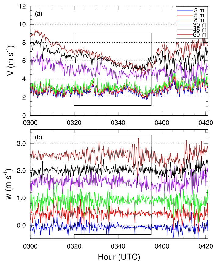
Figure 13. Times series of (a) horizontal wind speed V and (b) vertical wind speed, w (incremented 0.5 \text{ m s}^{-1} for an easy comparison) for 26 June 2011 at z_{3m} , z_{5m} , z_{8m} , z_{30m} , z_{45m} and z_{60m} . The black rectangle localises the top-down event. The data shown herein is the 10 s temporal average from sonic anemometers with a frequency of 10 Hz.
