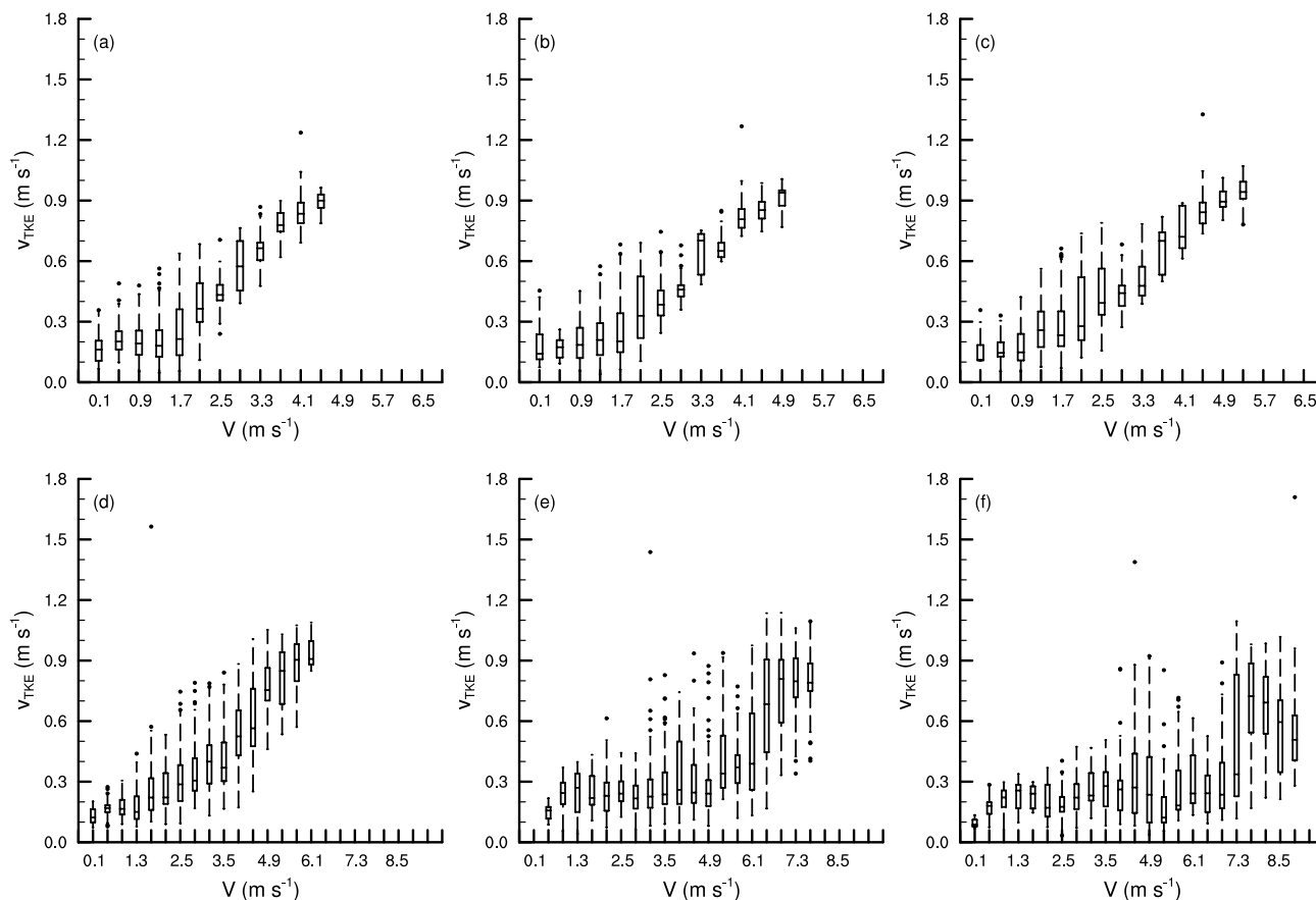
Figure 6. Box plots of the relationship between the bin-averaged turbulence strength V_{TKE} and the wind speed V for the nIOPs of the BLLAST field campaign. Data correspond to the Skinflow mast and to the Valimev tower at different heights, (a) z_{3m} , (b) z_{5m} and (c) z_{8m} Skinflow mast levels, and (d) z_{30m} , (e) z_{45m} and (f) z_{60m} Valimev tower levels.
