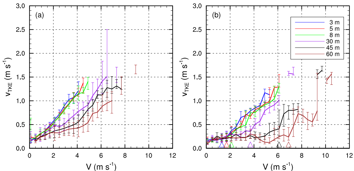
Figure 7. Relationships between the bin-averaged turbulence strength V_{TKE} and the wind speed V for the whole BLLAST field campaign for the main considered directions: (a) wind coming from 225° to 45° (included), named NW's, and (b) winds coming from 45° to 225° (included), named SE's. Each line represents the median within each 0.4 \text{ m s}^{-1} V bin. The vertical lines represent the deviation for each V bin with the low limit corresponding to Q1 and the upper limit to Q3. The threshold wind speed V_T is marked with a triangle with the heights colours in (b).
