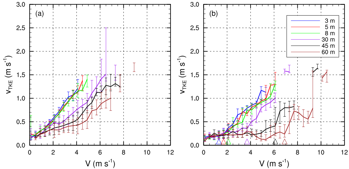
Figure 7. Relationships between the bin-averaged turbulence strength V_{TKE} and the wind speed V for the whole BLLAST field campaign for the main considered directions: (a) wind coming from 225^\circ to 45^\circ (included), named NW's, and (b) winds coming from 45^\circ to 225^\circ (included), named SE's. Each line represents the median within each 0.4 \text{ m s}^{-1} V bin. The vertical lines represent the deviation for each V bin with the low limit corresponding to Q1 and the upper limit to Q3. The threshold wind speed V_T is marked with a triangle with the heights colours in (b).
