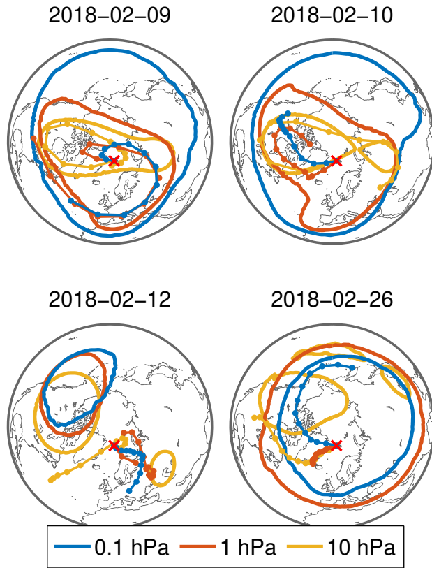
Figure 12. The solid lines indicate the contour of the polar vortex at 10 hPa, 1 hPa and 0.1 hPa during the major SSW of 2018. The line with dots shows the LAGRANTO 3-day backward trajectory at the same altitudes. The red cross indicates the location of Ny-Ålesund.
