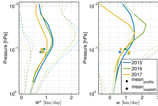
Figure 9. Vertical component of the residual mean meridional circulation \bar{w}^* and zonal mean vertical wind w profiles averaged between September 15 and November 1 for the years 2015, 2016 and 2017. The dashed line is the standard deviation and the bold line indicates the altitude range which was covered by the zonal mean 5.5 ppm isopleth of SD-WACCM in the same time period. The points indicate the mean of the profiles over this altitude range and the stars indicate the mean along the zonal mean 5.5 ppm isopleth of SD-WACCM.
