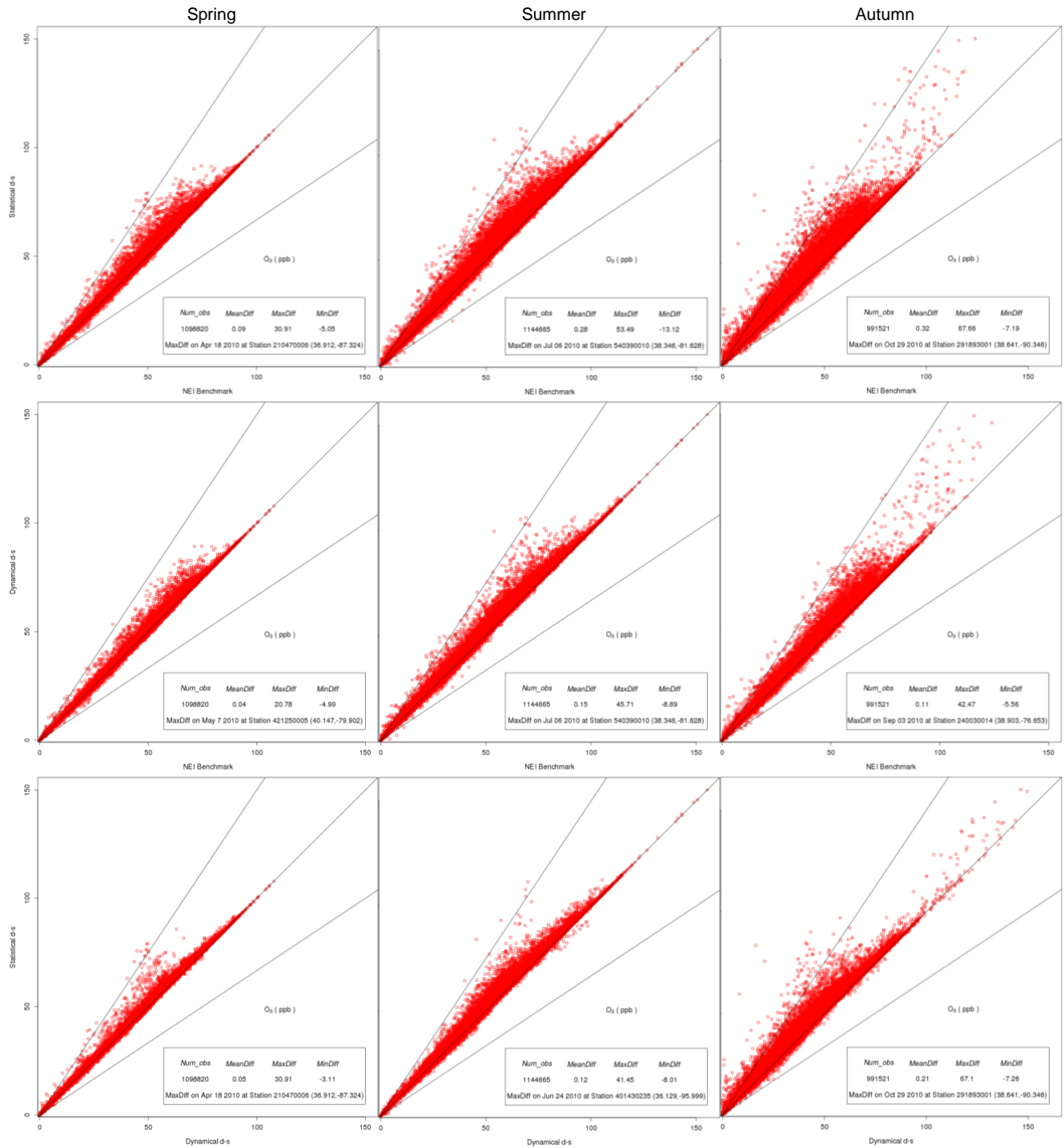
Figure 4. Seasonal comparisons of wildfire emissions methods for 1-hr O 3 (ppb) predicted at grid cells containing both Air Quality System (AQS) monitors and wildfires in 2010.
