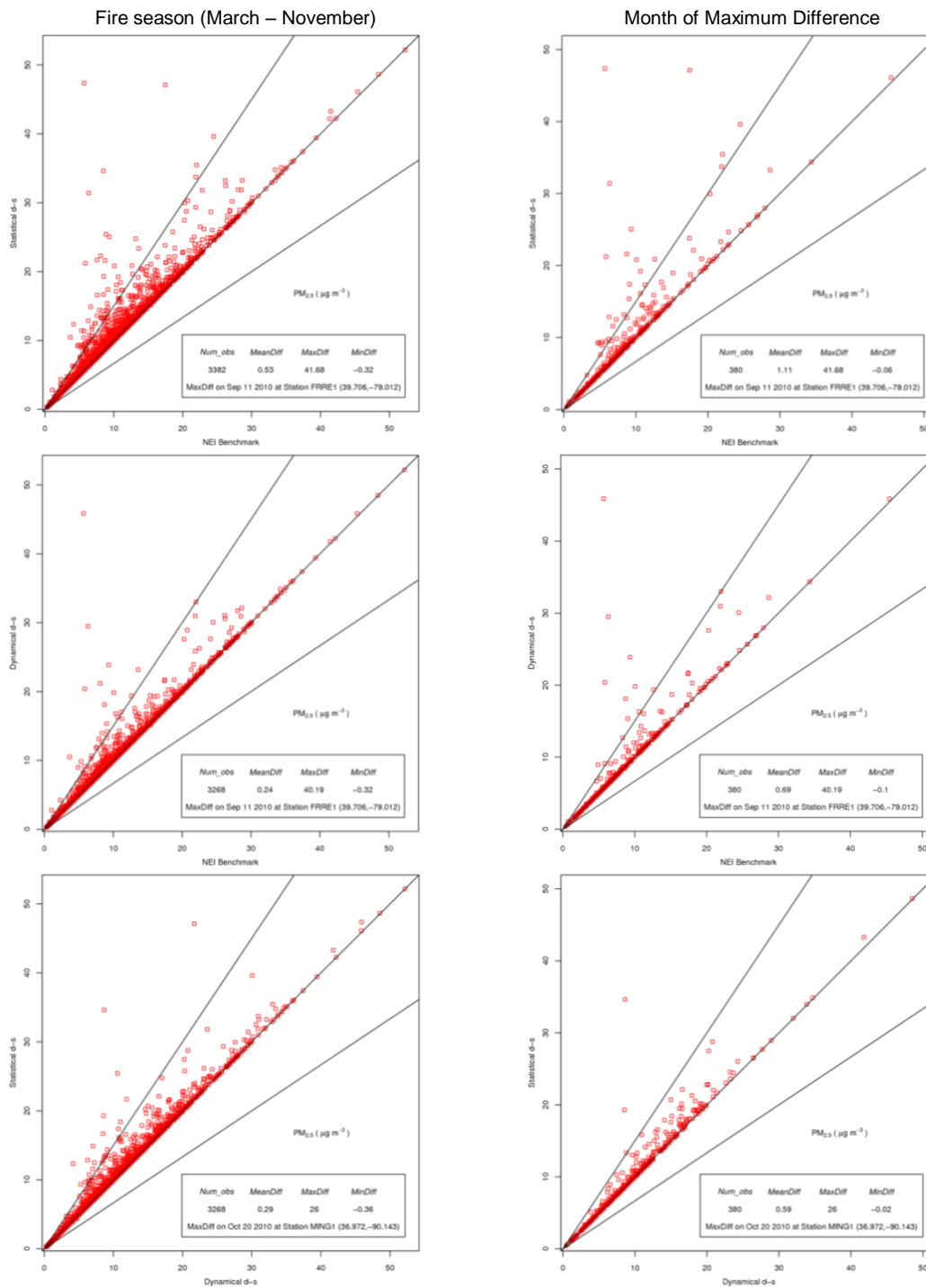
5 Figure 8. Comparisons of wildfire emissions methods for PM 2.5 (μg m -3 ) predicted at grid cells containing both Interagency Monitoring of PROtected Visual Environments (IMPROVE) monitors and wildfires in 2010. Right: top and middle – September; bottom – October.
