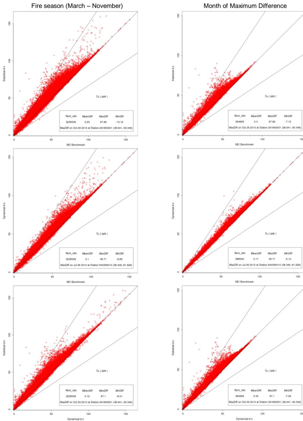
5 Figure 3. Comparisons of wildfire emissions methods for 1-hr O_3 (ppb) predicted at grid cells containing Air Quality System (AQS) monitors and wildfires in 2010. Left: fire season (March – November). Right: top and bottom – October; middle – July.
