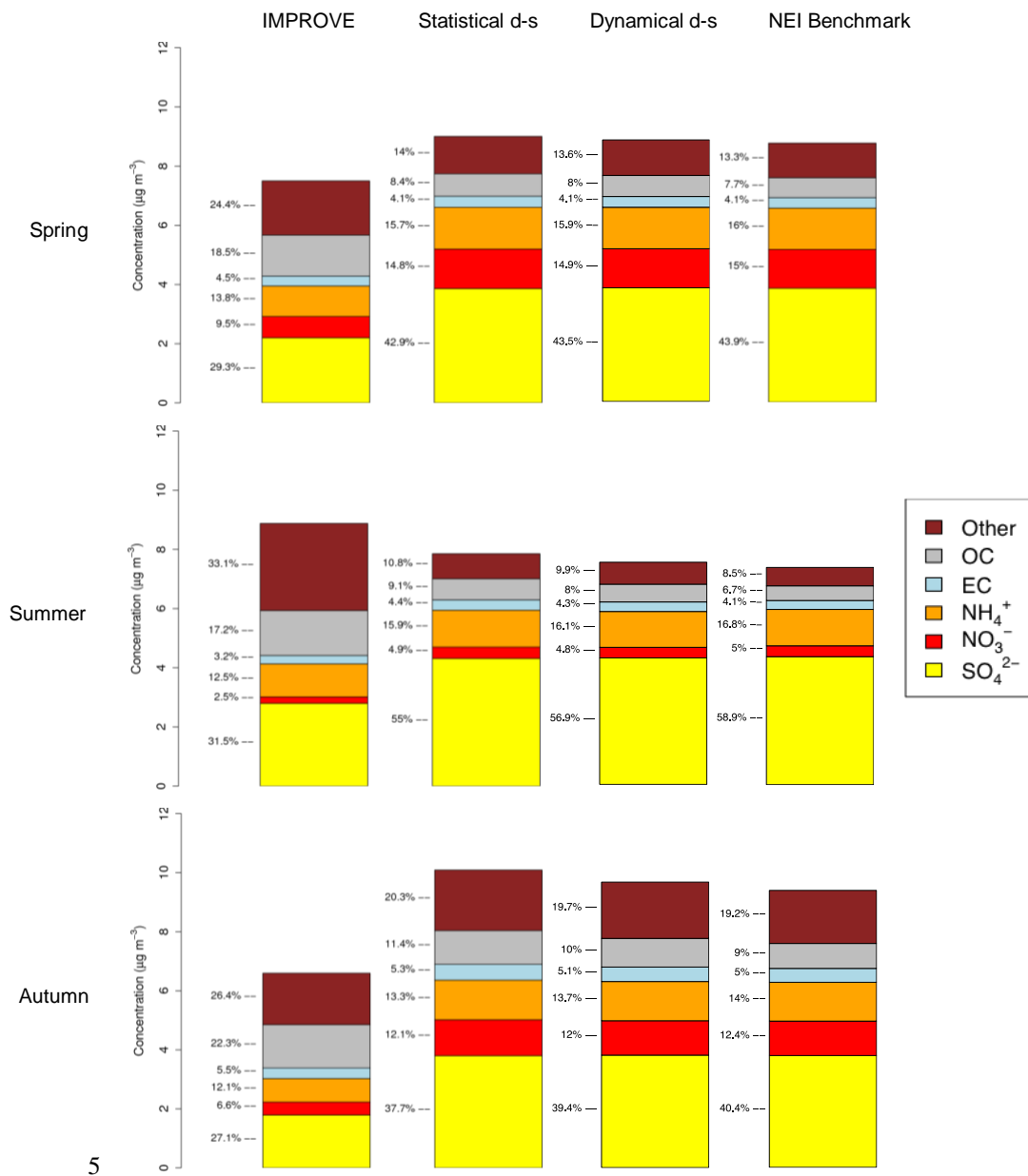
Figure 7. Domain-wide seasonally averaged total mass of PM 2.5 (µg m -3 ) and fractional mass of major constituents during the fire season compared to observations from the IMPROVE monitoring network.
