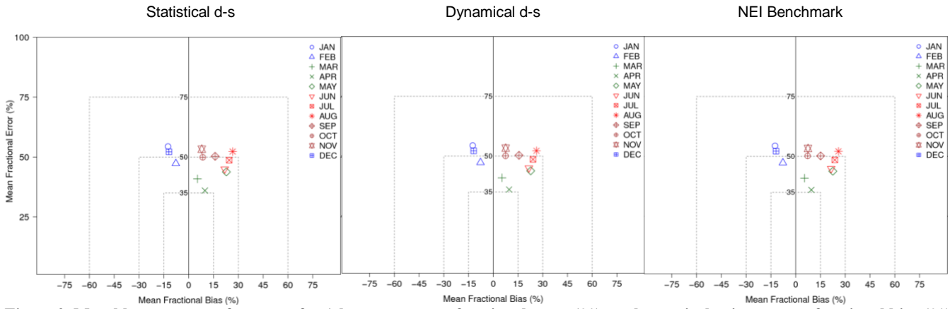
Figure 2. Monthly average performance for 1-hr ozone: mean fractional error (%) on the vertical axis vs. mean fractional bias (%) relative to observations from the Air Quality System. L – statistical d-s; C – dynamical d-s; R – NEI benchmark.
