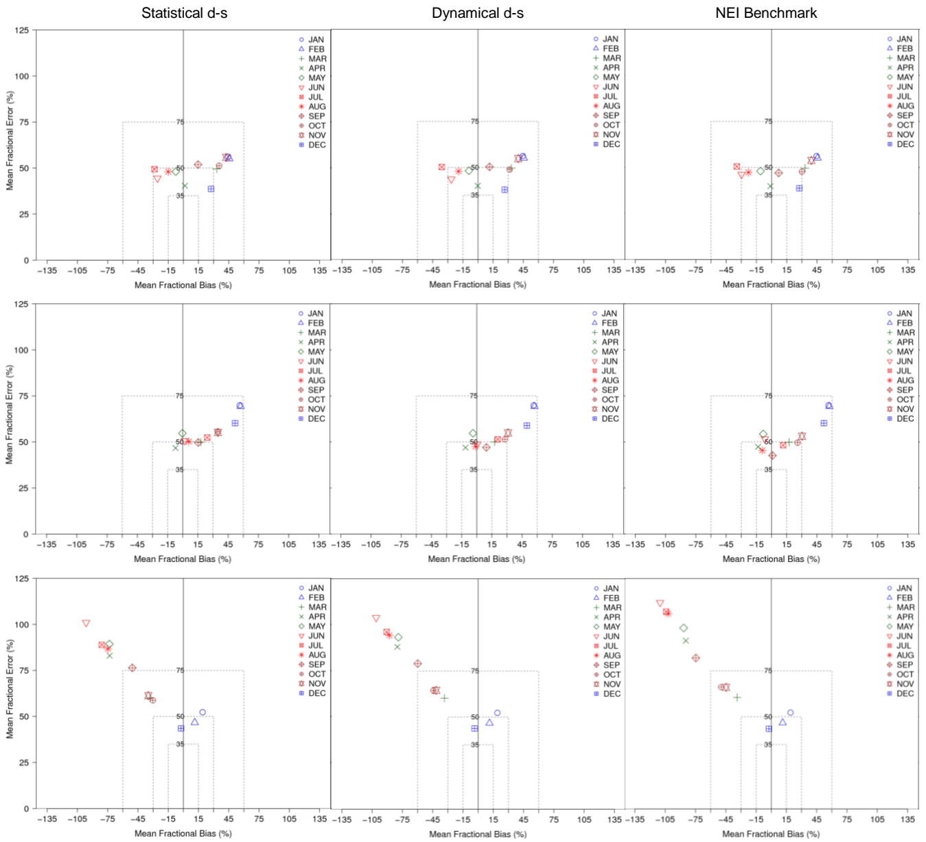
Figure 6. Monthly-averaged model performance for total PM_{2.5} and key wildfire constituents relative to observations from the IMPROVE monitoring network. Top panels – PM_{2.5} ; middle panels – elemental carbon (EC); bottom panels: organic carbon (OC).
