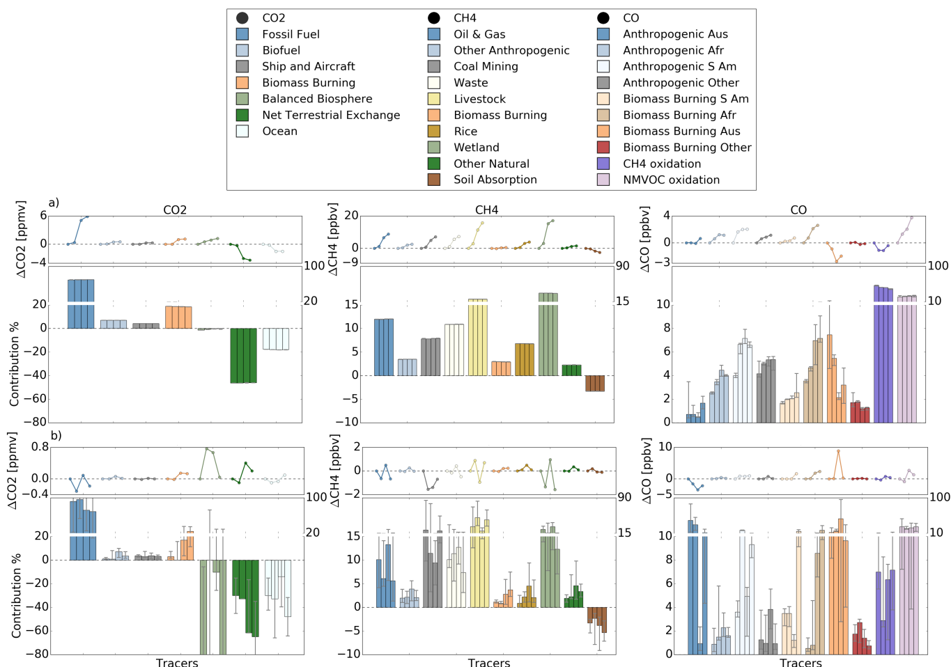
Figure 6. \text{CO}_2 , \text{CH}_4 and \text{CO} tracer contribution across the 4 measurement section in 2012 and 2013 (2012 NB, 2012 2B, 2013 NB, 2013 SB, from left to right) for the background (a) and enhancements (b). We separated out the total amount of each gas into background values and enhancements to examine the impact of different temporal and spatial scales on the change of the sources. The bottom plots show the contribution of each tracer during a specific trip while top plots show the change of each tracer across the four sections relative to the first section (2012 NB). The contributions are calculated based on the median for each section and the uncertainties represent the 25th (lower error bar) and 75th (upper error bar) percentile.
