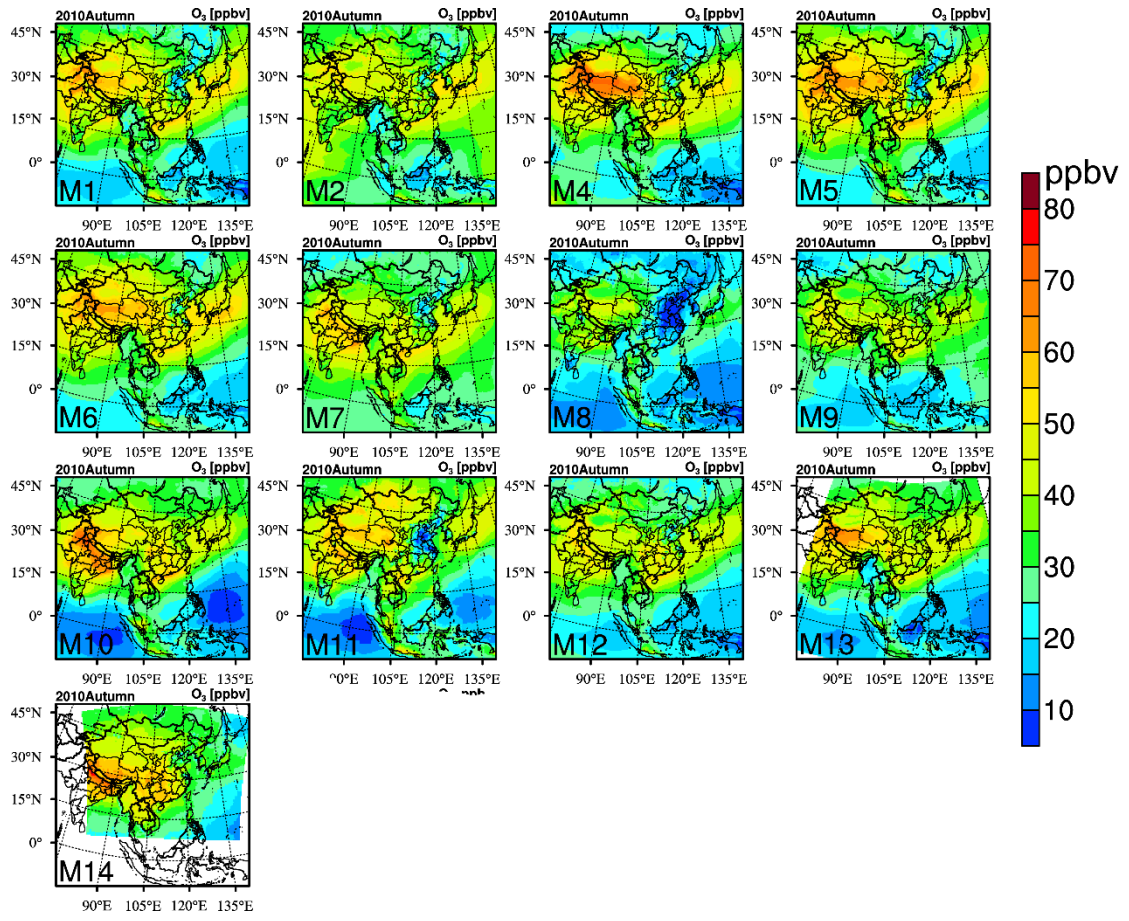
Fig.S2 Surface O 3 spatial distribution from 13 models for autumn 2010 (unit:ppbv).
