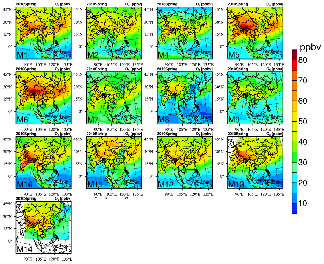
Fig.S1 Surface O 3 spatial distribution from 13 models for spring 2010 (unit:ppbv).
