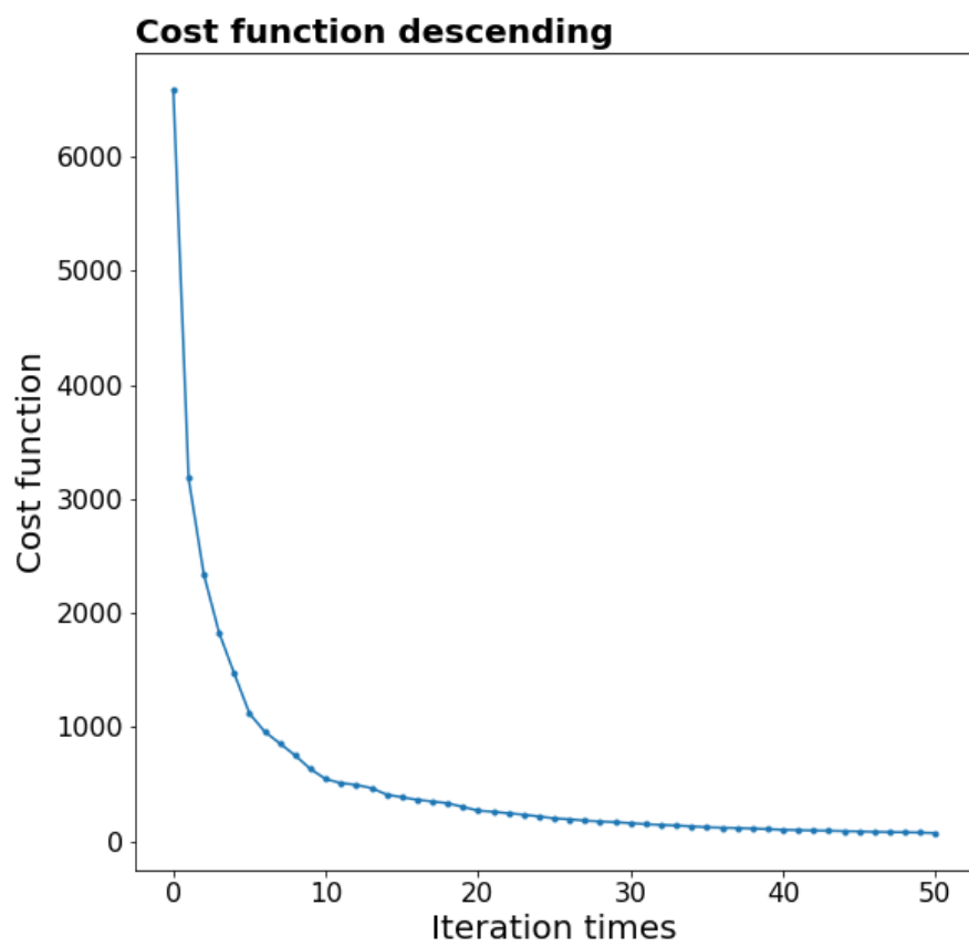
Figure 2. Cost function descending with iteration.
