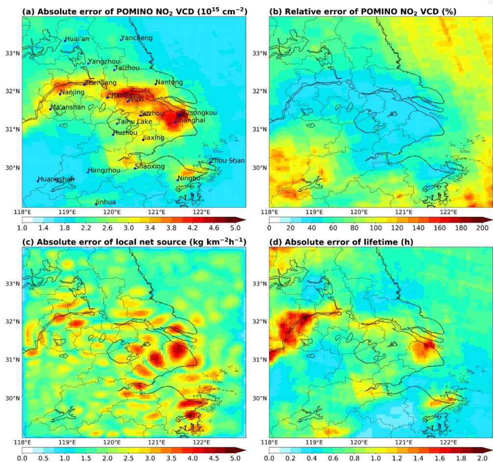
Figure 4. (a) Absolute error (1 \sigma ) of POMINO NO 2 VCD at each grid cell at the 0.05°×0.05° resolution. (b) Relative error (1 \sigma ) of POMINO NO 2 VCD. (c) Absolute error (1 \sigma ) of the derived local net source. (d) Absolute error (1 \sigma ) of the derived NO x lifetime due to chemical loss and deposition.
