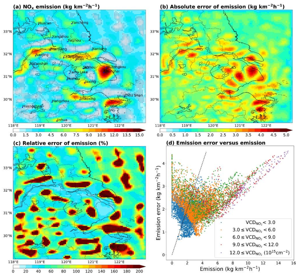
Figure 5. (a) Our \text{NO}_x emissions from anthropogenic, biomass burning and soil sources together. The blue crosses indicate where the relative errors exceed 100%. (b) Absolute errors ( 1\sigma ) of our \text{NO}_x emissions. (c) Relative errors of our emissions. (d) Absolute errors ( 1\sigma ) of \text{NO}_x emissions as a function of \text{NO}_x emissions at individual grid cells. Data points are coloured according to the magnitudes of POMINO \text{NO}_2 VCDs. The dashed line indicates an error of 100%.
