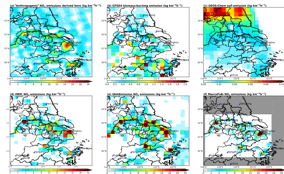
Figure 7. (a) Our “anthropogenic” \text{NO}_x emissions, by subtracting soil and biomass burning emissions from the derived emissions. (b) GFED4 biomass burning \text{NO}_x emissions. (c) Soil \text{NO}_x emissions calculated by a nested GEOS-Chem simulation. (d) MEIC \text{NO}_x emissions over summer 2012–2015. (e) DECISO v5.1qa top-down emissions in summer 2012–2015. (f) MarcoPolo bottom-up inventory in summer 2014; note that this inventory does not cover the grid cells shown in grey). All data are regridded to 0.05^\circ \times 0.05^\circ .
