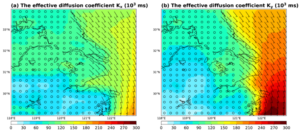
Figure A. The effective diffusion coefficients for summer 2012–2015 on a 0.05^\circ \times 0.05^\circ grid. Overlaid is the temporal mean wind vector, which is plotted for every 5 \times 5 = 25 grid cells to enhance the readability.
