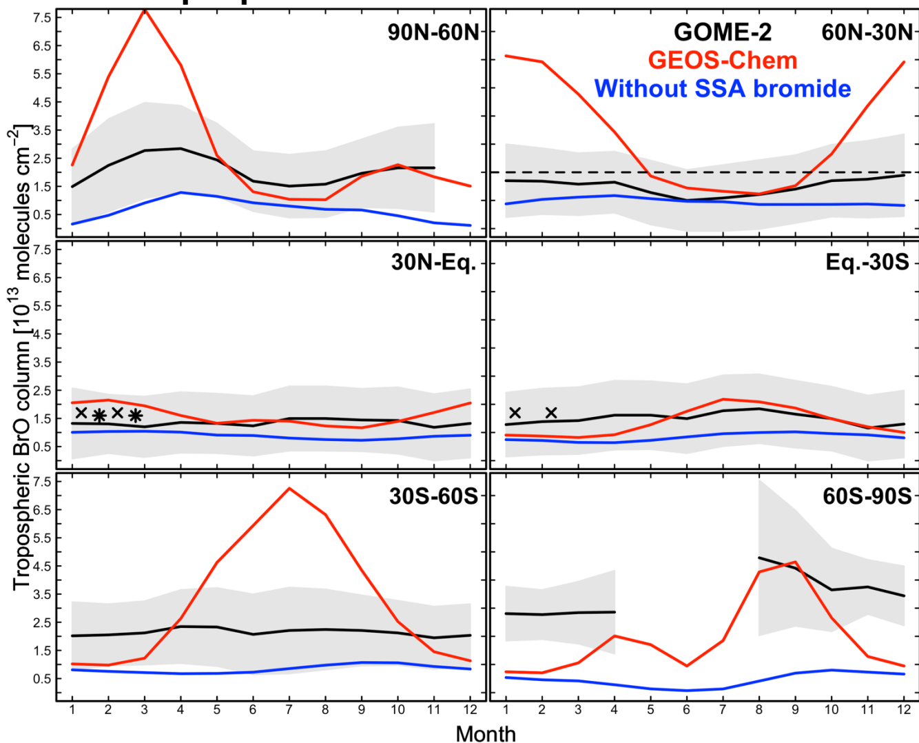
Figure 4. Seasonal variation of zonal mean tropospheric BrO columns in different latitudinal bands. Monthly GOME-2 BrO observations are for 2007 and taken from Theys et al. (2011); shading represents one standard deviation about the monthly mean GOME-2 BrO columns. GEOS-Chem BrO columns are sampled at the GOME-2 local overpass time (09:00–10:00). Red lines are from our standard simulation including sea salt aerosol (SSA) debromination, blue lines are from a sensitivity simulation without SSA debromination. The black dashed line indicates observations for 2009–2011 reported by Coburn et al. (2011) in Florida, USA without seasonality information. Black crosses and stars represent average BrO columns measured during aircraft campaigns over the eastern tropical Pacific (Volkamer et al., 2015; Wang et al., 2015; Dix et al., 2016) and western tropical Pacific (Koenig et al., 2017), respectively.
