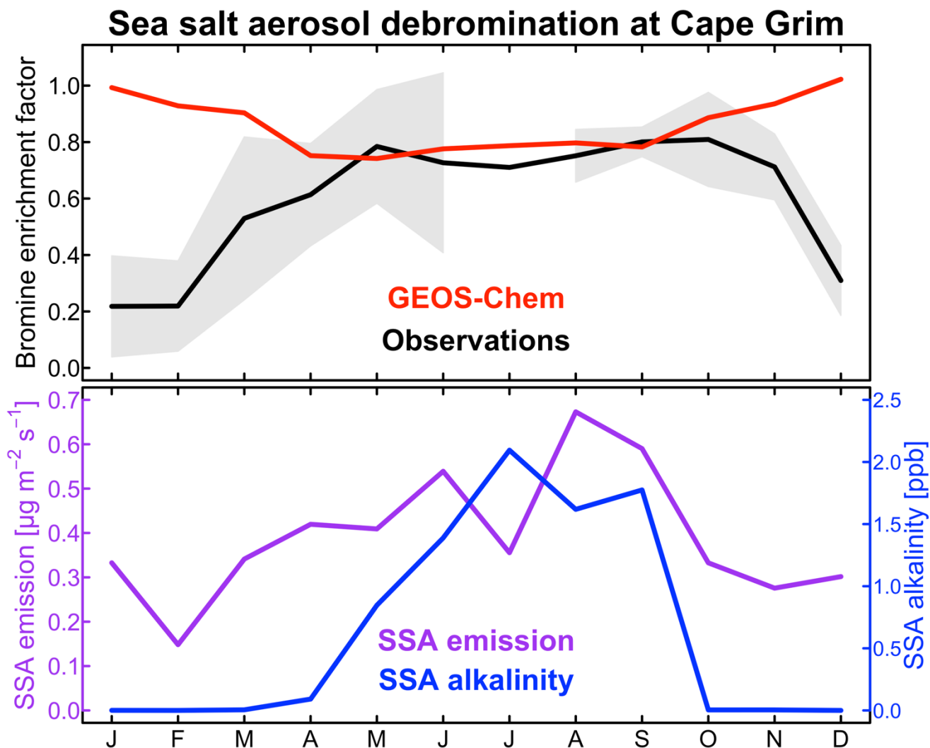
5 Figure 2. Seasonal variation of sea salt aerosol (SSA) debromination at Cape Grim, Tasmania (40.7°S, 144.7°E). The top panel shows the bromine enrichment factors ( EFs ) of monthly mean SSA in surface air. Observations from Ayers et al. (1999) and Sander et al. (2003) for 1996–1998 are compared to GEOS-Chem model values for 2012. Shading gives the interannual standard deviation in the observations. The bottom panel shows the GEOS-Chem monthly SSA emission flux at Cape Grim (Site 3 in Figure 1) and the SSA alkalinity. The SSA emission flux is for the oceanic fraction of the Cape Grim gridsquare.
