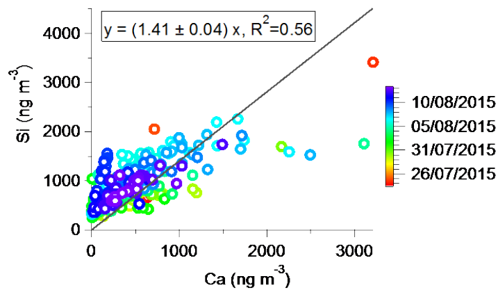
Figure S20: Scatter plot of Si vs. Ca.
