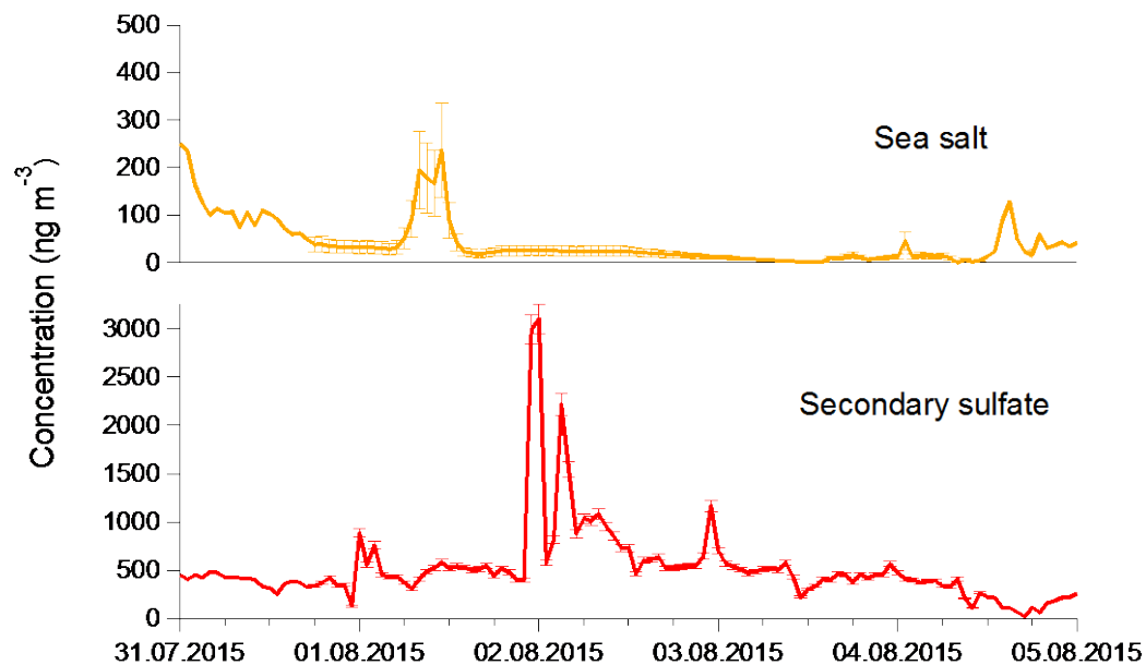
Figure S12: The factor time series of the sea salt and the secondary sulfate factors during the fireworks period (31.07.2015-04.08.2015). The estimated uncertainties of the sea salt ( \pm 42\% ) and the secondary sulfate ( \pm 5\% ) factors during the fireworks period are added as error bars (standard deviation).
