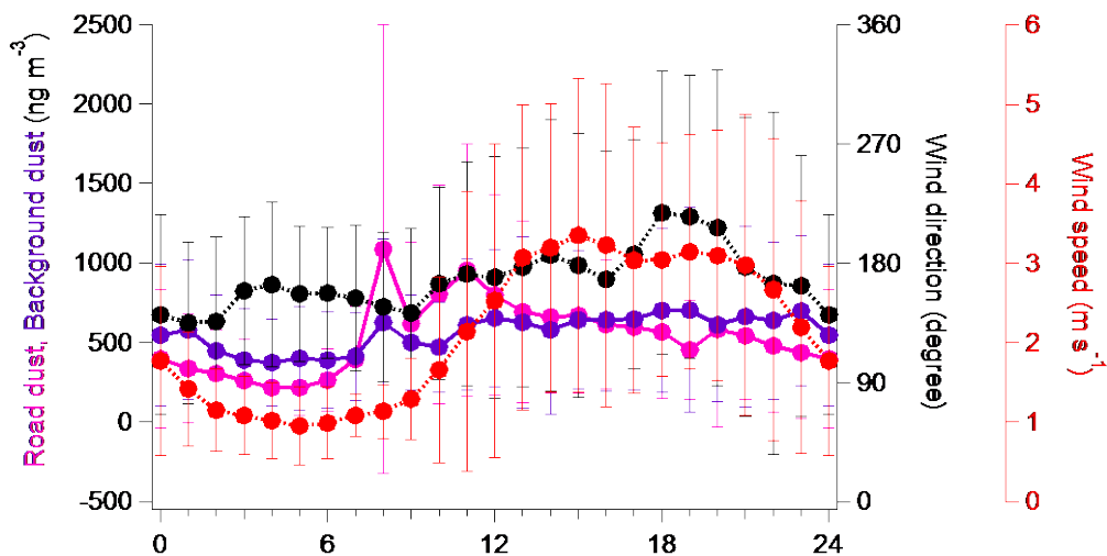
Figure S21: Mean diurnal variations of the two dust factors (left-y axis) along with wind speed and wind direction (right y-axes) with error bars (one standard deviation).
