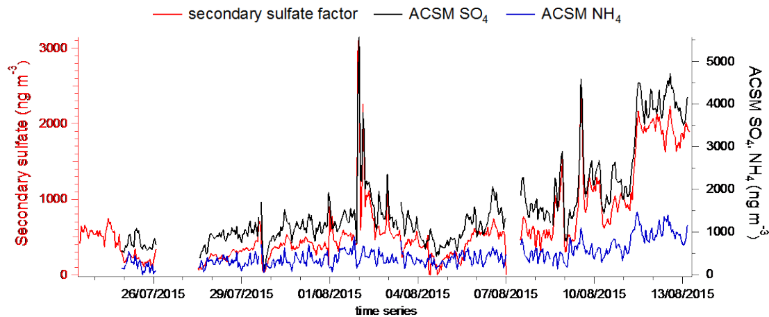
Figure S22: Time series of the secondary sulfate factor (left y-axis) and mass concentration of \text{SO}_4 , \text{NH}_4 from the ACSM (right y-axis).
