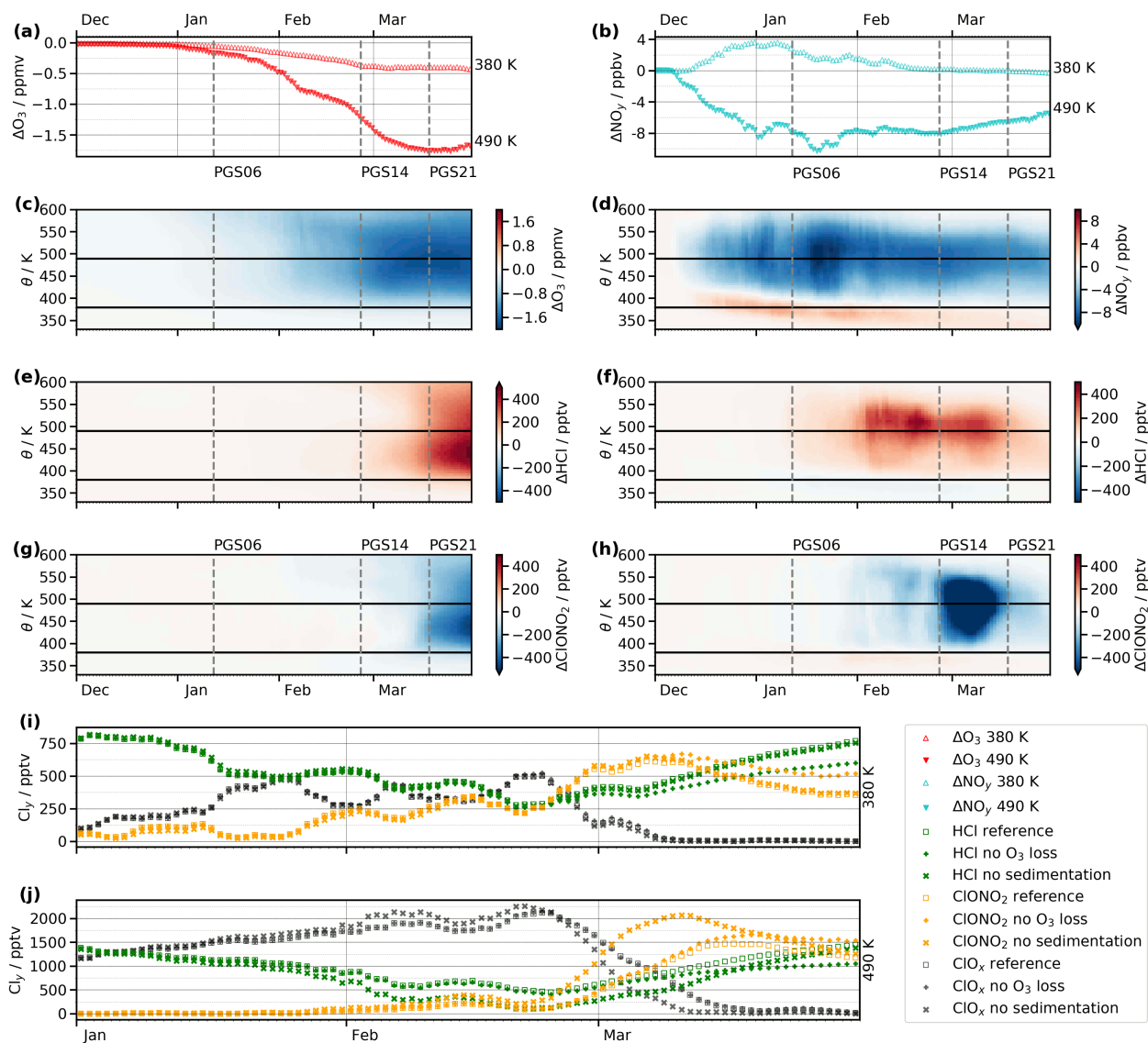
Figure 10. CLaMS vortex average (equivalent latitude > 75^\circ N ) time series for ozone loss at 380 K and 490 K (a), and as cross section (c). Denitrification is presented in the same manner (b,d). Differences in HCl and ClONO 2 between a reference simulation and a simulation without the influence of ozone depletion (e,g) or PSC sedimentation (f,h). Altitudes of 380 K and 490 K, which are illustrated in other panels, are marked with horizontal lines. The bottom panels show ClO x (black), HCl (green), and ClONO 2 (orange) for the reference simulation (open squares), and for the sensitivity simulations without ozone depletion (+) and without PSC sedimentation (x) at 380 K (i) and 490 K (j). Please note that these time series, in contrast to others in this figure, start in January.
