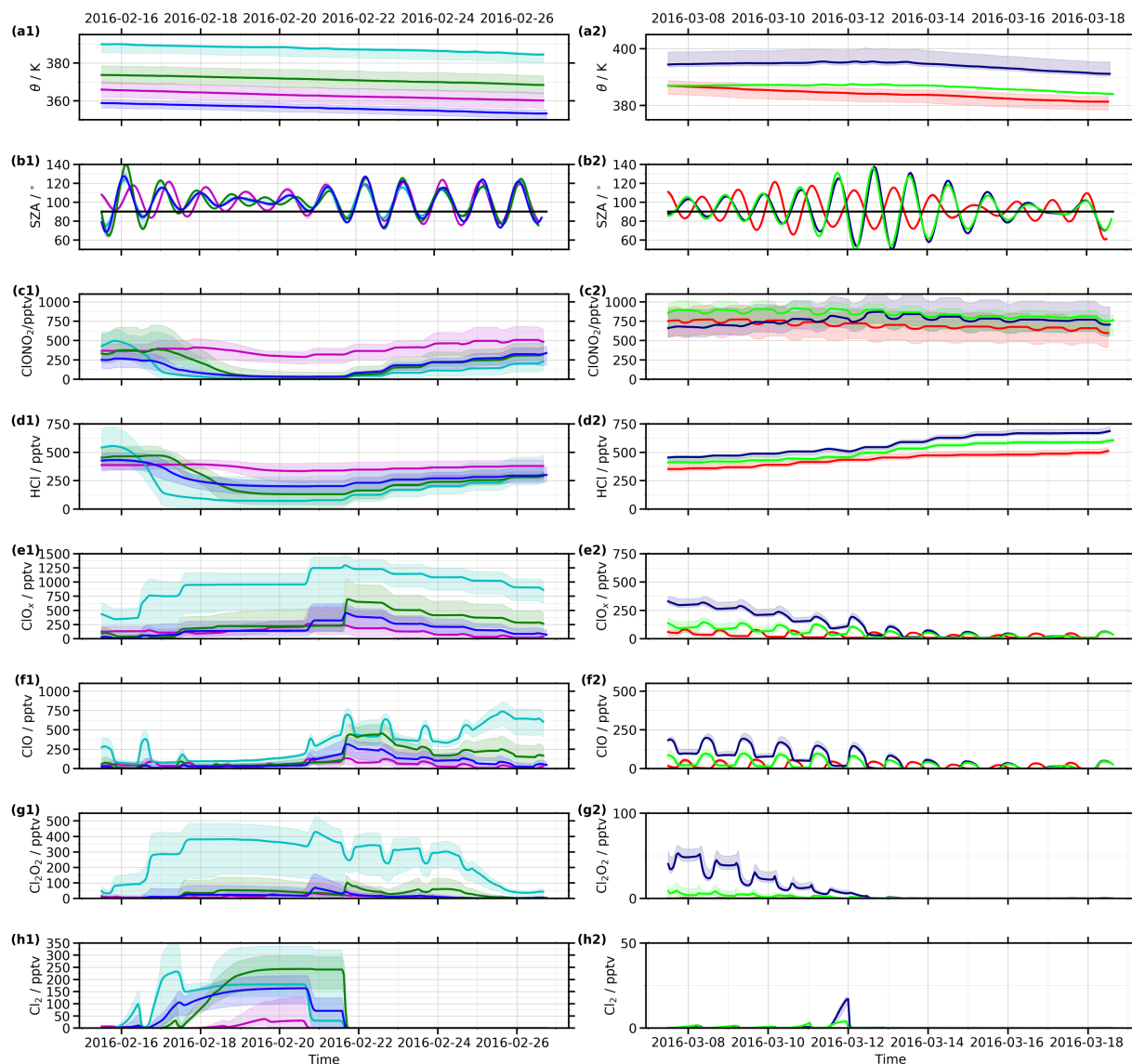
Figure 12. Modeled temporal evolution of (a) potential temperature, (b) solar zenith angle (SZ A, the 90^\circ threshold is marked with a black line), (c) \text{ClONO}_2 , (d) \text{HCl} , (e) \text{ClO}_x , (f) \text{ClO} , (g) \text{Cl}_2\text{O}_2 , and (h) \text{Cl}_2 for (1) flight PGS14 (left) and (2) flight PGS21 (right). These trajectories are color-coded as defined in Fig. 11 a-c and e-g. Solid lines show the mean of all trajectories connected with these regions and the light colors show minimum/maximum values among those trajectories. Please note different ordinate scales in each column.
