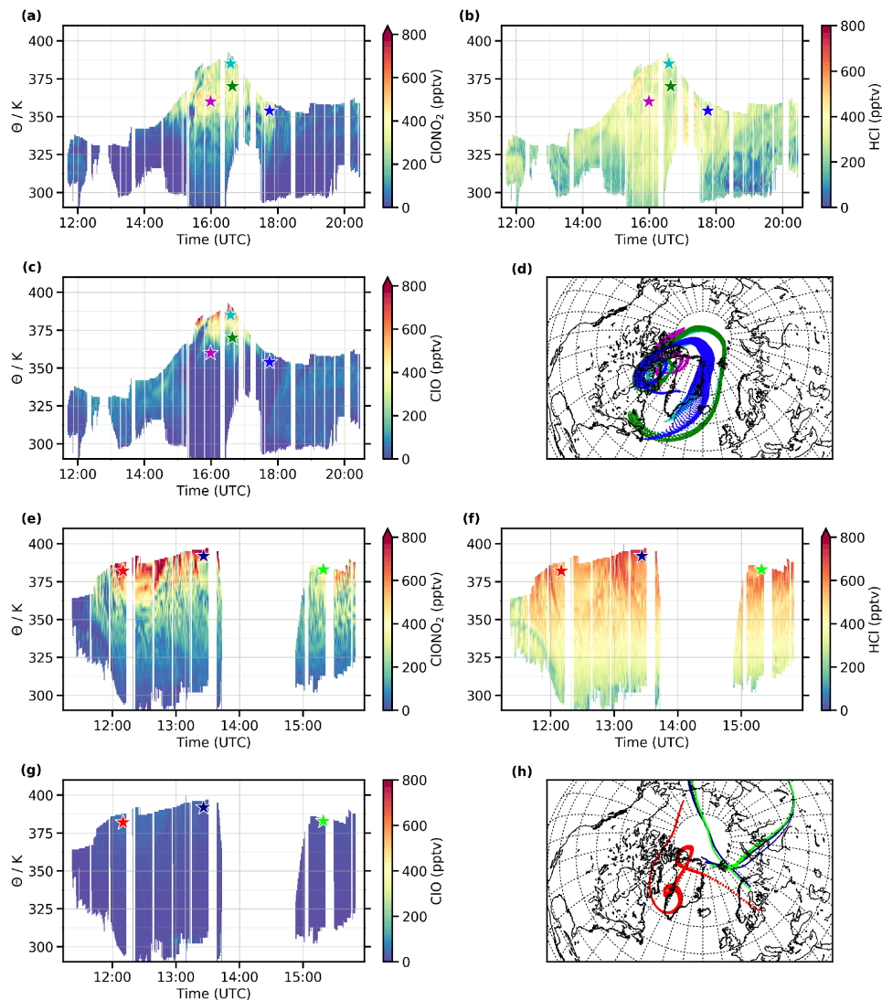
Figure 11. Cross sections for (a,e) ClONO 2 , (b,f) HCl and (c,g) ClO at the end of CLaMS trajectories leading to the GLORIA tangent point geolocations for flights PGS14 (a-d) and PGS21 (e-h). Regions of interest are marked with colored star symbols. 11-day backward trajectories calculated for each flight by CLaMS are shown on the map (d,h) in corresponding colors. The underlain map (bold black lines show coastal lines, dotted lines indicate a latitude/longitude grid) shows the northern polar region and is centered at 80°N latitude / 20°W longitude.
