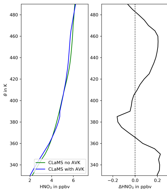
Fig. 1. Left: Exemplary vortex mean profiles (HNO 3 on 26 February 2016) from CLaMS with (blue) and without (green) the application of the MLS averaging kernel. Right: Difference of profiles with & without AVK
