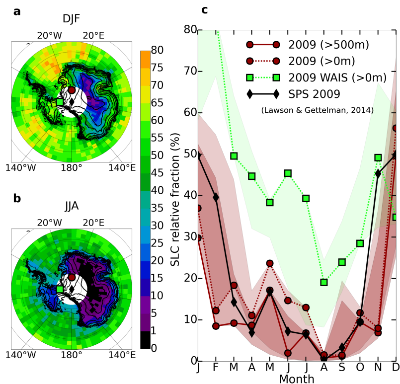
Figure 13. Left column: Geographical distribution of the 2007-2010 average of the SLC relative fraction in DJF (a) and JJA (b). The diamond marker indicates the Amundsen-Scott South Pole Station (SPS). The circle and square markers indicate the approximate locations of the gridboxes - north of the markers - used to extract the time-series in area 1 (circle) and area 2 (square), respectively (see text for exact definition of area 1 and 2). Right column: (c) Monthly time-series of the DARDAR SLC relative fraction in 2009 with (red solid line) and without (red dotted line) the lower altitude cut-off of 500m, extracted north of the circle marker shown in (a) and (b). The green dotted line shows the time-series extracted north of the square marker shown in (a) and (b). The shaded areas represent the corresponding interannual variabilities. The black diamond markers show the relative fraction of mixed-phase clouds observed with the MPL at SPS (2850m asl) in 2009 (Lawson and Gettelman, 2014, extracted from their Figure 2D).
