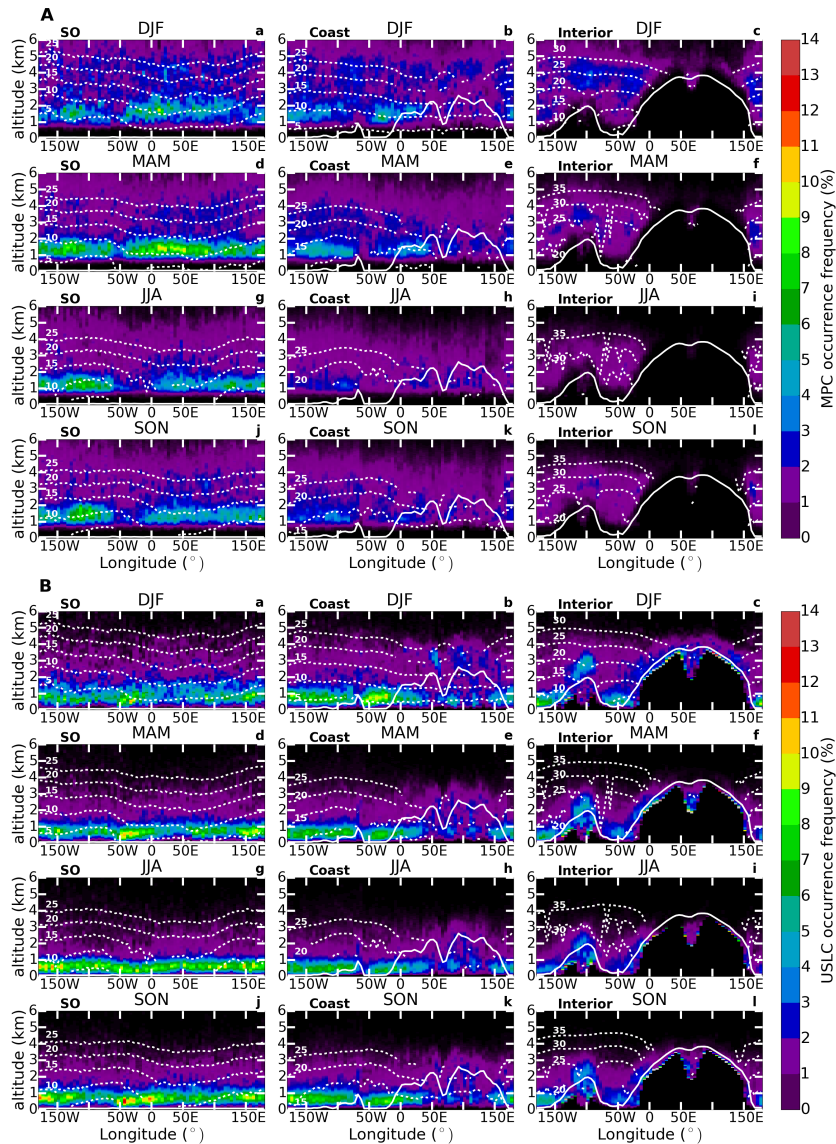
Figure 8. (A) Same as Figure 7A but for MPC fraction. (B) Same as (A) but for USLC fraction. Additionally, isotherms are shown every 5^{\circ}\text{C} (white dotted lines) and they are labelled ignoring the minus sign in the temperature value. The warmest temperature shown in all subplots is -5^{\circ}\text{C} . In plots Aa to Ak and Ba to Bk (SO and Coastal transects) isotherms are shown down to -25^{\circ}\text{C} only, while for the interior transects they are shown down to -35^{\circ}\text{C} .
