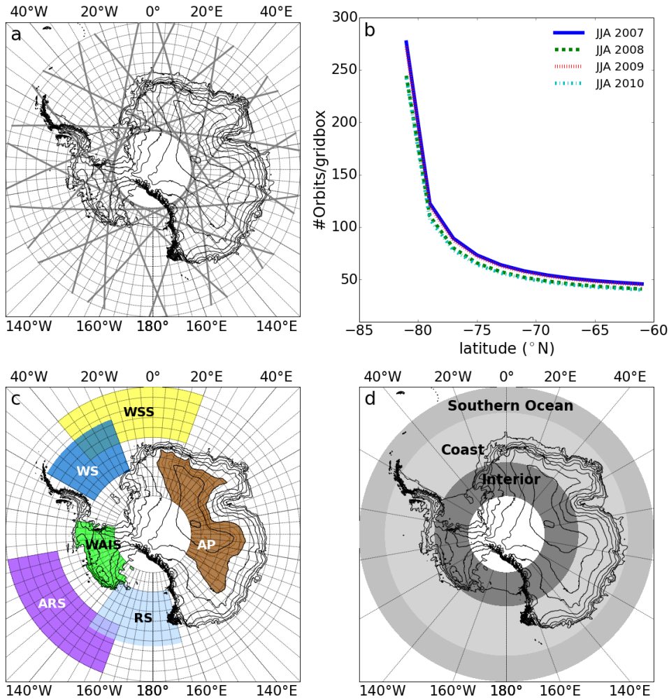
Figure 4. (a) The Cloudsat tracks across the Antarctic on the 1st of January 2007, and the grid (gridboxes of 2^\circ in latitude and 5^\circ in longitude) used to derive the geographical distribution of cloud occurrences and extending between 60^\circ S and 82^\circ S (b) The zonally averaged number of satellite overpasses per gridbox as a function of latitude, for the whole winter season each year. (c) Areas of interest used in the study, and introduced in section 4.3 for investigating the monthly evolution of cloud occurrences. They are called: WSS (in the Weddell Sea Sector), ARS (in the Amundsen-Ross sector), WS (in the Weddell Sea), RS (in the Ross Sea), the WAIS (on the West Antarctic Ice Sheet), and AP (on the Antarctic Plateau). Names are recalled in Table 1. (d) The three latitudinal bands used for the average vertical transects presented in section 4.2.
