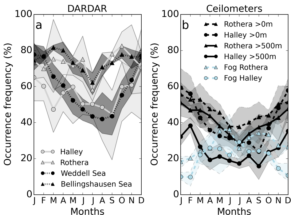
Figure 12. (a) Four-year (2007-2010) average time-series of the monthly mean low-level cloud fraction plotted for the gridbox corresponding to Rothera (triangle, solid line) and Halley station (circle, solid line), and the Bellingshausen Sea (triangle, dotted line) and the Weddell Sea (circle, dotted line). (b) Four-year (2007-2010) average time-series of the monthly mean of the cloud base detections by the ceilometers at Rothera (triangle) and Halley (circle), for detections above 0 m (dashed line) and 500 m (solid line) above surface. Light blue dashed lines show the fog detections for Rothera (triangle), and Halley (circle).
