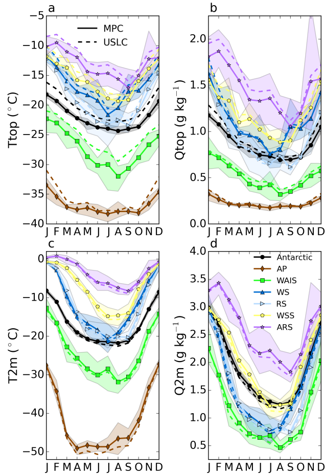
Figure 11. Top row: monthly time series of (a) the in-cloud Temperature ( T_{top} ), and of (b) the in-cloud water vapour mixing ratio ( Q_{top} ), at the top of the low-level MPC and USLC layers, for the different regions of interest. Bottom row: near-surface (two-meters) temperature (c) and water vapour mass mixing ratio (d) below these layers. The shaded areas indicate the interannual variability for the MPC layers. For readability, the ones for the USLC layers are not shown, but they are of similar amplitude.
