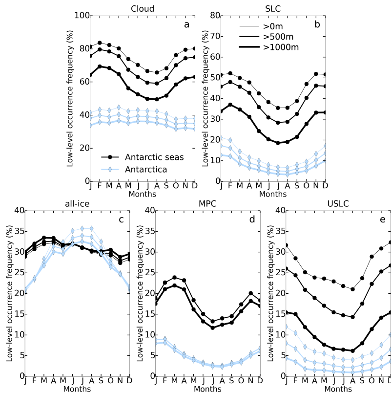
Figure B1. Monthly time series of the low-level cloud fraction (a), SLC fraction (b), all-ice fraction (c), MPC fraction (d), and USLC fraction (e), for three different lower-altitude cut-offs: 0m (thinnest solid line), 500m (intermediate), 1000m (thickest solid line). They are plotted by distinguishing between continental (blue lines) and marine (black lines) clouds. See section 3.2 for the definitions of the phases.
