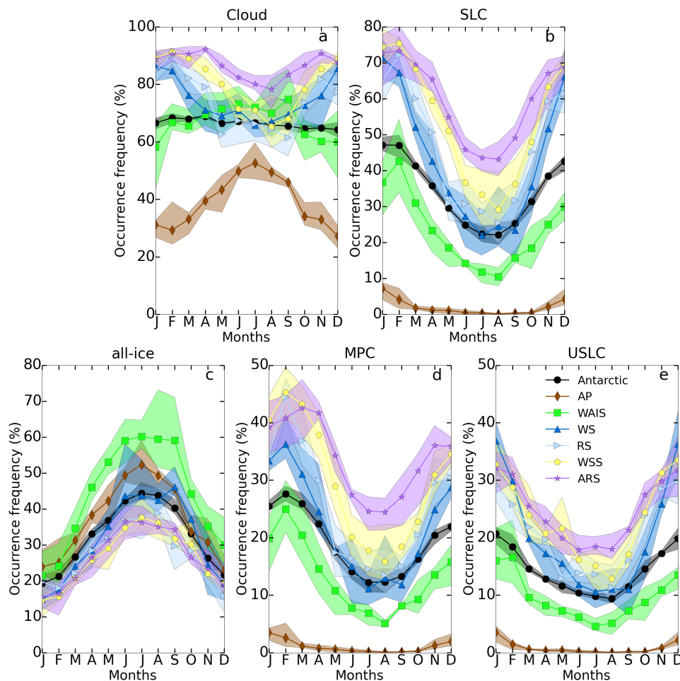
Figure 9. Four-year (2007-2010) average monthly time series of the total cloud fraction (a), SLC fraction (b), all-ice fraction (c), MPC fraction (d), and USLC fraction (e). See section 3.2 for the definition of the cloud categories. The different colours correspond to the different investigated regions (see map in Figure 4c): WSS (in the Weddell Sea sector), ARS (for the Amundsen-Ross sector), WS (in the Weddell Sea), RS (in the Ross Sea), the WAIS (on the West Antarctic Ice Sheet), and AP (Antarctic Plateau). The shaded areas indicate the amplitude between the monthly minimum and maximum encountered over the years from 2007 to 2010.
