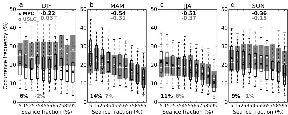
Figure 15. Same as Figure 14 for the low-level MPC (narrow empty black boxes, with a cross showing the average) and USLC (larger shaded grey boxes, with a white circle for the average) fractions. The p-values for the correlation coefficients are always <0.01, except for the USLC fraction in summer (p-value=0.06).
