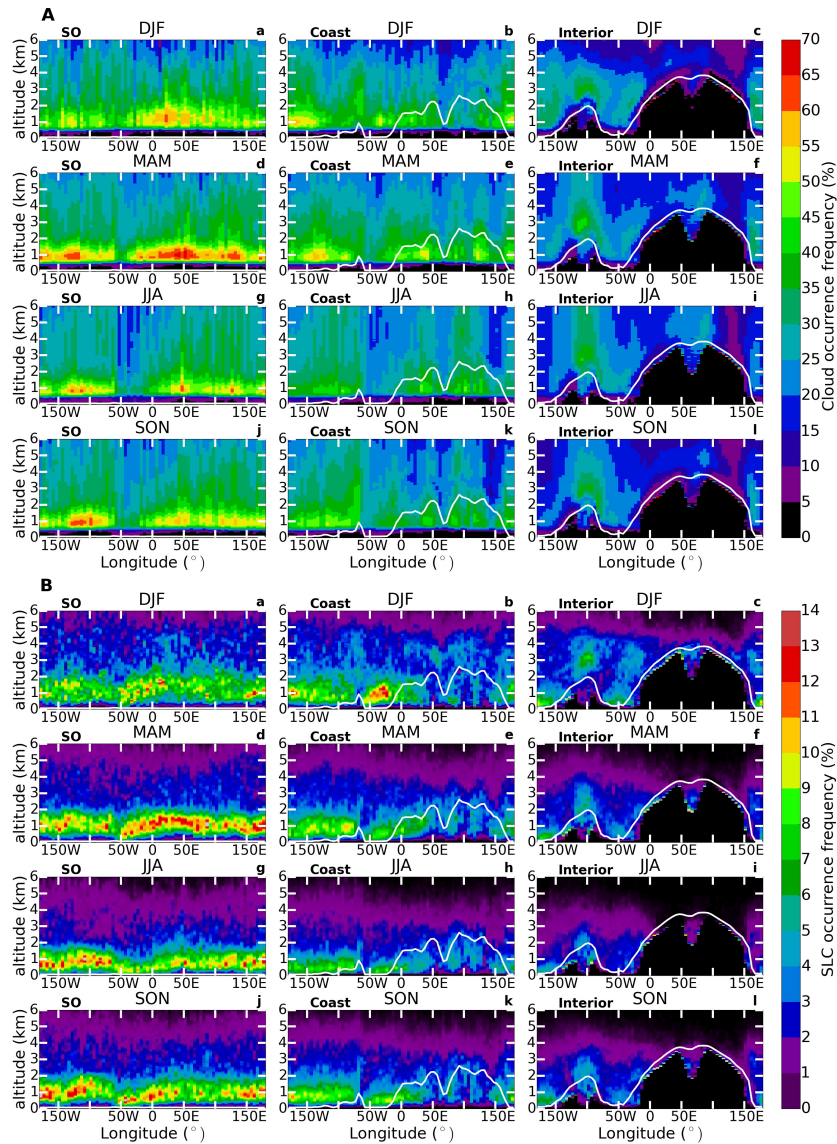
Figure 7. (A) Four-year (2007-2010) average seasonal vertical transects of the cloud fraction, spatially averaged over three latitudinal bands defined in Figure 4d (SO stands for Southern Ocean). One column corresponds to one latitudinal band, showing the four seasons. Each line corresponds to one season. (B) Same as (A) for the SLC fraction. The white line is the average surface elevation in the latitudinal band.
